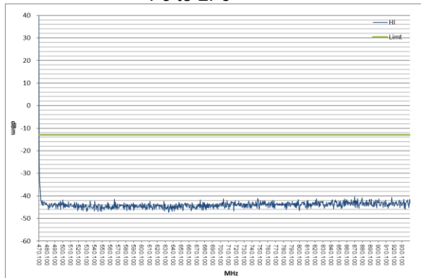
Hi Power Fc= 470.05 MHz Fc to 2Fc
