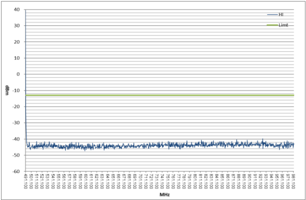
Hi Power Fc= 491.05 MHz Fc to 2Fc
