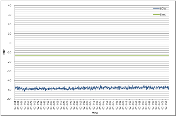
Low Power Fc= 470.05 MHz Fc to 2Fc
