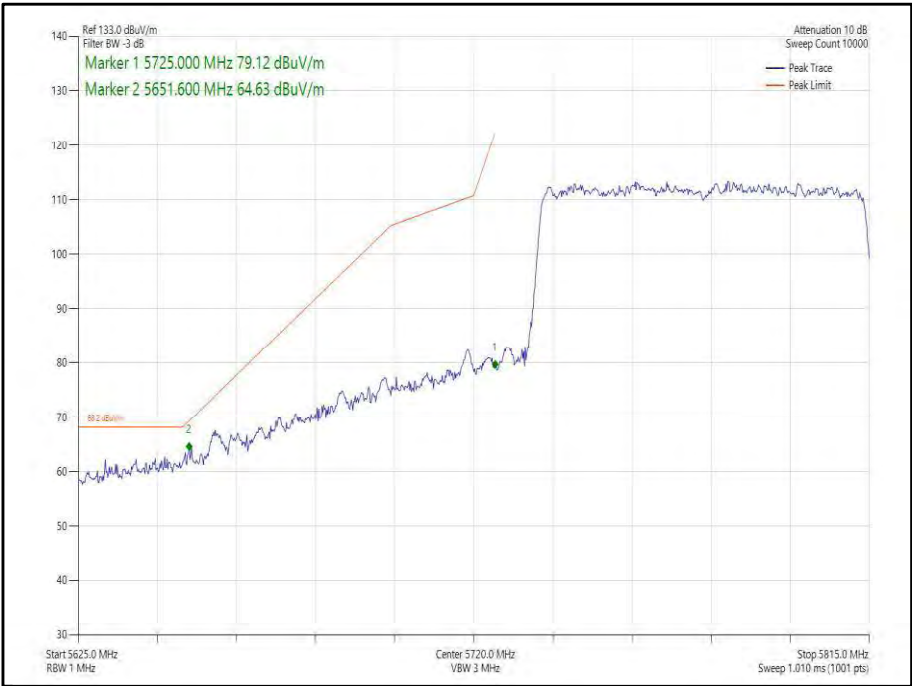
Figure 470 - 802.11ax, HE80, SU, SDM, Core 0-1 - 5775 MHz, Band Edge Frequency 5725 MHz
