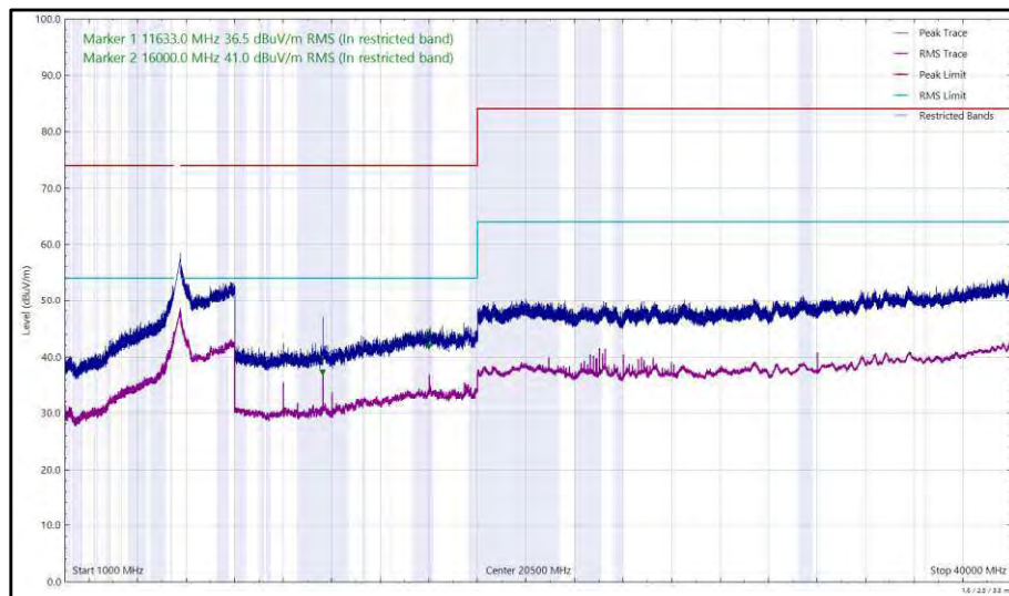
Figure 548 - U-NII-2C - 5700 MHz (CH140), 802.11a, Core 1, 1 GHz to 40 GHz, Horizontal
