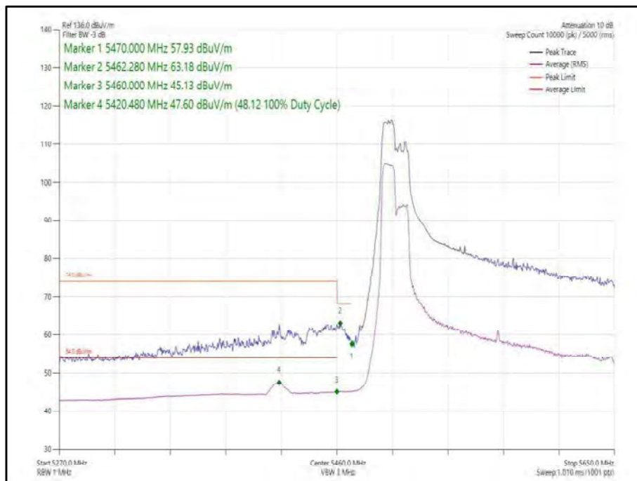
Figure 491 - 802.11ax, HE160, RU 106-53 SISO, Core 0 - 5570 MHz, Band Edge Frequency 5470 MHz
