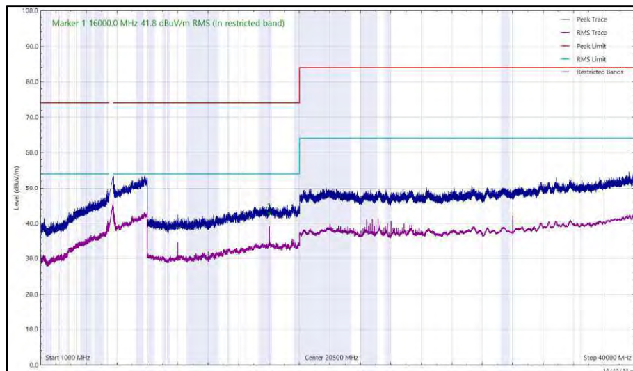
Figure 547 - U-NII-2C - 5700 MHz (CH140), 802.11a, Core 0, 1 GHz to 40 GHz, Vertical
