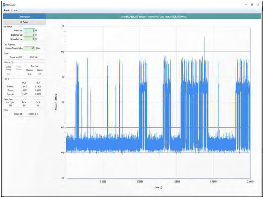
Figure 586 - Channel Loading
