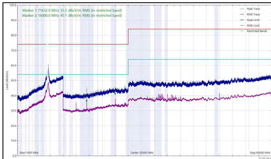
Figure 546 - U-NII-2C - 5700 MHz (CH140), 802.11a, Core 0, 1 GHz to 40 GHz, Horizontal
