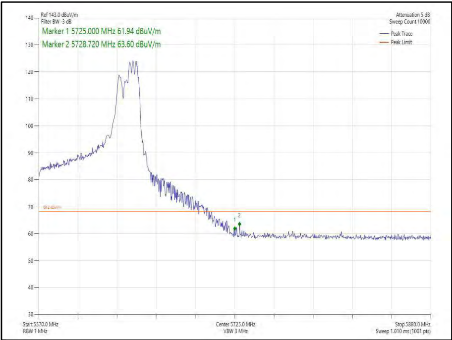
Figure 474 - 802.11ax, HE80, RU 106-60, SDM, Core 0-1 - 5610 MHz, Band Edge Frequency 5725 MHz
