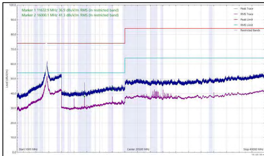
Figure 550 - U-NII-2C - 5700 MHz (CH140), VHT20, CDD, Core 0 + Core 1, 1 GHz to 40 GHz, Horizontal
