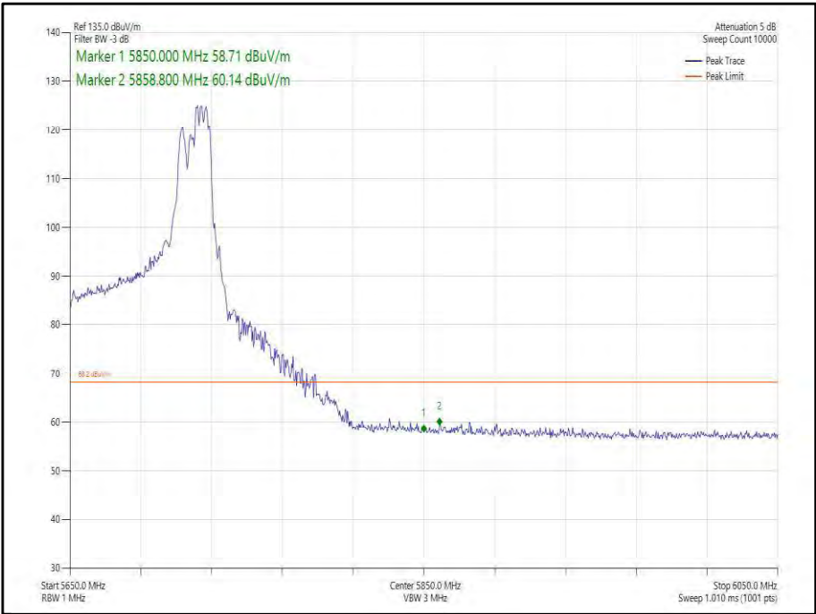
Figure 463 - 802.11ax, HE80, RU 106-60, CDD, Core 0-1 - 5690 MHz, Band Edge Frequency 5850 MHz
