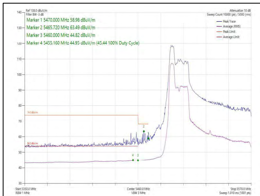
Figure 438 - 802.11ax, HE80, RU 52-37, SISO, Core 1 - 5530 MHz, Band Edge Frequency 5470 MHz
