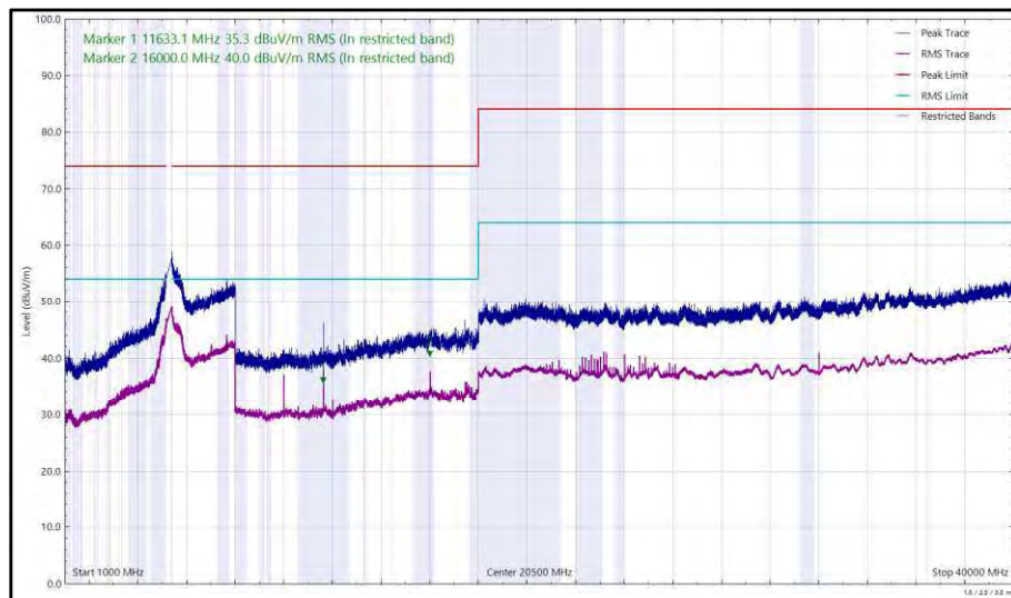
Figure 536 - U-NII-2A - 5320 MHz (CH64), VHT20, CDD, Core 0 + Core 1, 1 GHz to 40 GHz, Horizontal
