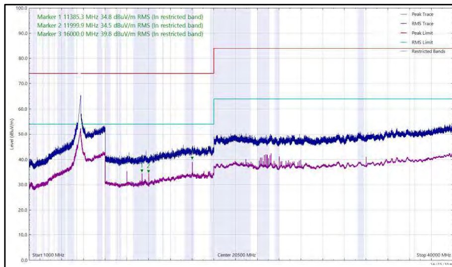
Figure 552 - U-NII-2C - 5700 MHz (CH140), HE20, RU52-37, CDD, Core 0 + Core 1, 1 GHz to 40 GHz, Horizontal
