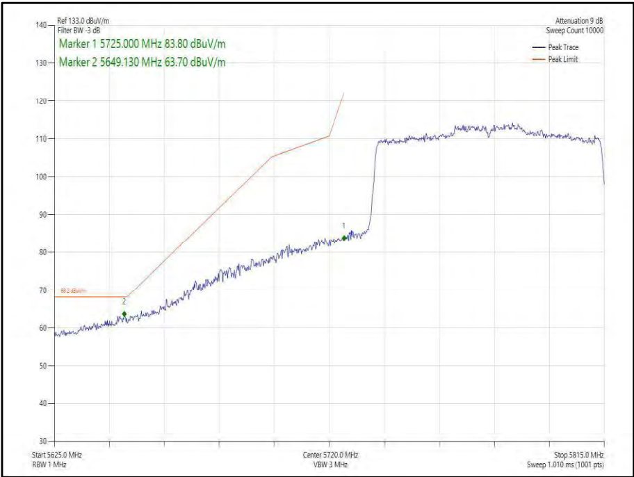
Figure 440 - 802.11ax, HE80, SU, SISO, Core 1 - 5775 MHz, Band Edge Frequency 5725 MHz
