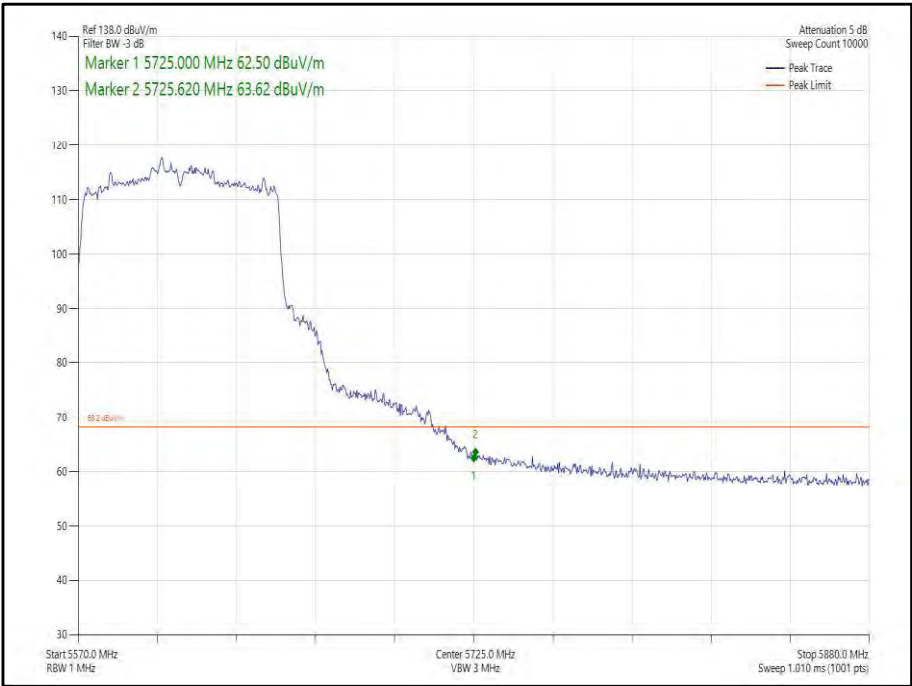
Figure 472 - 802.11ac, VHT80, SDM, Core 0-1 - 5610 MHz, Band Edge Frequency 5725 MHz
