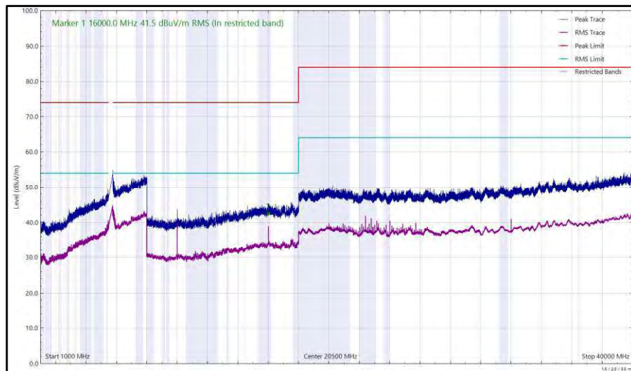
Figure 549 - U-NII-2C - 5700 MHz (CH140), 802.11a, Core 1, 1 GHz to 40 GHz, Vertical
