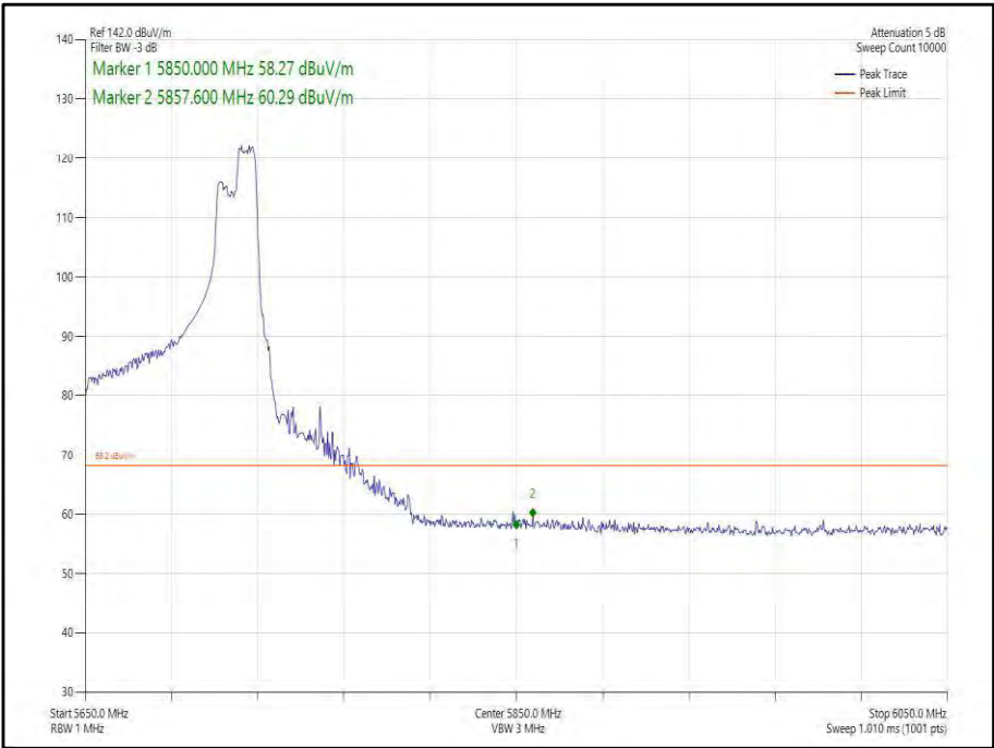
Figure 448 - 802.11ax, HE80, RU 106-60, SISO, Core 1 - 5690 MHz, Band Edge Frequency 5850 MHz
