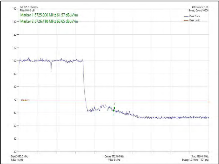
Figure 499 - 802.11ax, HE160, SU, SISO, Core 1 - 5570 MHz, Band Edge Frequency 5725 MHz
