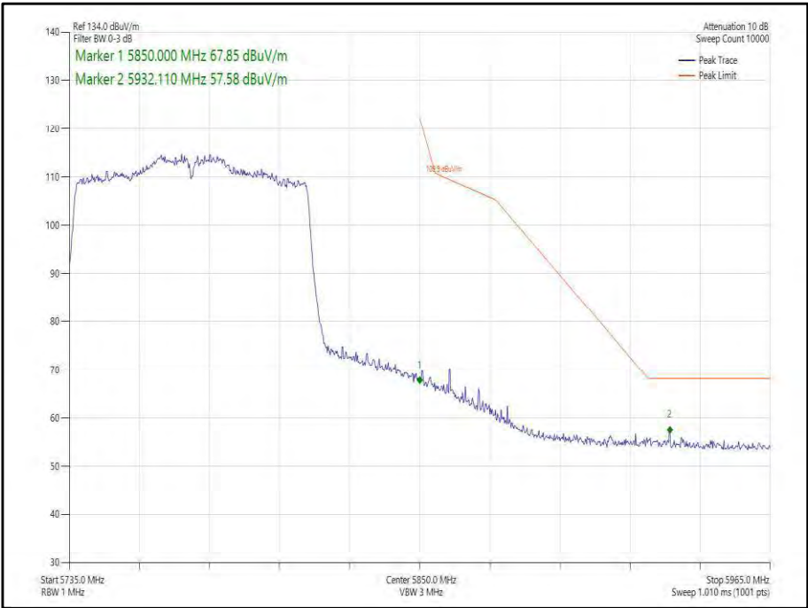
Figure 487 - 802.11ac, VHT80, TxBF, Core 0-1 - 5775 MHz, Band Edge Frequency 5850 MHz
