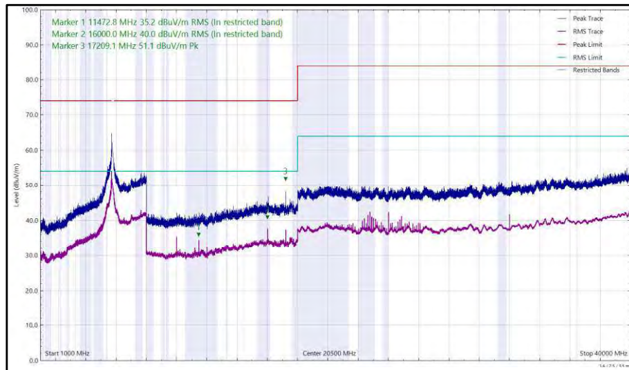
Figure 560 - U-NII-3 - 5745 MHz (CH149), HE20, RU26-0, CDD, Core 0 + Core 1, 1 GHz to 40 GHz, Horizontal
