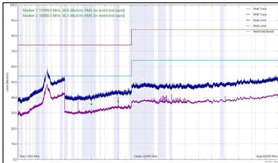
Figure 534 - U-NII-2A - 5320 MHz (CH64), HE20, RU52-37, CDD, Core 0 + Core 1, 1 GHz to 40 GHz, Horizontal
