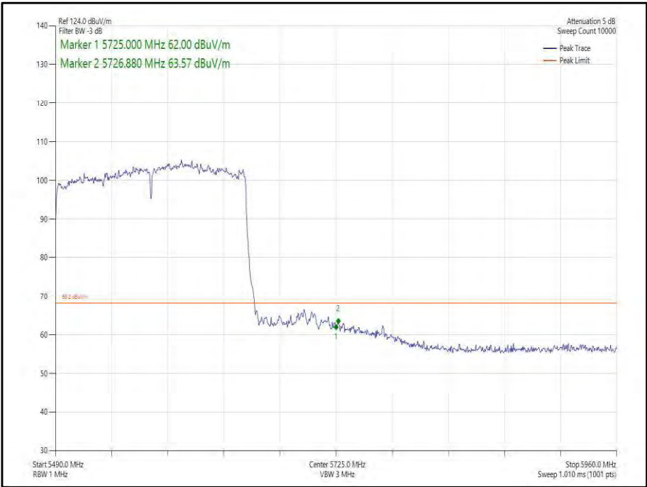
Figure 493 - 802.11ax, HE160, SU, SISO, Core 0 - 5570 MHz, Band Edge Frequency 5725 MHz
