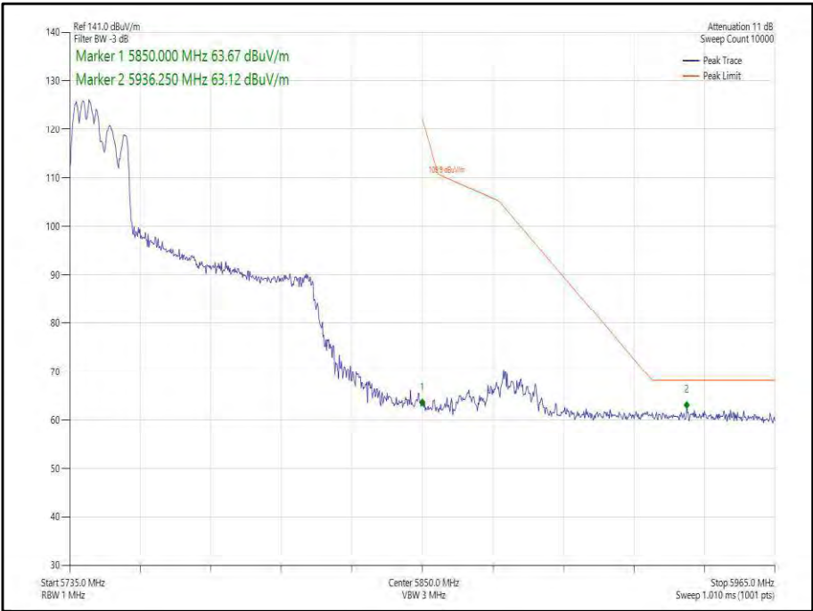
Figure 480 - 802.11ax, HE80, RU 106-53, SDM, Core 0-1 - 5775 MHz, Band Edge Frequency 5850 MHz
