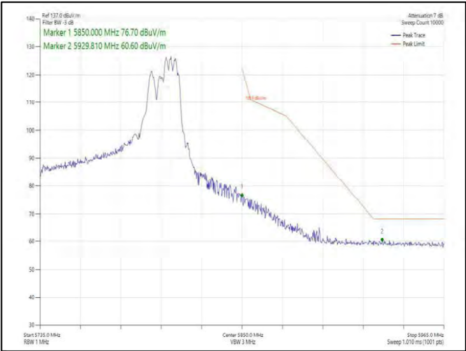
Figure 465 - 802.11ax, HE80, RU 106-60, CDD, Core 0-1 - 5775 MHz, Band Edge Frequency 5850 MHz
