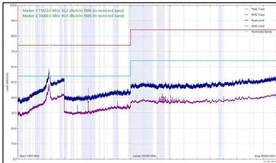
Figure 554 - U-NII-3 - 5745 MHz (CH149), 802.11a, Core 0, 1 GHz to 40 GHz, Horizontal
