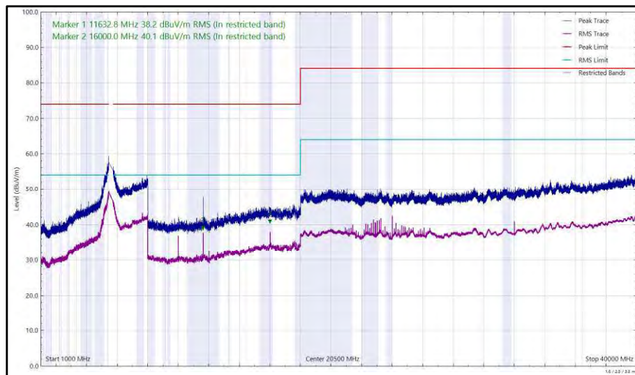
Figure 542 - U-NII-2C - 5500 MHz (CH100), VHT20, CDD, Core 0 + Core 1, 1 GHz to 40 GHz, Horizontal
