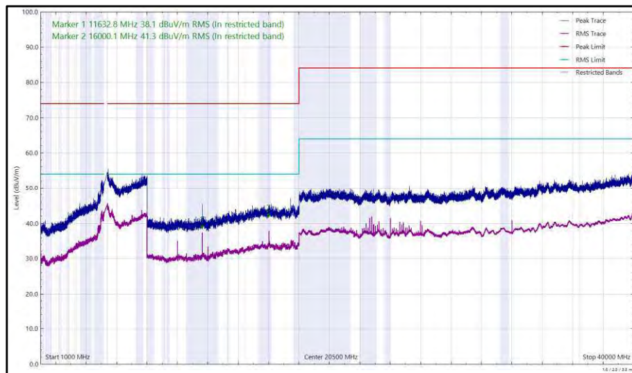
Figure 532 - U-NII-2A - 5320 MHz (CH64), 802.11a, Core 1, 1 GHz to 40 GHz, Horizontal
