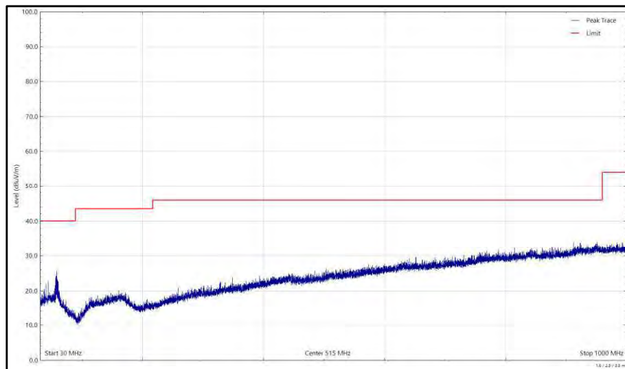
Figure 566 - U-NII-3 - 5825 MHz (CH165), 802.11a, Core 1, 30 MHz to 1 GHz, Horizontal (Peak)
