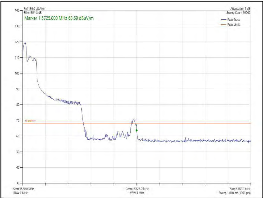
Figure 444 - 802.11ax, HE80, RU 52-37, SISO, Core 1 - 5610 MHz, Band Edge Frequency 5725 MHz
