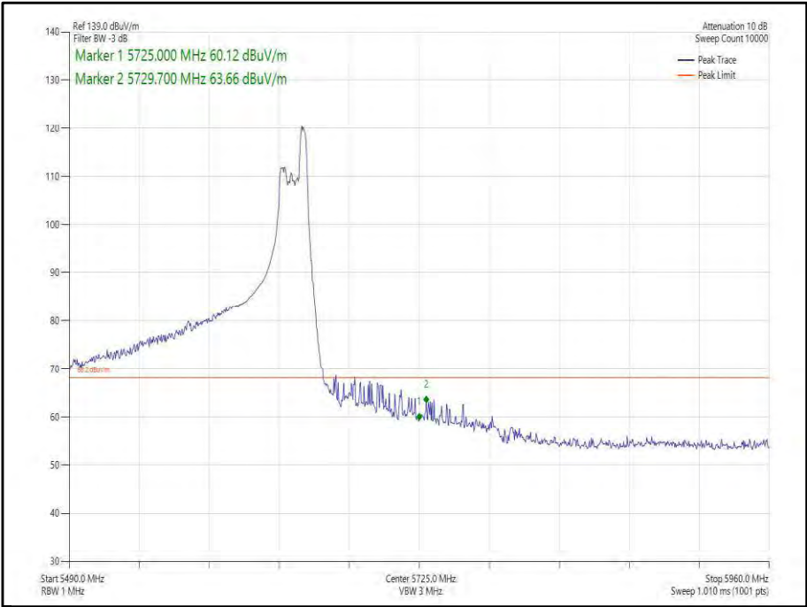
Figure 494 - 802.11ax, HE160, RU 52-52, SISO, Core 0 - 5570 MHz, Band Edge Frequency 5725 MHz
