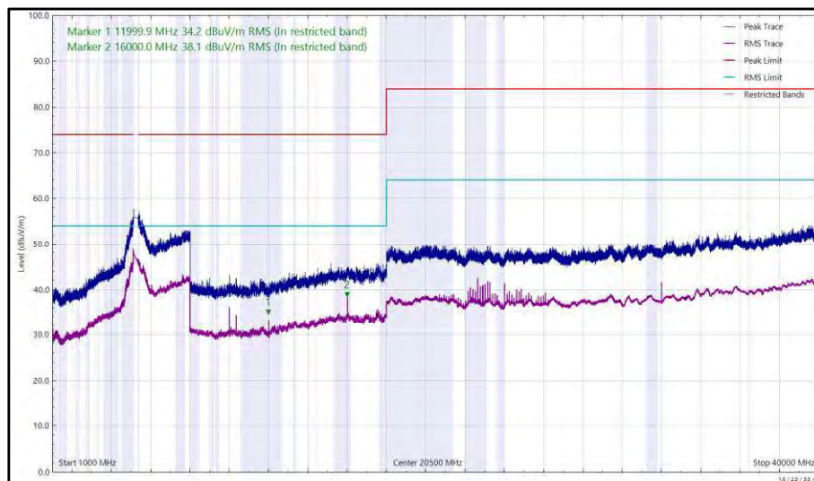
Figure 523 - U-NII-1 - 5180 MHz (CH36), HE20, RU26-0, CDD, Core 0 + Core 1, 1 GHz to 40 GHz, Horizontal
