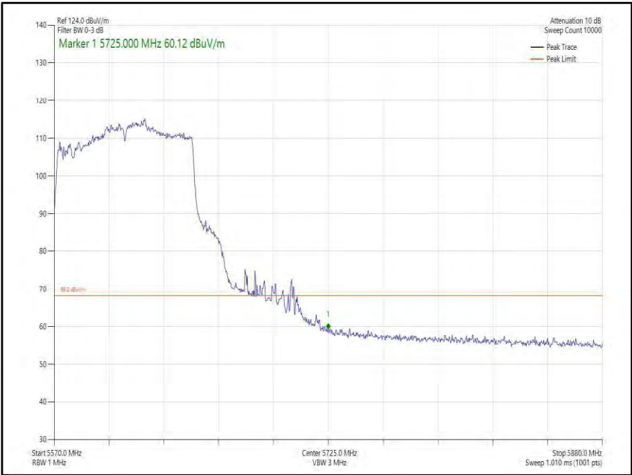
Figure 485 - 802.11ac, VHT80, TxBF, Core 0-1 - 5610 MHz, Band Edge Frequency 5725 MHz
