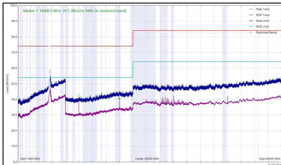
Figure 553 - U-NII-2C - 5700 MHz (CH140), HE20, RU52-37, CDD, Core 0 + Core 1, 1 GHz to 40 GHz, Vertical
