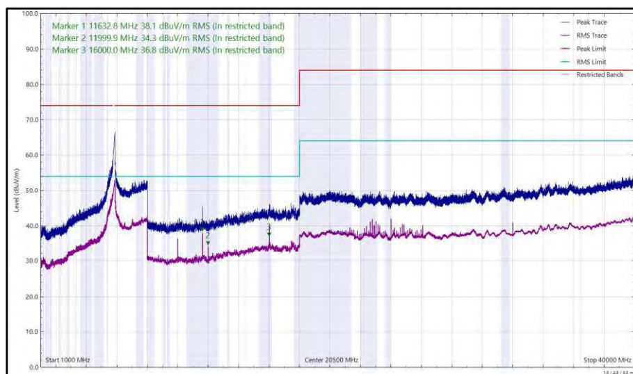
Figure 575 - U-NII-3 - 5825 MHz (CH165), HE20, RU26-0, CDD, Core 0 + Core 1, 1 GHz to 40 GHz, Horizontal
