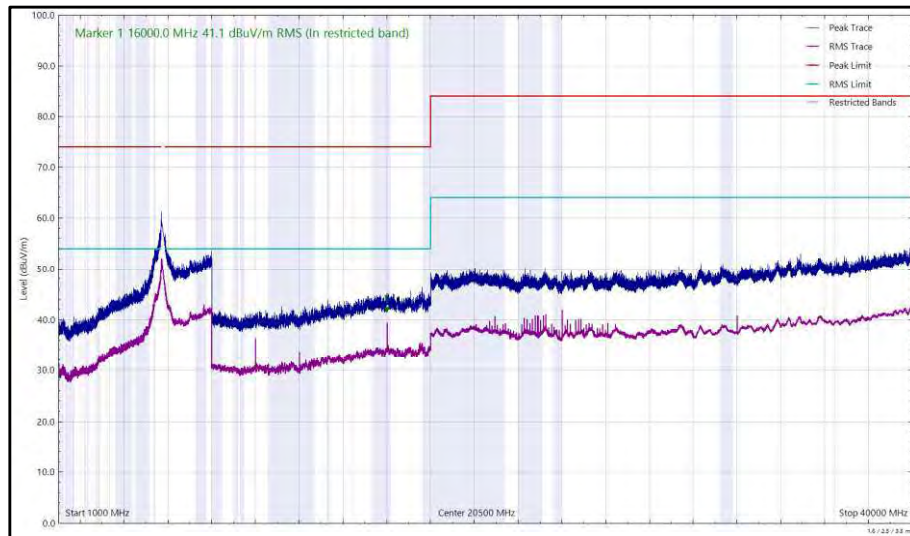
Figure 558 - U-NII-3 - 5745 MHz (CH149), VHT20, CDD, Core 0 + Core 1, 1 GHz to 40 GHz, Horizontal
