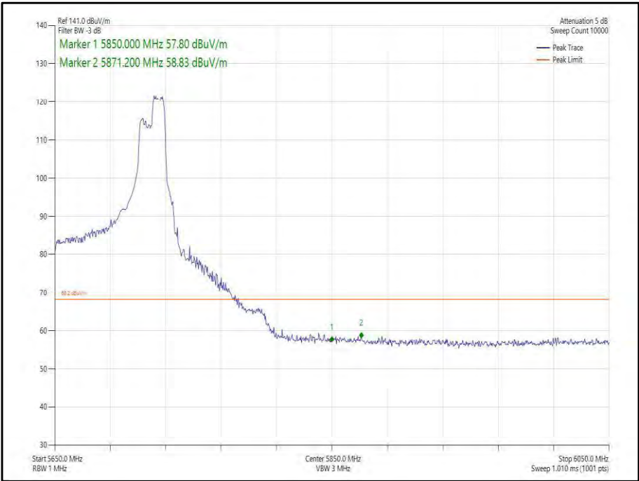
Figure 433 - 802.11ax, HE80, RU 106-60, SISO, Core 0 - 5690 MHz, Band Edge Frequency 5850 MHz
