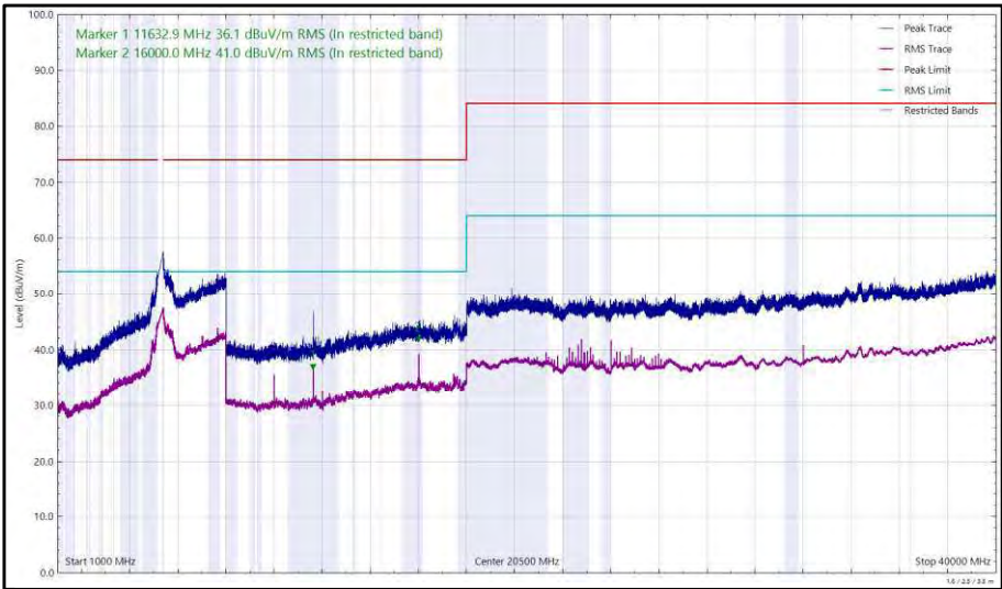
Figure 530 - U-NII-2A - 5320 MHz (CH64), 802.11a, Core 0, 1 GHz to 40 GHz, Horizontal
