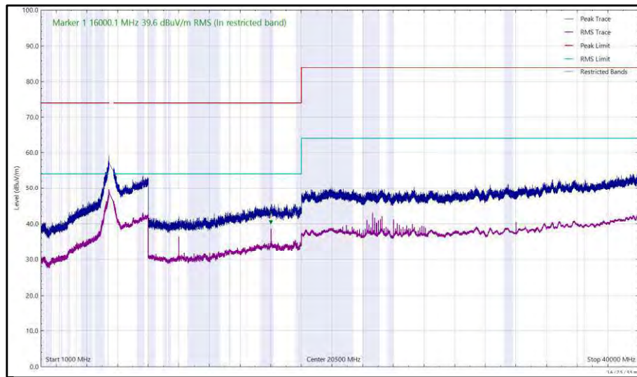
Figure 544 - U-NII-2C - 5500 MHz (CH100), HE20, RU52-37, CDD, Core 0 + Core 1, 1 GHz to 40 GHz, Horizontal
