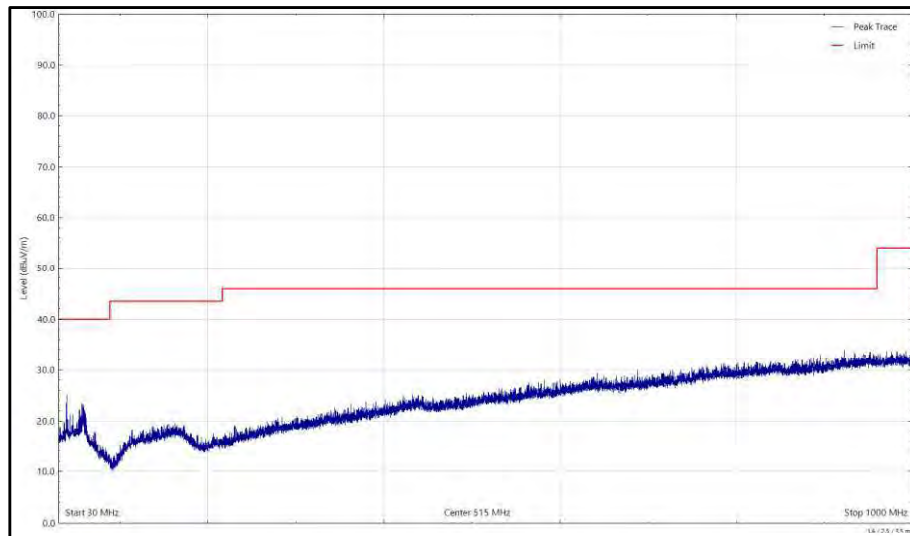
Figure 526 - U-NII-1 - 5180 MHz (CH36), VHT20, CDD, Core 0 + Core 1, 30 MHz to 1 GHz, Horizontal (Peak)
