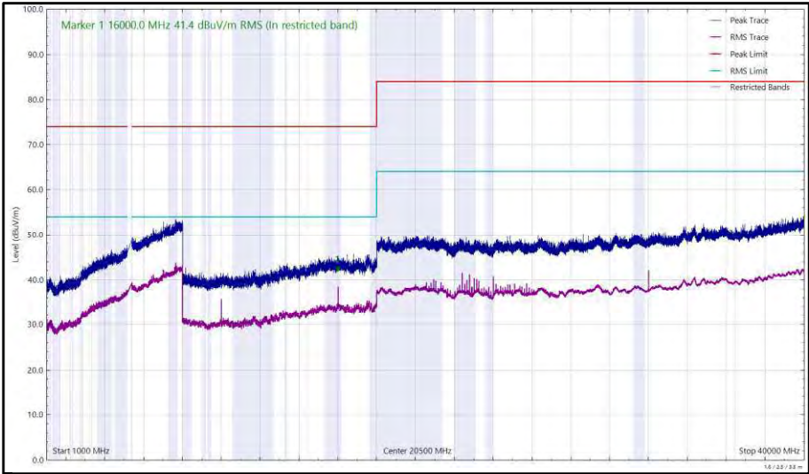
Figure 531 - U-NII-2A - 5320 MHz (CH64), 802.11a, Core 0, 1 GHz to 40 GHz, Vertical
