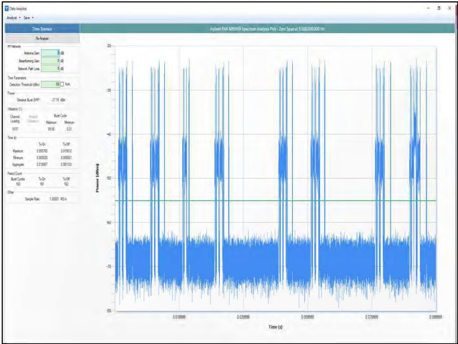
Figure 580 - Channel Loading
