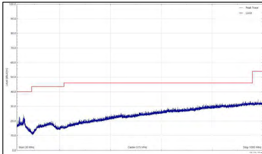
Figure 562 - U-NII-3 - 5825 MHz (CH165), 802.11a, Core 0, 30 MHz to 1 GHz, Horizontal (Peak)
