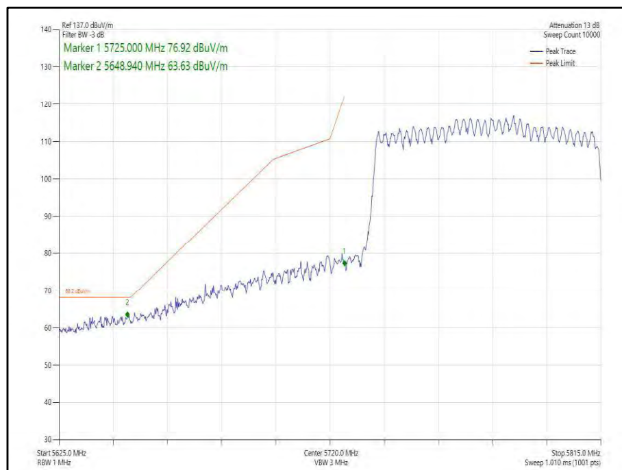
Figure 455 - 802.11ax, HE80, SU, CDD, Core 0-1 - 5775 MHz, Band Edge Frequency 5725 MHz
