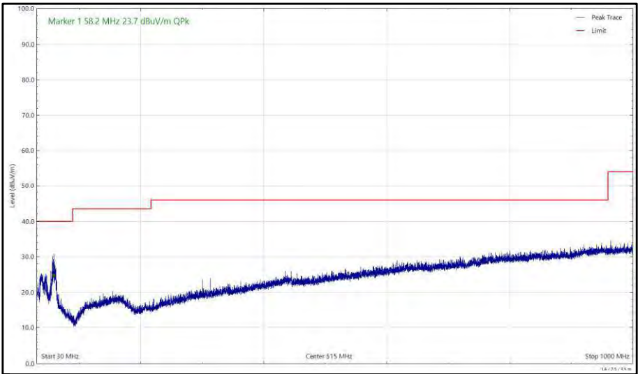
Figure 568 - U-NII-3 - 5825 MHz (CH165), 802.11a, Core 1, 30 MHz to 1 GHz, Vertical (Peak)
