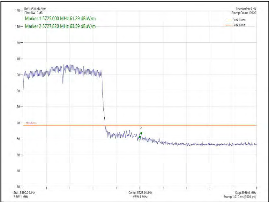
Figure 505 - 802.11ax, HE160, SU, CDD, Core 0-1 - 5570 MHz, Band Edge Frequency 5725 MHz
