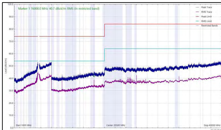
Figure 543 - U-NII-2C - 5500 MHz (CH100), VHT20, CDD, Core 0 + Core 1, 1 GHz to 40 GHz, Vertical
