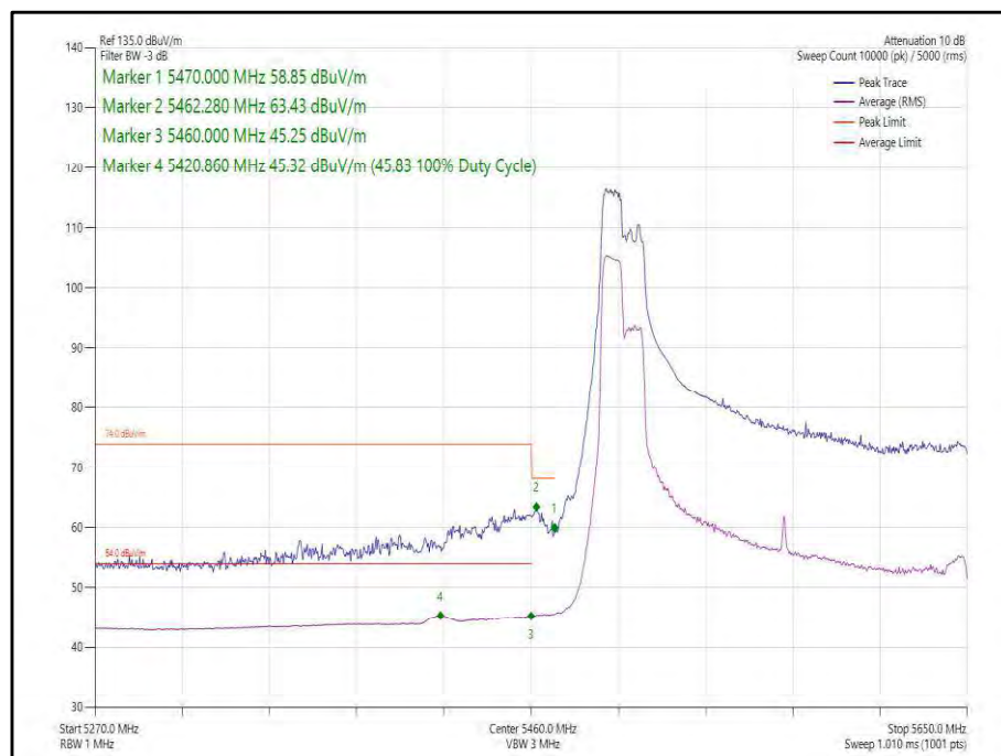
Figure 497 - 802.11ax, HE160, RU 106-53, SISO, Core 1 - 5570 MHz, Band Edge Frequency 5470 MHz
