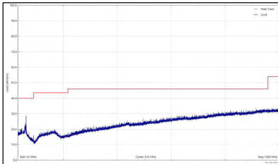
Figure 570 - U-NII-3 - 5825 MHz (CH165), VHT20, CDD, Core 0 + Core 1, 30 MHz to 1 GHz, Horizontal (Peak)
