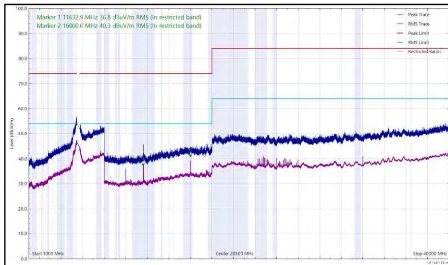
Figure 538 - U-NII-2C - 5500 MHz (CH100), 802.11a, Core 0, 1 GHz to 40 GHz, Horizontal
