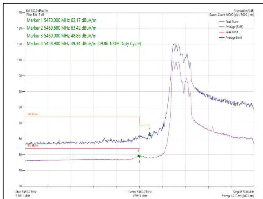
Figure 453 - 802.11ax, HE80, RU 106-53, CDD, Core 0-1 - 5530 MHz, Band Edge Frequency 5470 MHz
