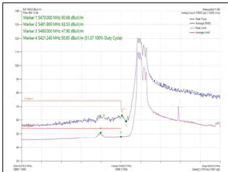
Figure 509 - 802.11ax, HE160, RU 106-53, SDM, Core 0-1 - 5570 MHz, Band Edge Frequency 5470 MHz
