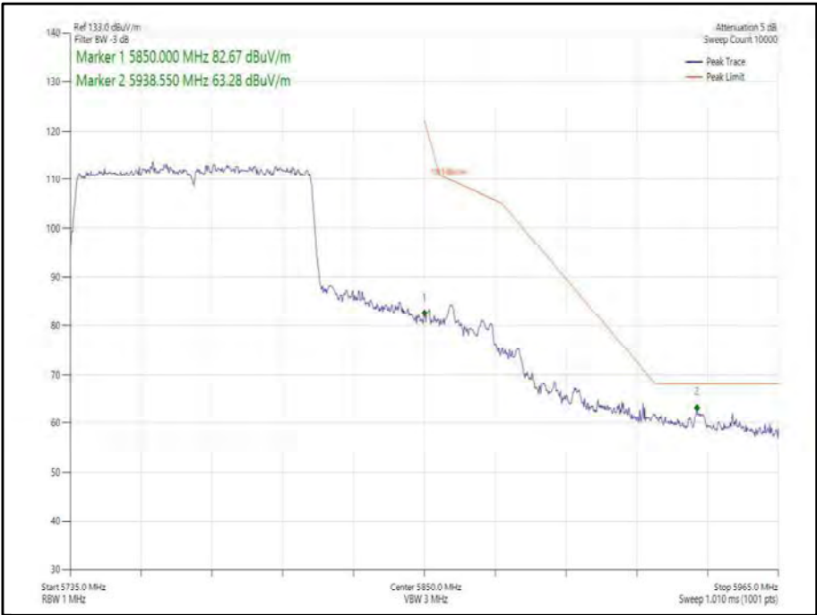
Figure 446 - 802.11ac, VHT80, SISO, Core 1 - 5775 MHz, Band Edge Frequency 5850 MHz
