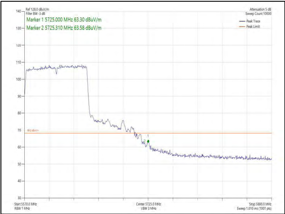
Figure 442 - 802.11ac, VHT80, SISO, Core 1 - 5610 MHz, Band Edge Frequency 5725 MHz
