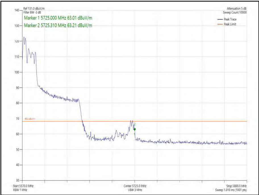
Figure 459 - 802.11ax, HE80, RU 52-37, CDD, Core 0-1 - 5610 MHz, Band Edge Frequency 5725 MHz
