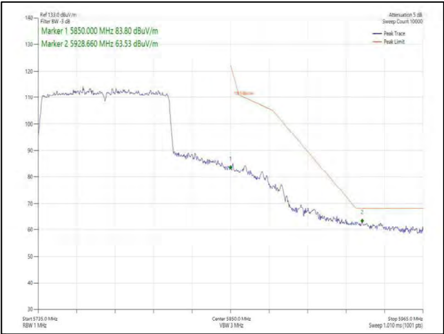
Figure 431 - 802.11ac, VHT80, SISO, Core 0 - 5775 MHz, Band Edge Frequency 5850 MHz
