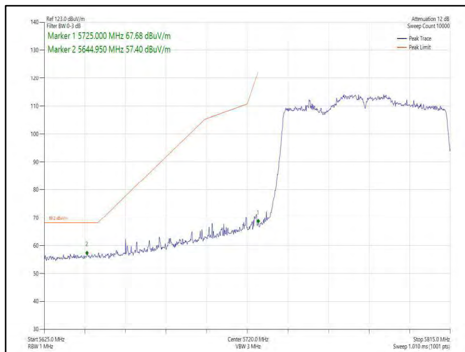
Figure 483 - 802.11ac, VHT80, TxBF, Core 0-1 - 5775 MHz, Band Edge Frequency 5725 MHz
