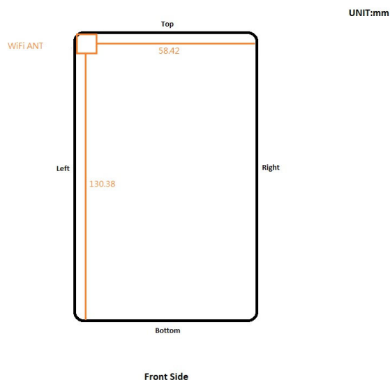
Fig.18 Antenna position of EUT (WLAN)
