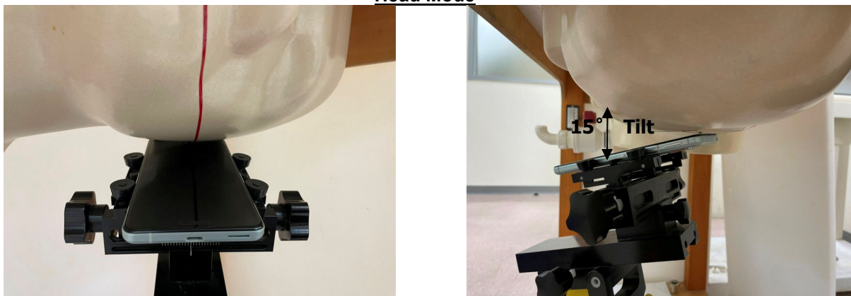
Fig.6 Left Head Section / Ear-Tilt Position(15°)
