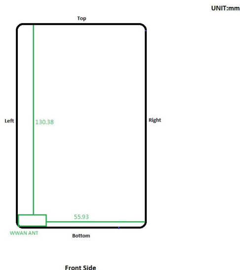
Fig.17 Antenna position of EUT (WWAN)
