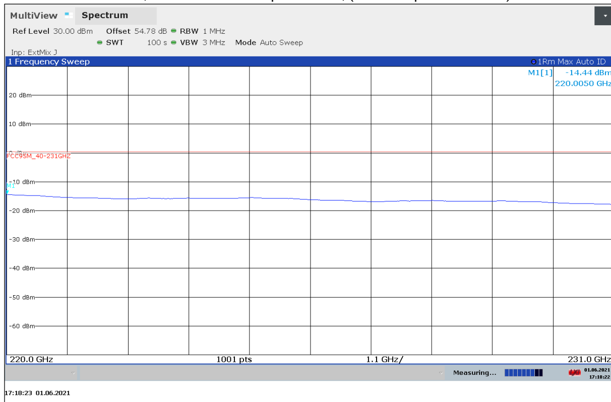
Plot 14: 220 GHz – 231 GHz, vertical / horizontal polarization, (Valid for specified Modes)
