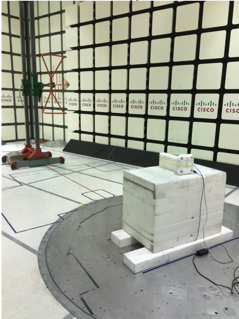
AIR-CAP3702P-B-K9 Radiated Test setup photo 30MHz to 1GHz
