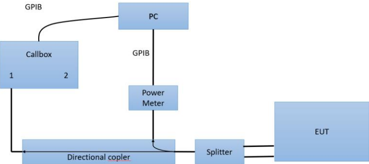
(b) Appendix D – Test Setup Photo 4
