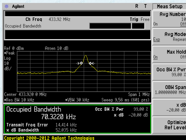
ASK
