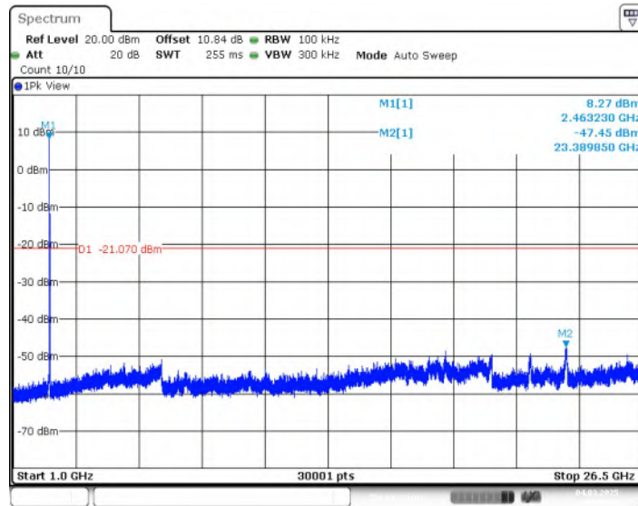
Fig.11 Conducted Spurious Emission (1GHz-26.5GHz, 802.11b, CH11)
