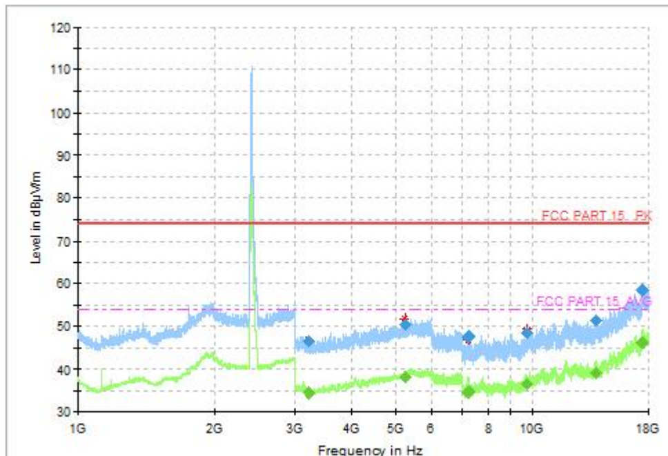
Fig.45 Radiated Spurious Emission (802.11be-EHT20, CH11, 1GHz-18GHz, MIMO)
