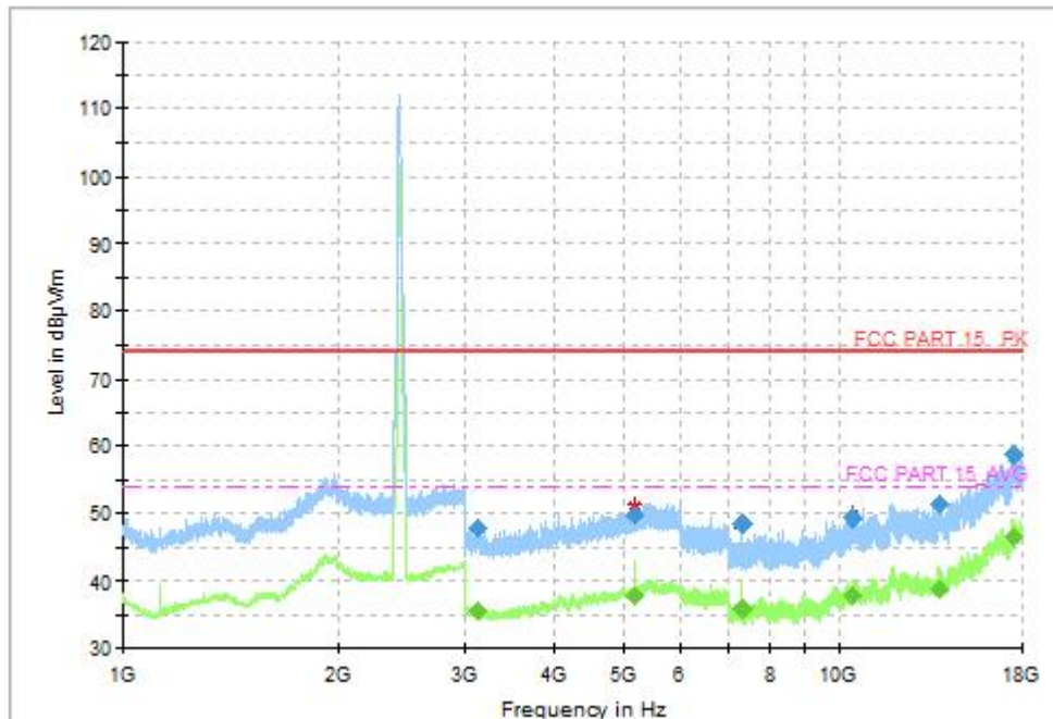
Fig.44 Radiated Spurious Emission (802.11be-EHT20, CH6, 1GHz-18GHz, MIMO)
