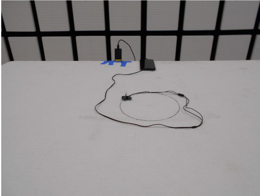
RADIATED PHOTO (>1GHz 2.4 WLAN/BLE/BT CHAIN 0/1)
