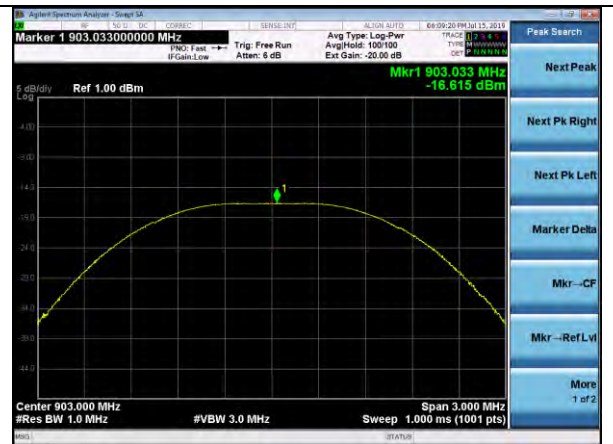
Pout, DR13 Low Channel Laird Rev_B, Power Setting -17
