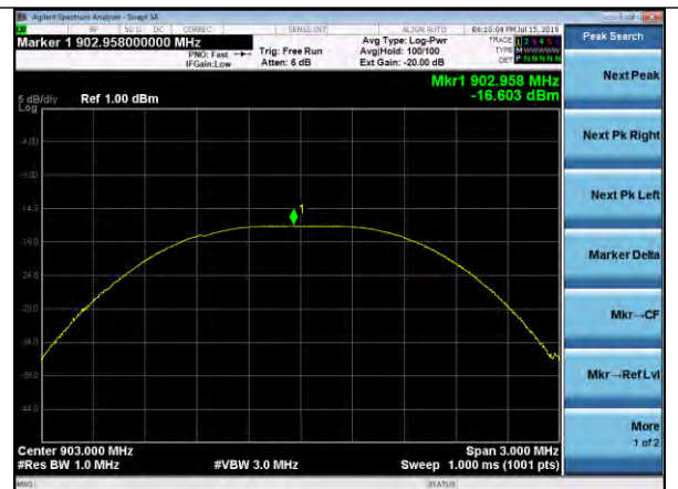
Pout, DR4 Low Channel Laird Rev_B, Power Setting -17
