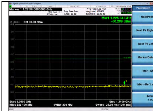
1000-1240 MHz, DR4 Low Channel Laird Rev_B, Power Setting 18
