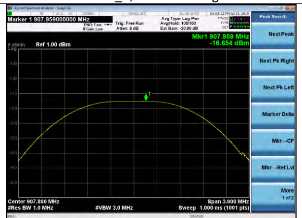
Pout, DR4 Mid Channel Laird Rev_B, Power Setting -17
