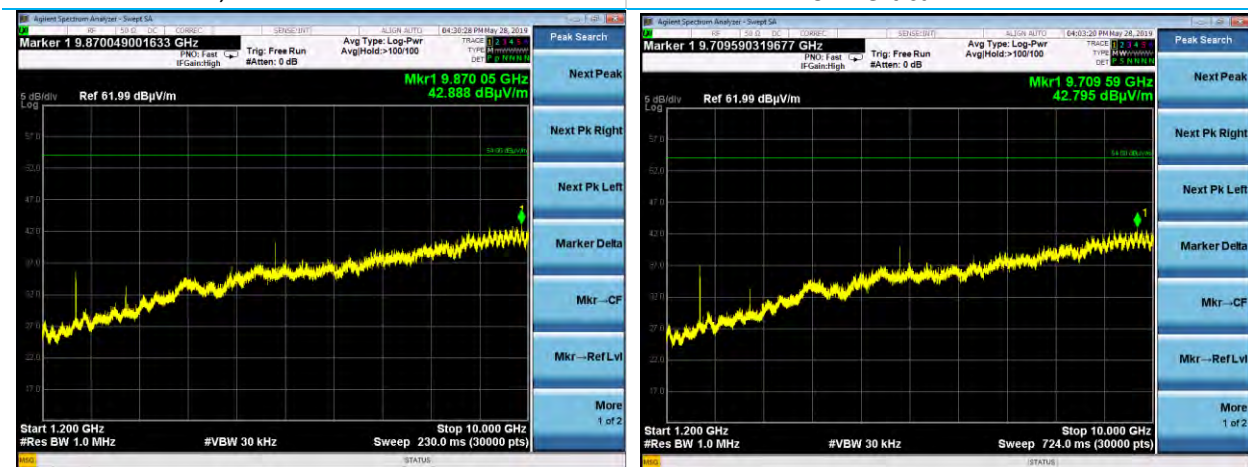
1.2-10 GHz, Horizontal Antenna, Low Ch, 500k, DR4, EUT Side
