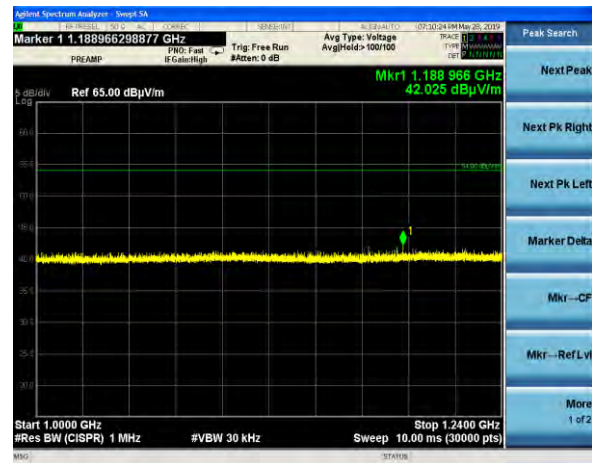
1000-1240 MHz, Horizontal Antenna, High Channel, 500 kHz, DR 13, Reduced VBW
