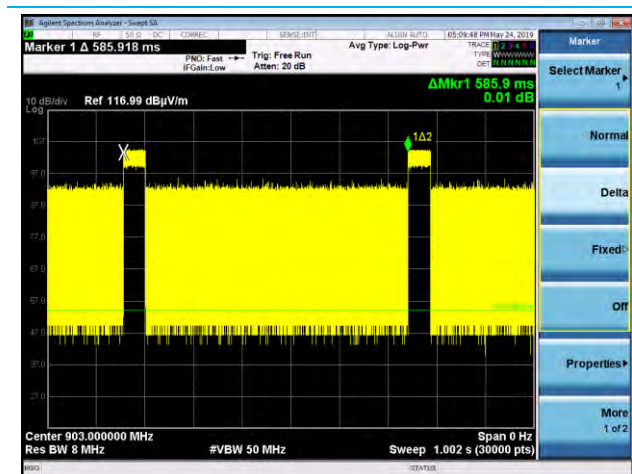
DR4 Duty Cycle
