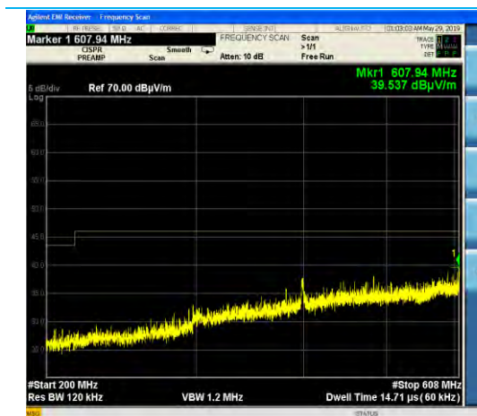
200-608 MHz, Horizontal Antenna, Low Ch, 500kHz, DR13
