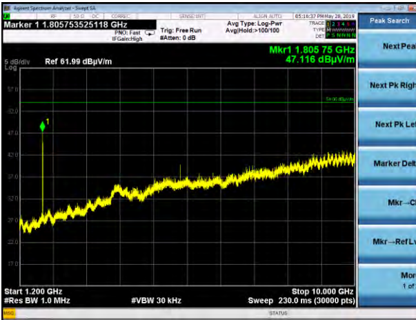
1.2-10 GHz, Horizontal Antenna, Low Ch, 500k, DR4, EUT Flat
