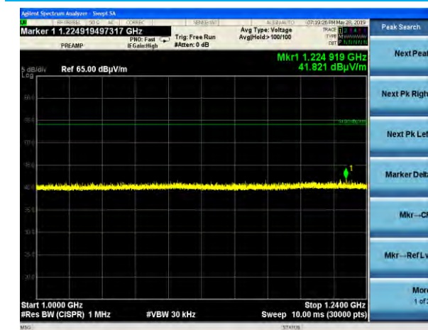
1000-1240 MHz, Vertical Antenna, High Channel, 500 kHz, DR 13, Reduced VBW
