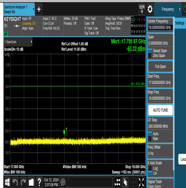
Thread-Ant1-2405-17000~19000-PASS
