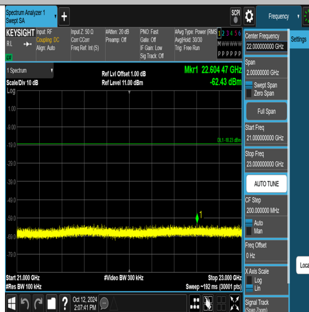
Thread-Ant1-2405-21000~23000-PASS
