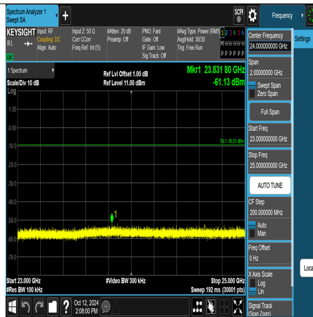
Thread-Ant1-2405-23000~25000-PASS
