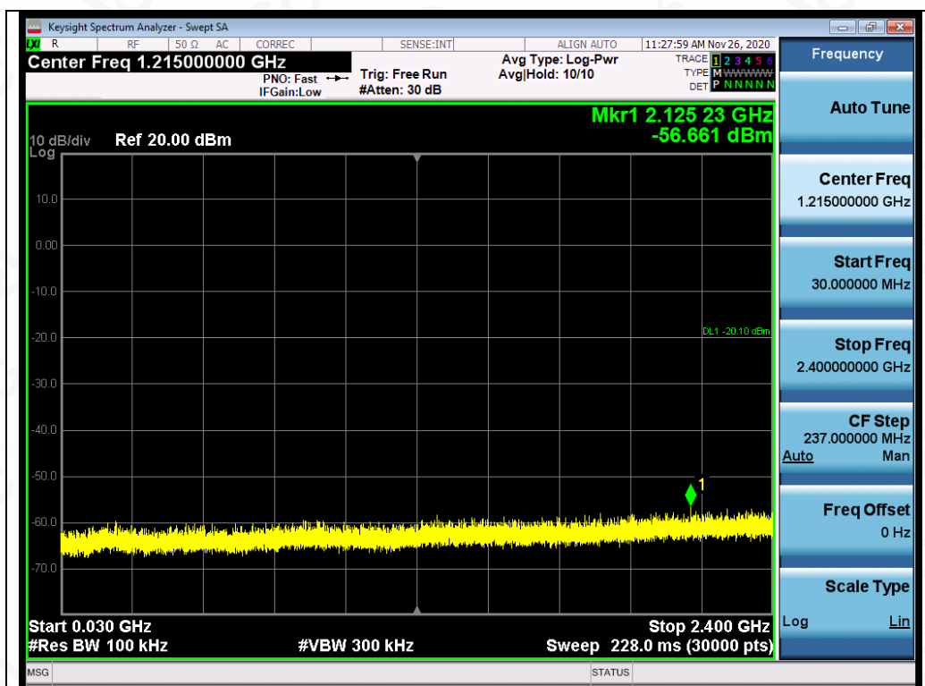
Test_Graph_LE1M_2440_1Mbps_Lower Band Emissions
