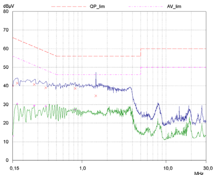
Picture 28: AC power line emissions, line L.
