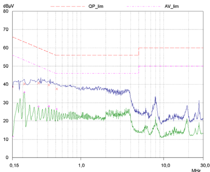
Picture 29: AC power line emissions, line N
