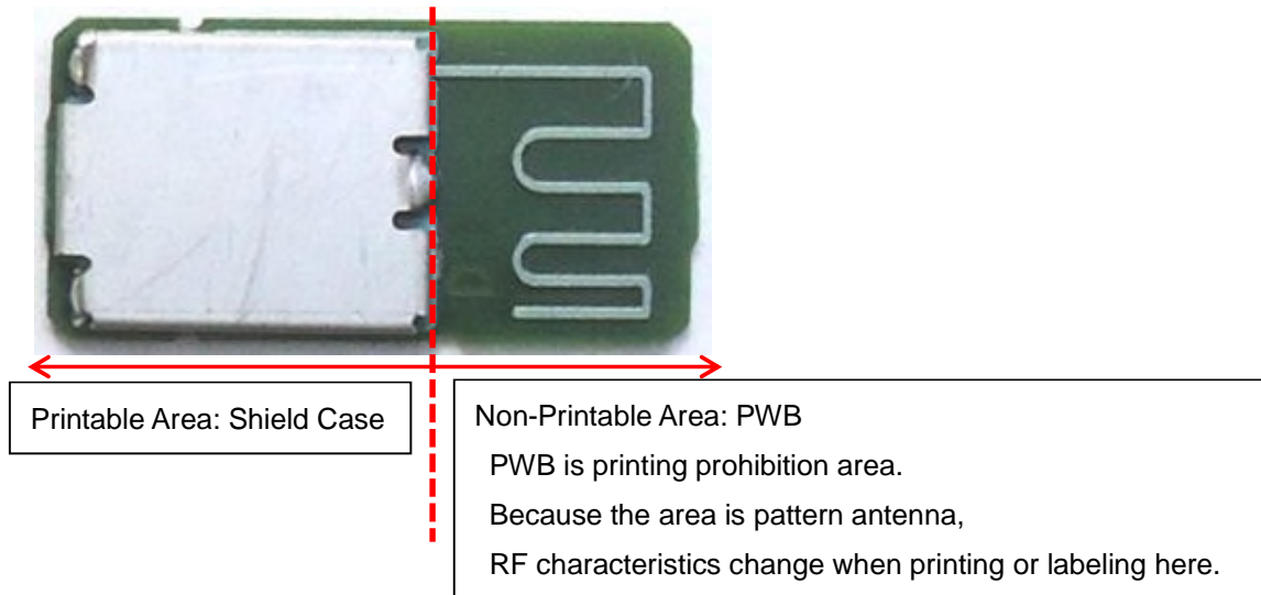
BTS05 module External View
