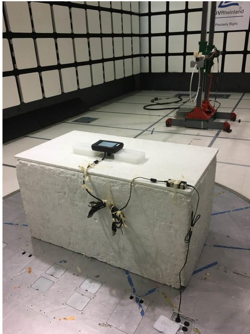
Figure 1: Test Setup for Radiated Emissions 9 kHz to 30 MHz - Rear
