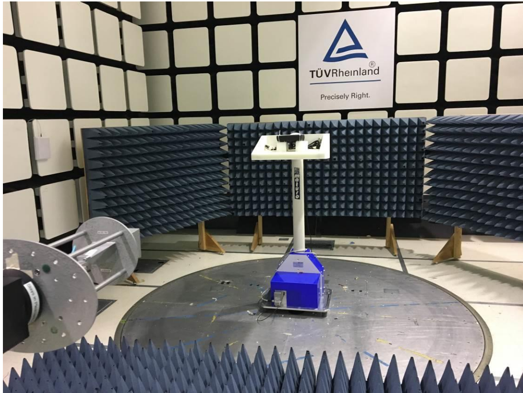
Figure 4: Test Setup for Radiated Emissions 18 GHz to 26.5 GHz
