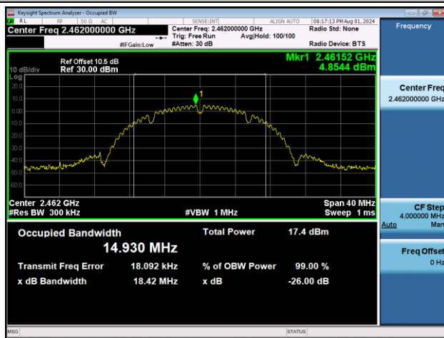
11B-Ant1-2462
