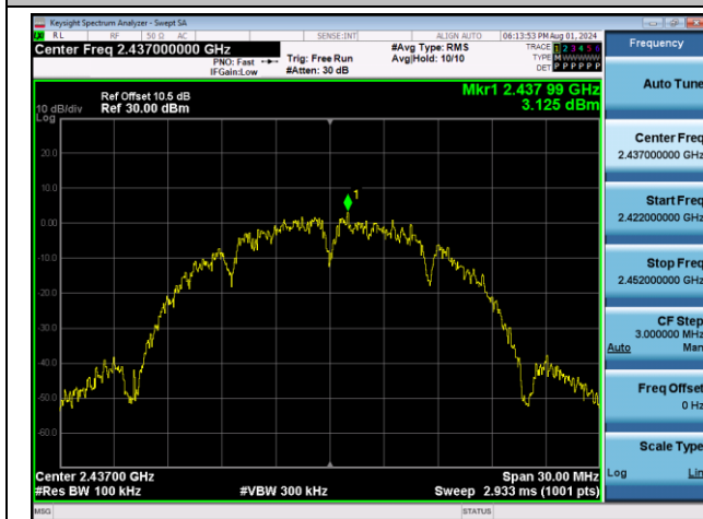
11B-Ant1-2437-0~Reference-PASS
