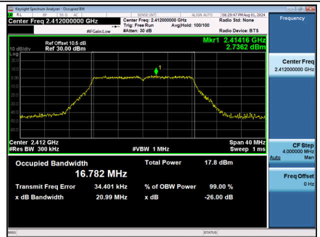
11G-Ant1-2412
