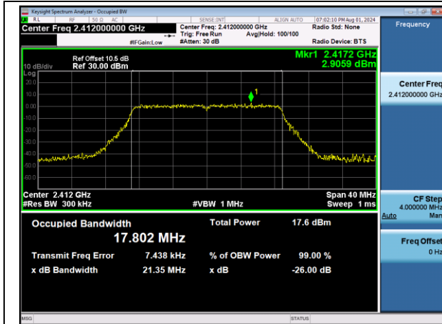
11N20SISO-Ant1-2412
