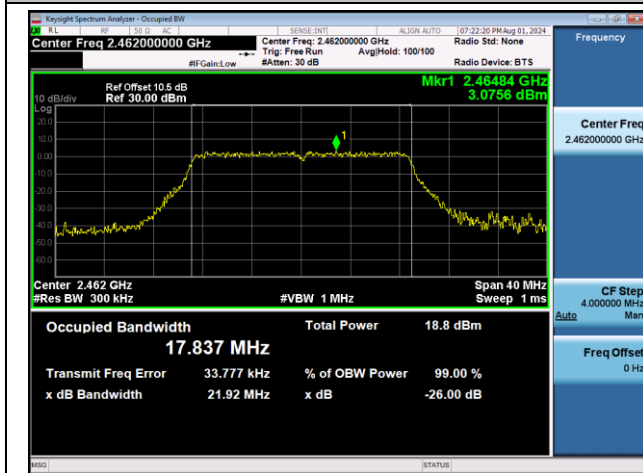
11N20SISO-Ant1-2462
