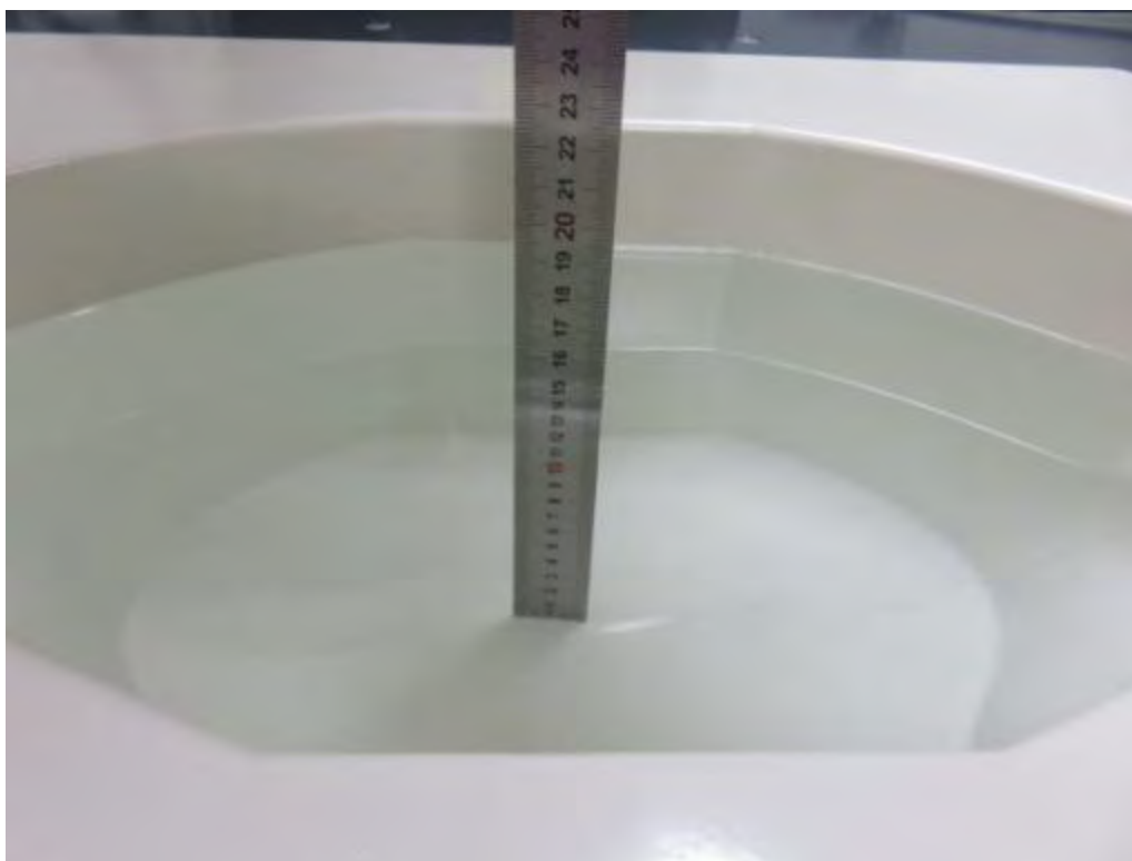
Photograph of the depth in the Body Phantom (5200MHz, 16.1cm depth)
