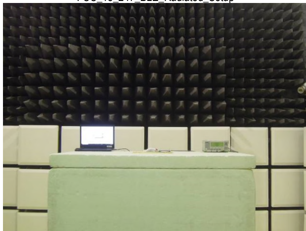
FCC_15_247_BLE_Radiated_Setup
