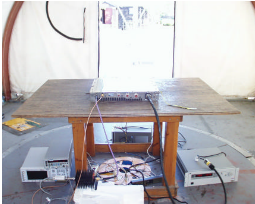
Below 1 GHz Radiated Emission Setup
