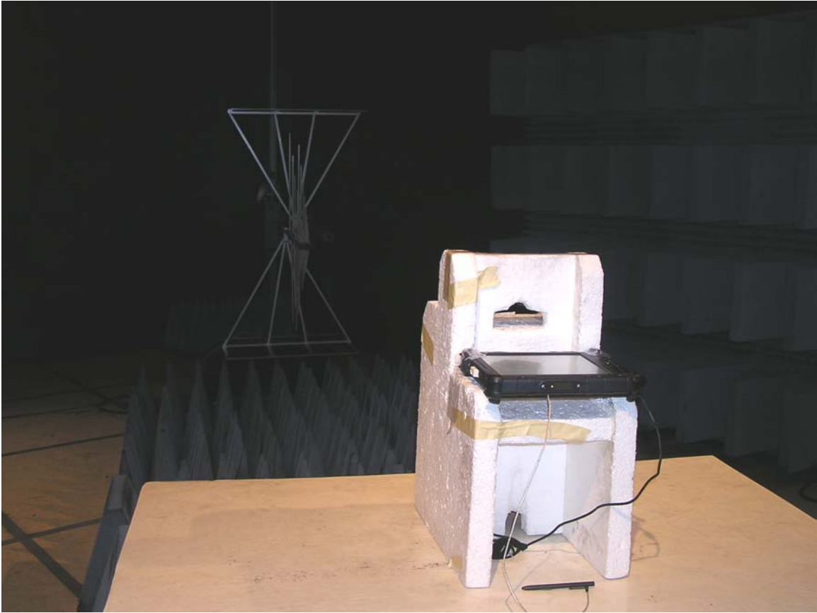
Test setup – Radiated emissions (above 1GHz)
