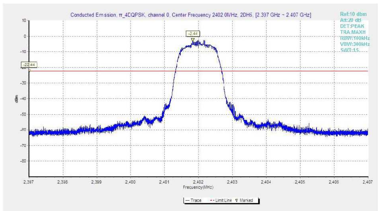
Fig. 22 Conducted Spurious Emission ( \pi/4 QPSK, Ch0, 2.402GHz)
