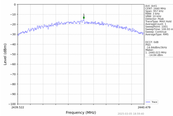
Middle channel
