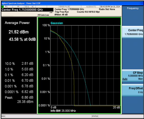
Band4-3MHz-16QAM-20385-1RB#0-PASS
