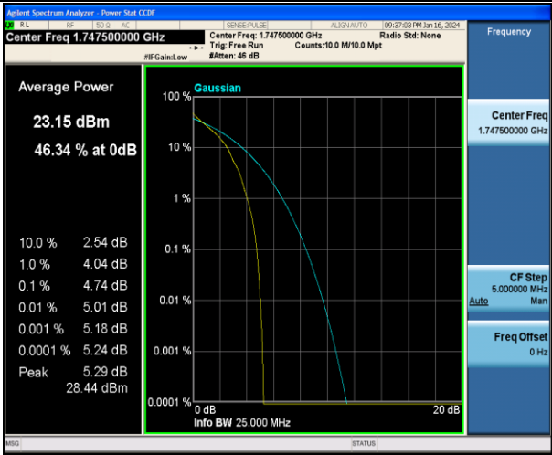
Band4-15MHz-QPSK-20325-1RB#0-PASS
