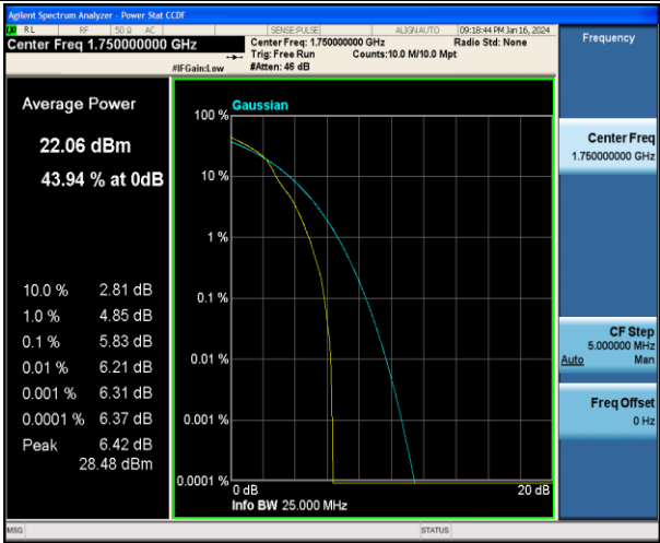
Band4-10MHz-16QAM-20350-1RB#0-PASS
