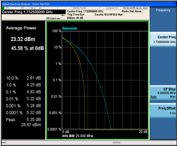
Band4-15MHz-QPSK-20175-1RB#0-PASS
