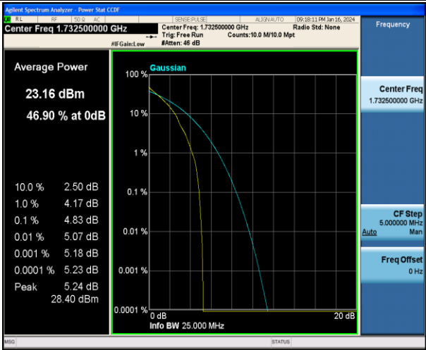
Band4-10MHz-QPSK-20175-1RB#0-PASS
