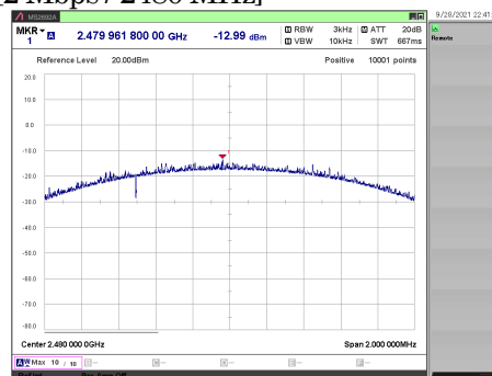
[2 Mbps / 2480 MHz]
