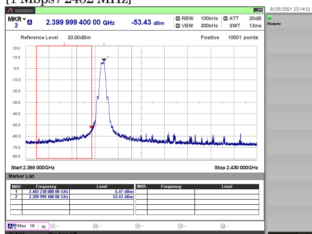
[1 Mbps / 2402 MHz]
