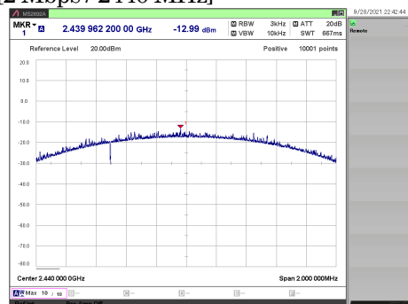
[2 Mbps / 2440 MHz]
