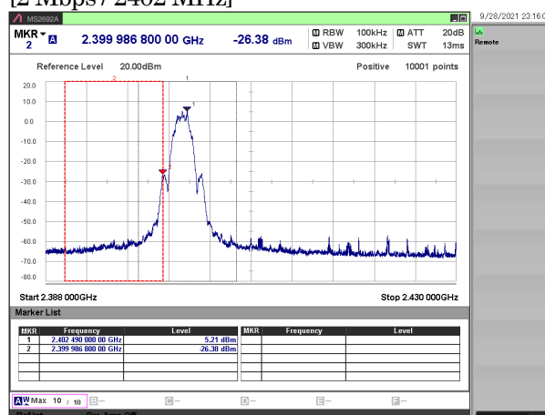
[2 Mbps / 2402 MHz]
