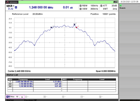
[2 Mbps / 2440 MHz]
