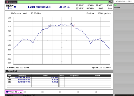
[2 Mbps / 2480 MHz]
