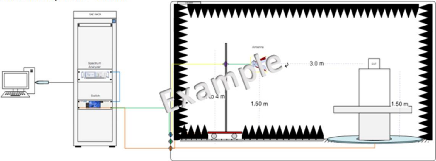
Radiated Setup 1 GHz – 6.4 GHz
