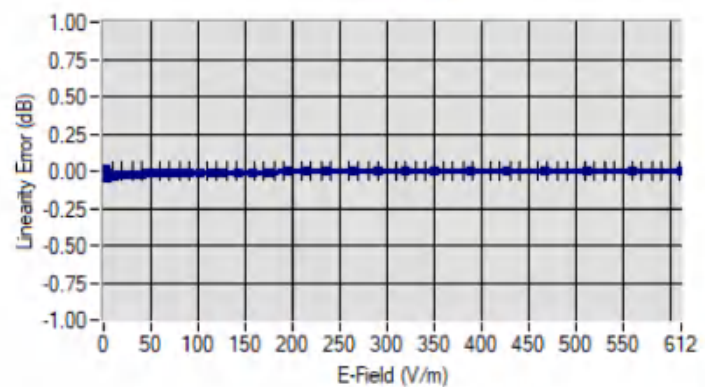
Linearity
