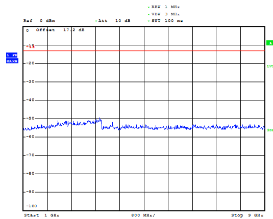
LTE Band 14 5MHz CH-High 1GHz~9GHz
