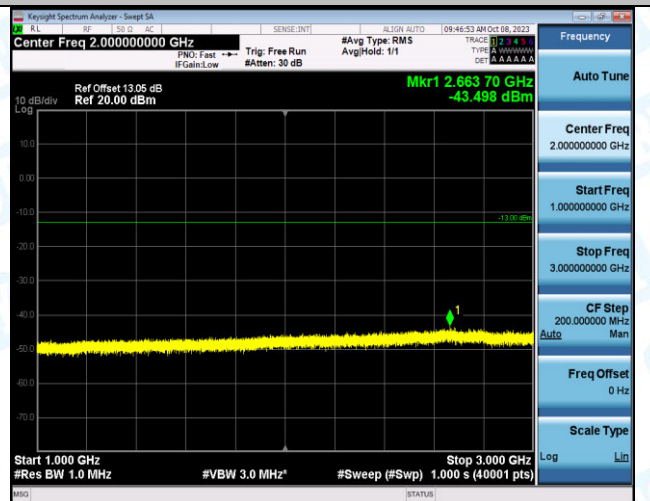
Band2_5MHz_QPSK_18900_1RB#0_1000~3000_1000~3 000
