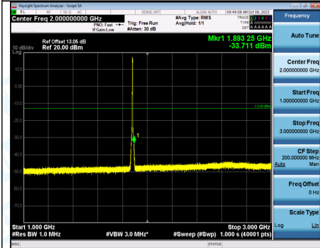
Band2_5MHz_16QAM_18900_25RB#0_1000~3000_1000~3000
