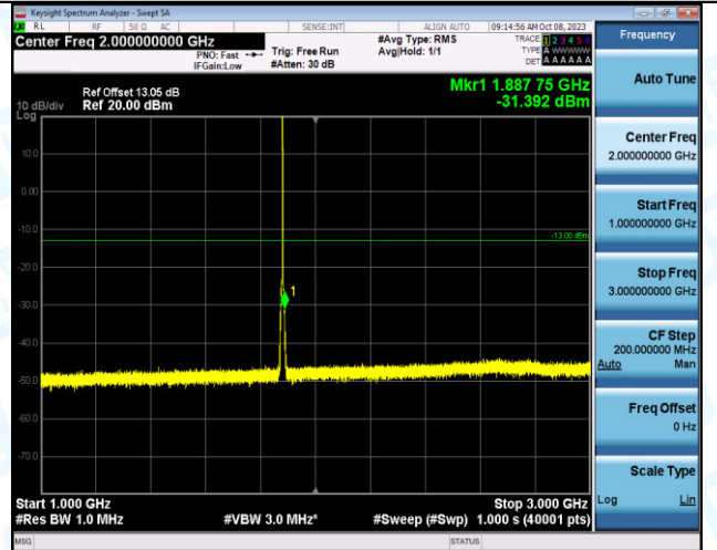
Band2_3MHz_QPSK_18900_15RB#0_1000~3000_1000~3000
