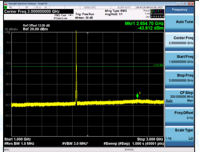
Band2_5MHz_QPSK_18625_1RB#0_1000~3000_1000~3000
