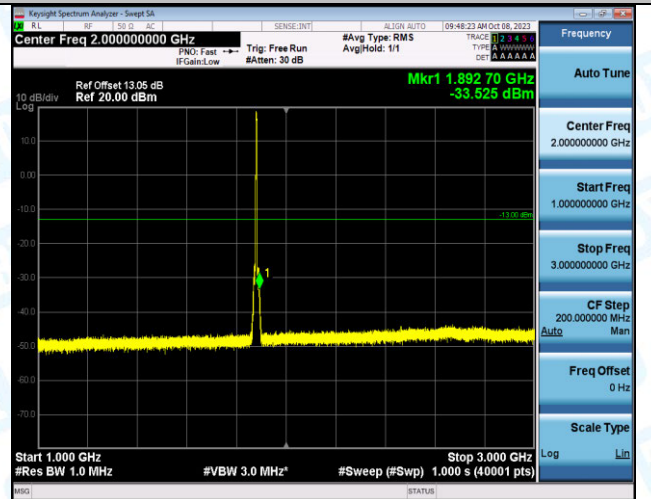
Band2_5MHz_QPSK_18900_25RB#0_1000~3000_1000~3000
