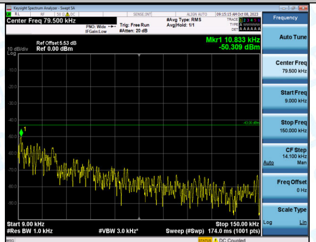
Band2_3MHz_16QAM_18900_15RB#0_0.009~0.15_0.009~0.15
