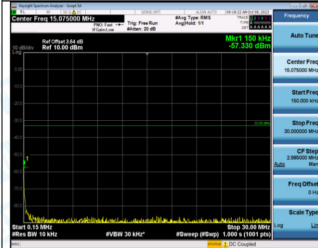
Band2_3MHz_16QAM_19185_15RB#0_0.15~30_0.15~30
