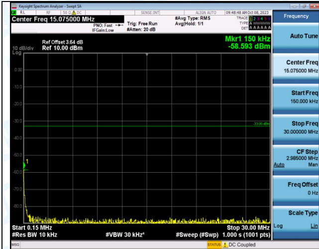
Band2_5MHz_16QAM_18900_25RB#0_0.15~30_0.15~30
