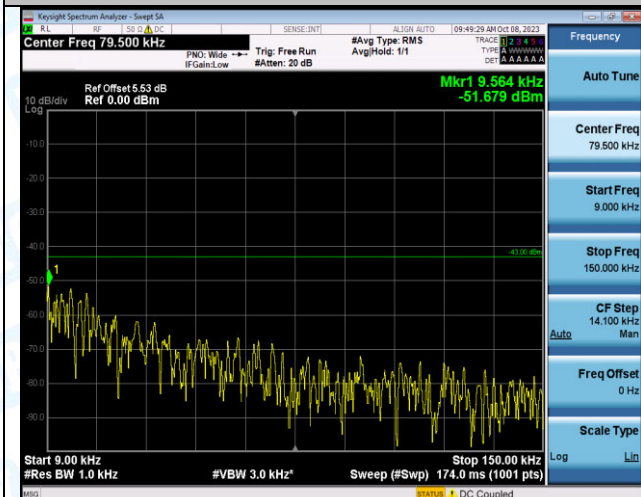
Band2_5MHz_QPSK_19175_1RB#0_0.009~0.15_0.009~0.15
