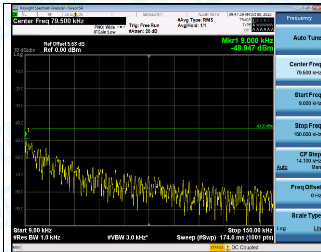
Band2_5MHz_QPSK_18900_25RB#0_0.009~0.15_0.009~0.15
