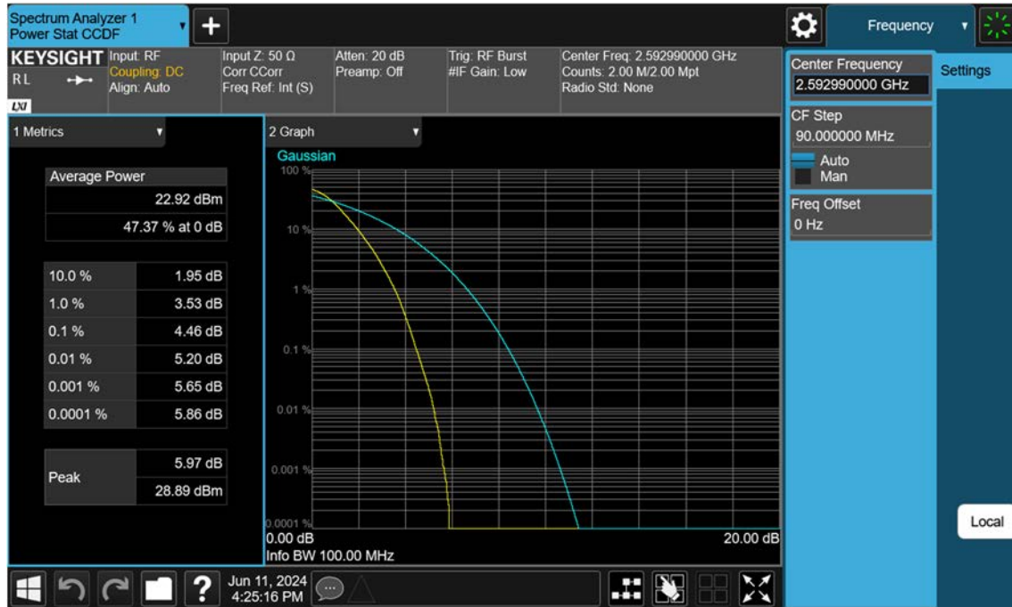
Sub6 n41_100 M_PAR_Mid_BPSK_FullRB
