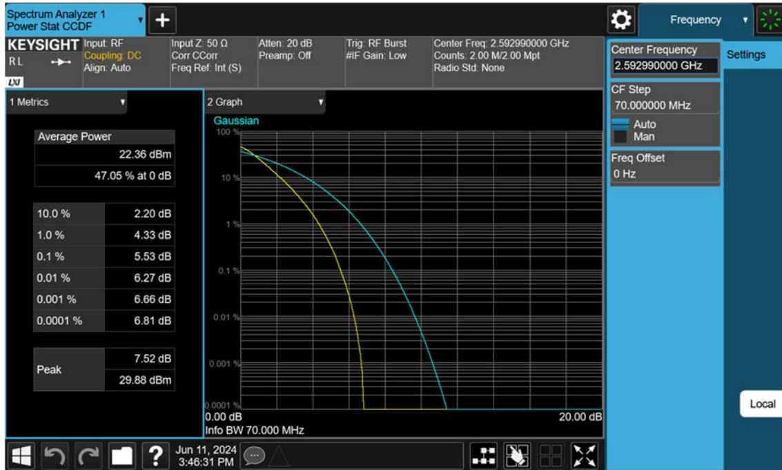
Sub6 n41_70 M_PAR_Mid_QPSK_FullRB
