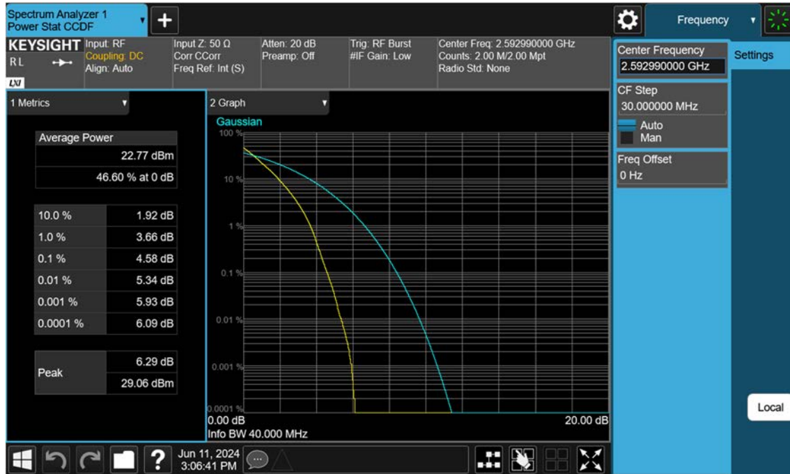
Sub6 n41_40 M_PAR_Mid_BPSK_FullRB
