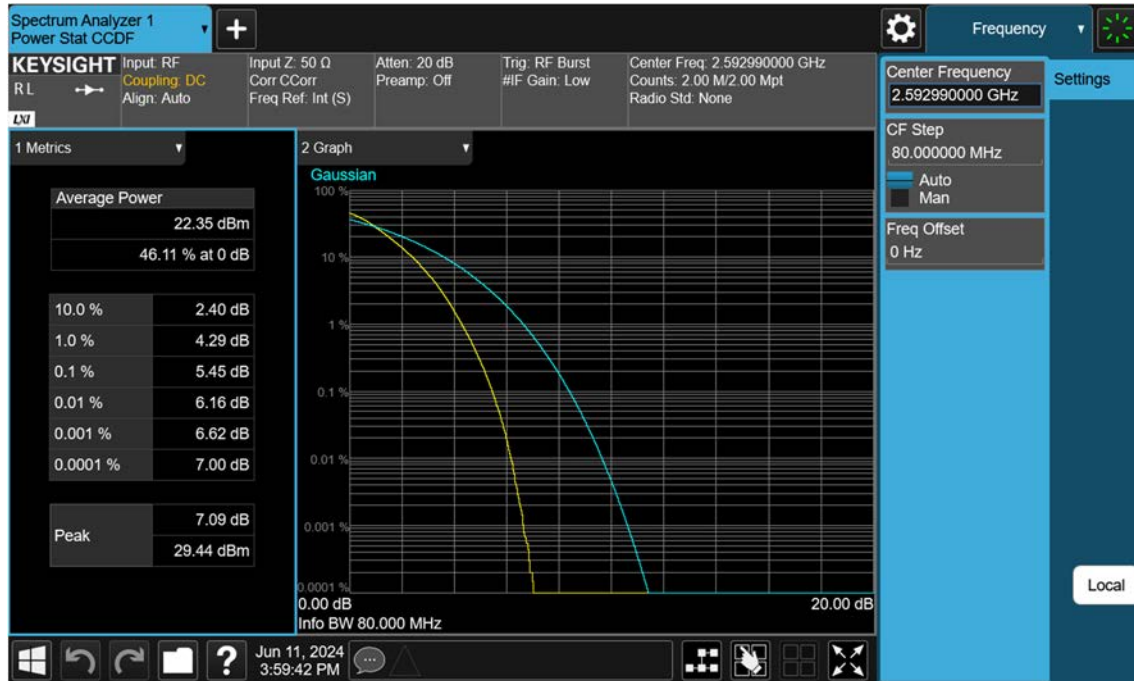
Sub6 n41_80 M_PAR_Mid_QPSK_FullRB
