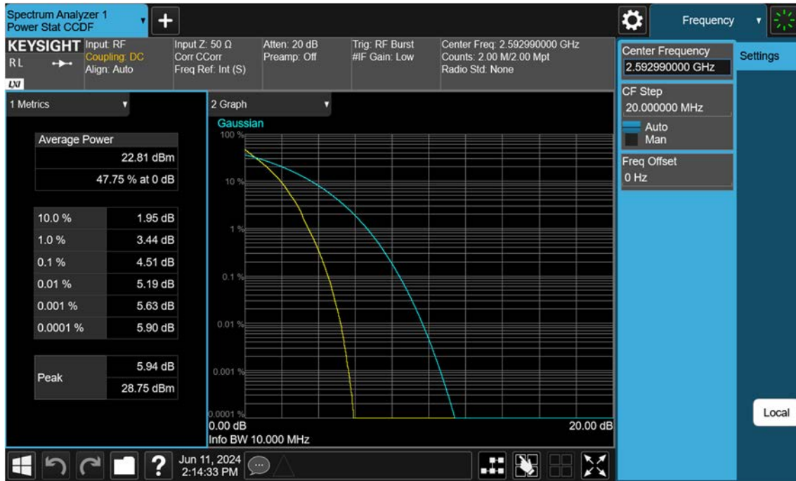
Sub6 n41_10 M_PAR_Mid_BPSK_FullRB
