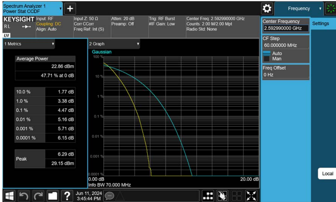
Sub6 n41_70 M_PAR_Mid_BPSK_FullRB
