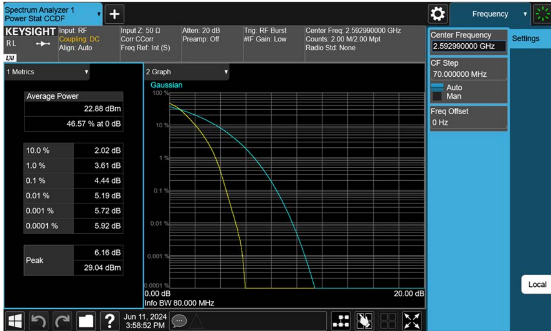
Sub6 n41_80 M_PAR_Mid_BPSK_FullRB
