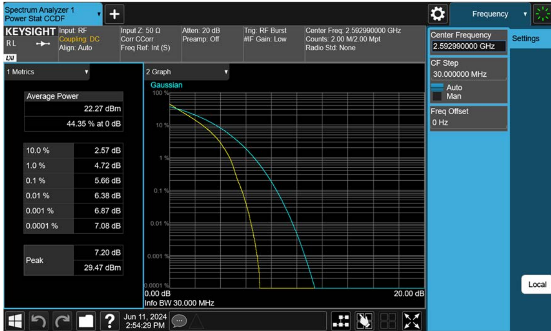
Sub6 n41_30 M_PAR_Mid_QPSK_FullRB
