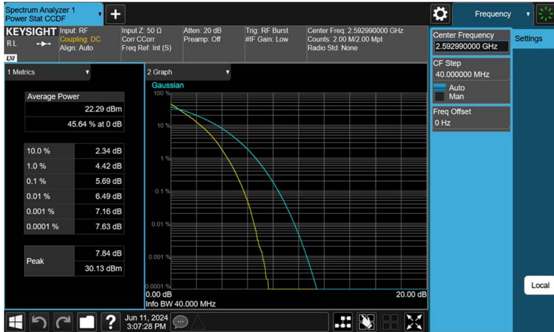
Sub6 n41_40 M_PAR_Mid_QPSK_FullRB
