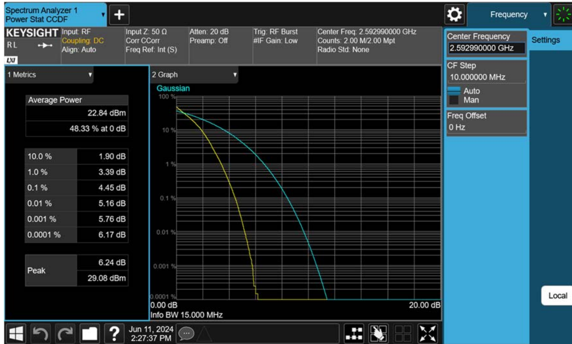
Sub6 n41_15 M_PAR_Mid_BPSK_FullRB
