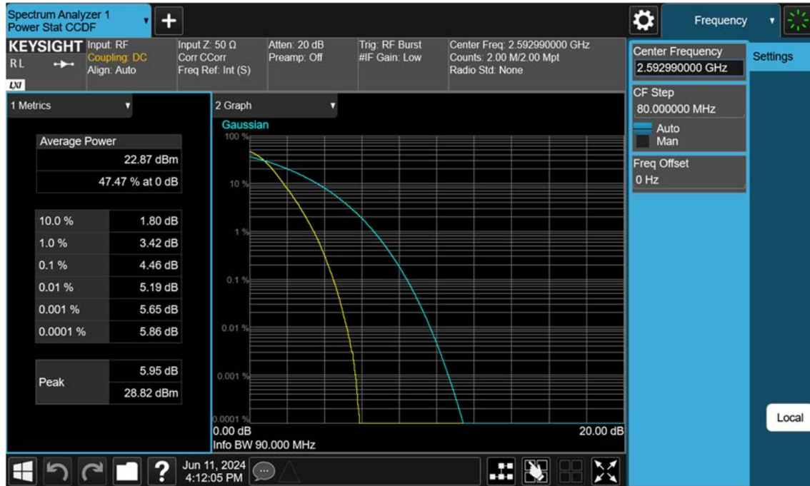
Sub6 n41_90 M_PAR_Mid_BPSK_FullRB
