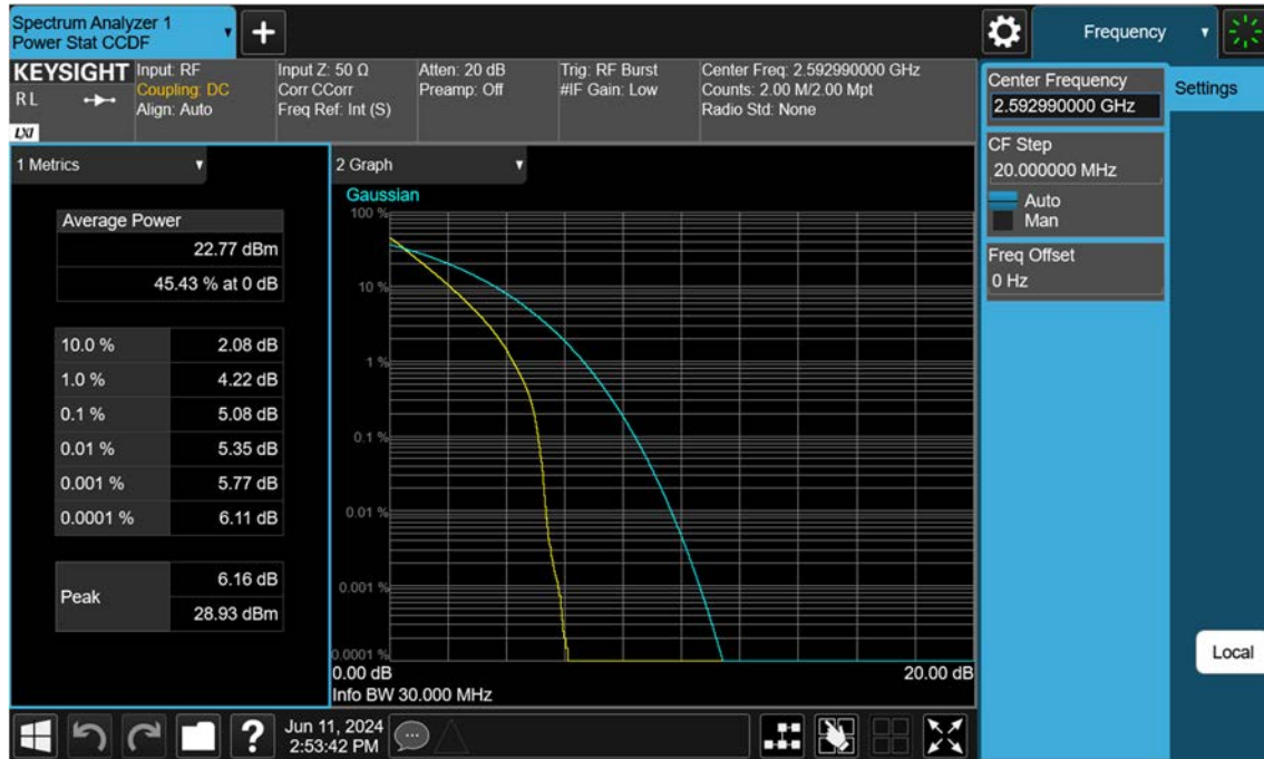
Sub6 n41_30 M_PAR_Mid_BPSK_FullRB
