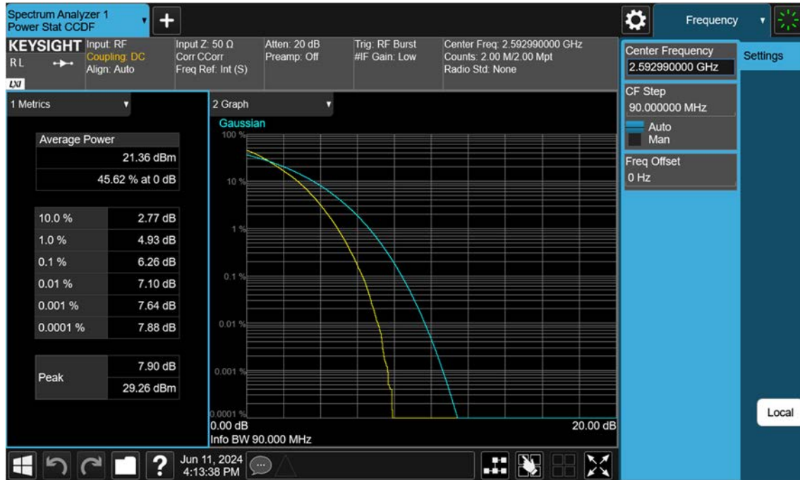
Sub6 n41_90 M_PAR_Mid_16QAM_FullRB
