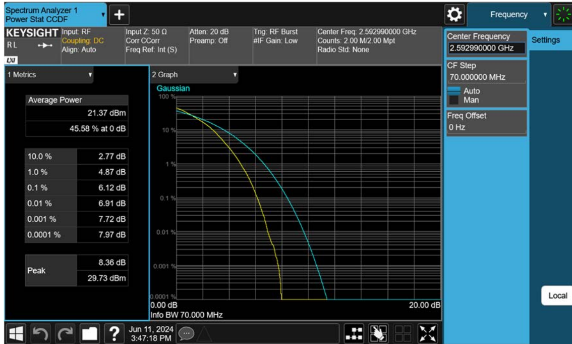
Sub6 n41_70 M_PAR_Mid_16QAM_FullRB
