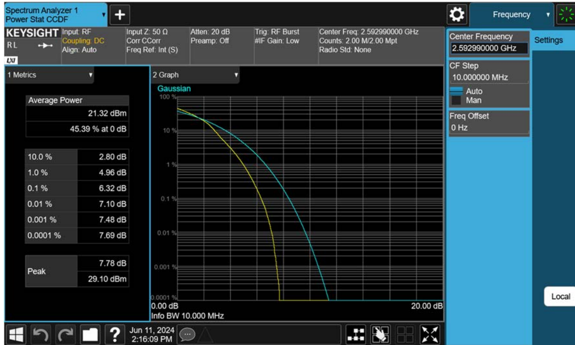
Sub6 n41_10 M_PAR_Mid_16QAM_FullRB
