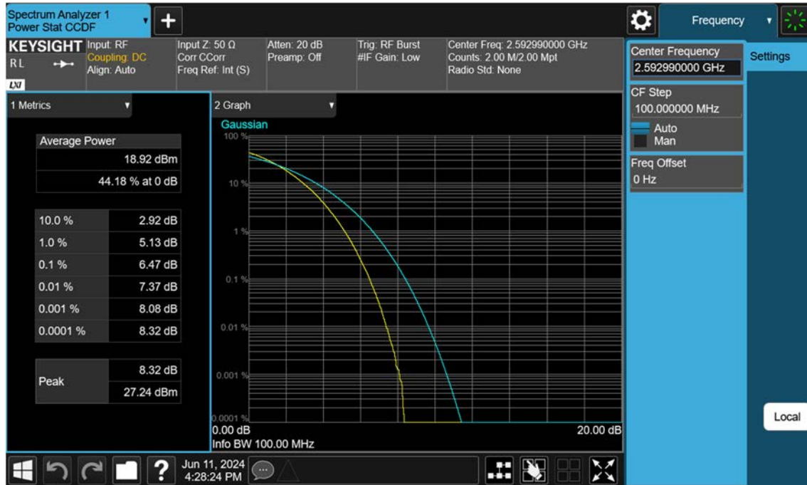
Sub6 n41_100 M_PAR_Mid_256QAM_FullRB
