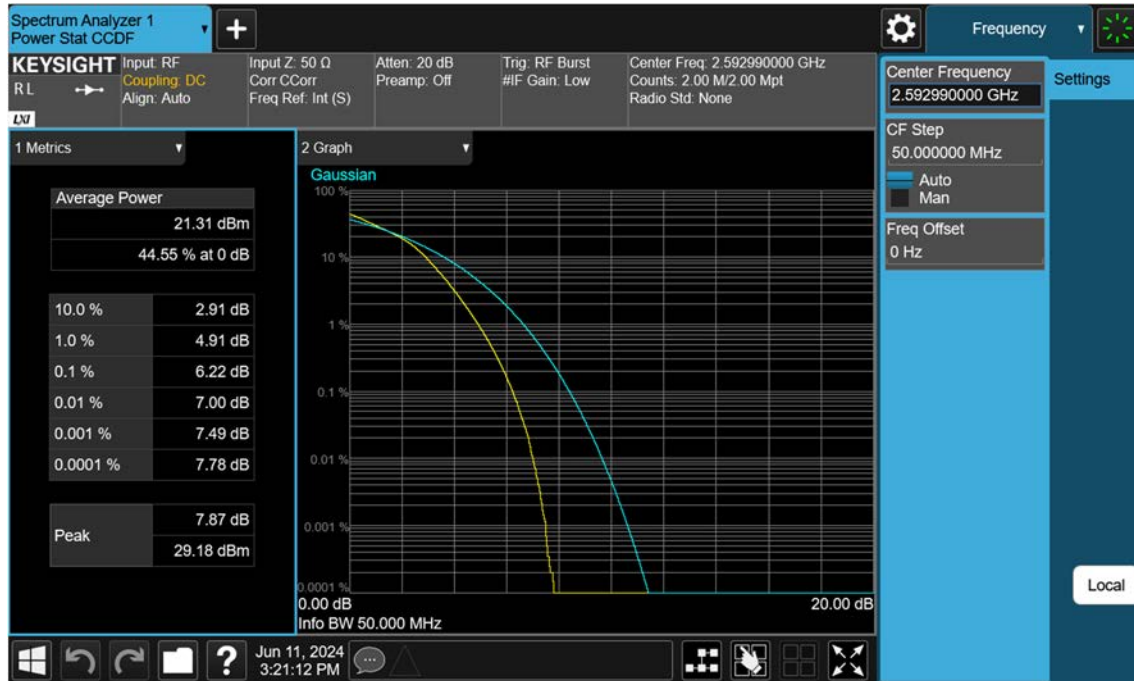
Sub6 n41_50 M_PAR_Mid_16QAM_FullRB
