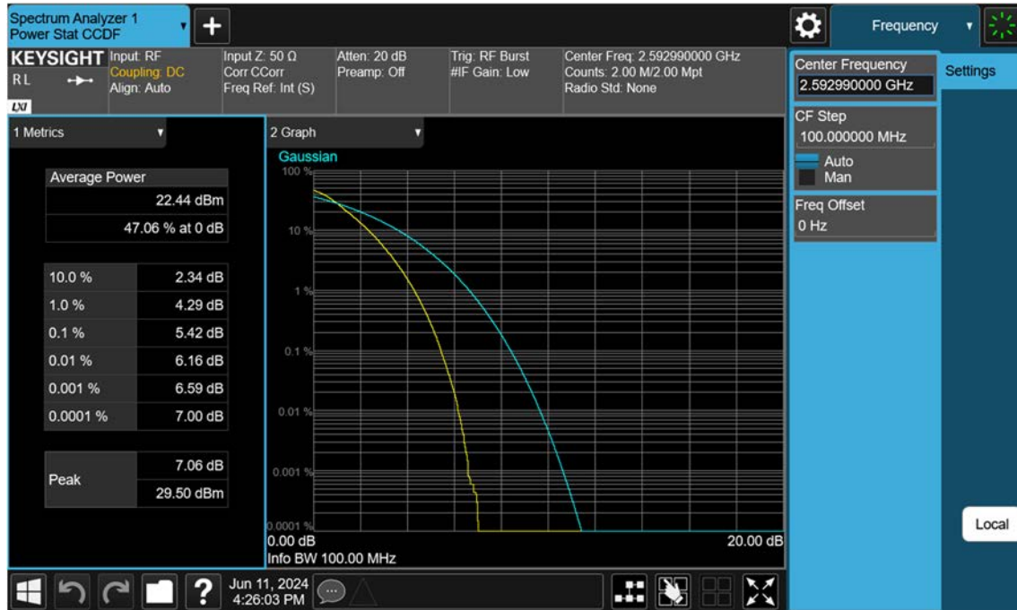
Sub6 n41_100 M_PAR_Mid_QPSK_FullRB
