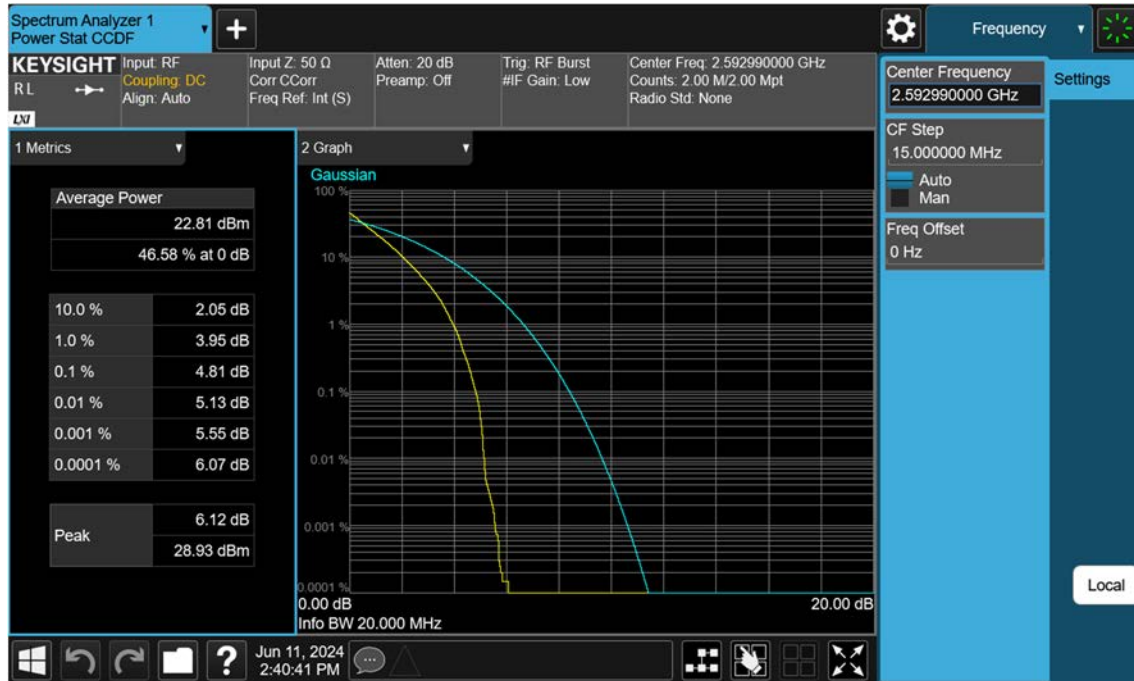
Sub6 n41_20 M_PAR_Mid_BPSK_FullRB
