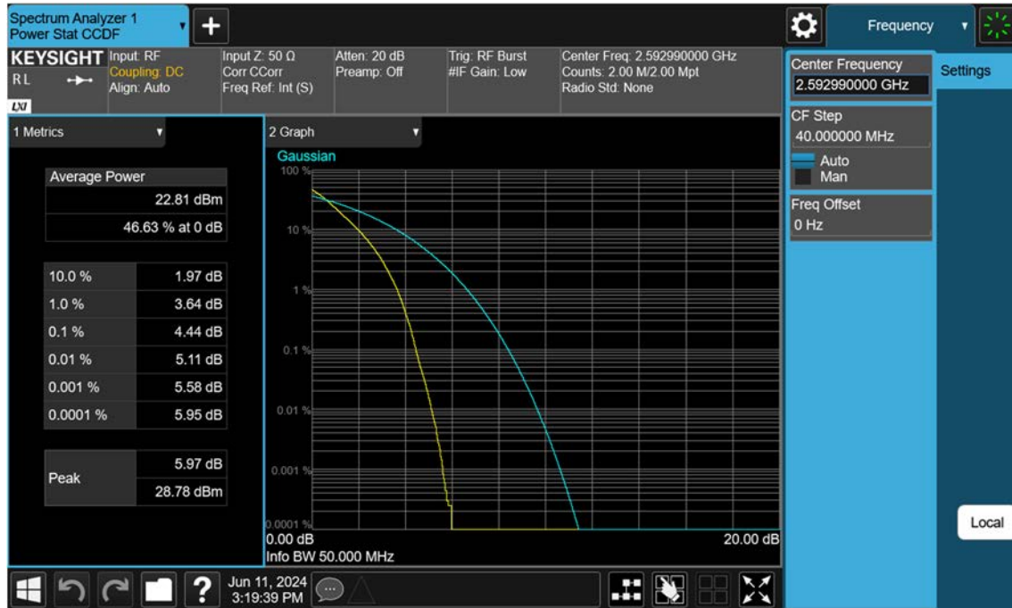
Sub6 n41_50 M_PAR_Mid_BPSK_FullRB
