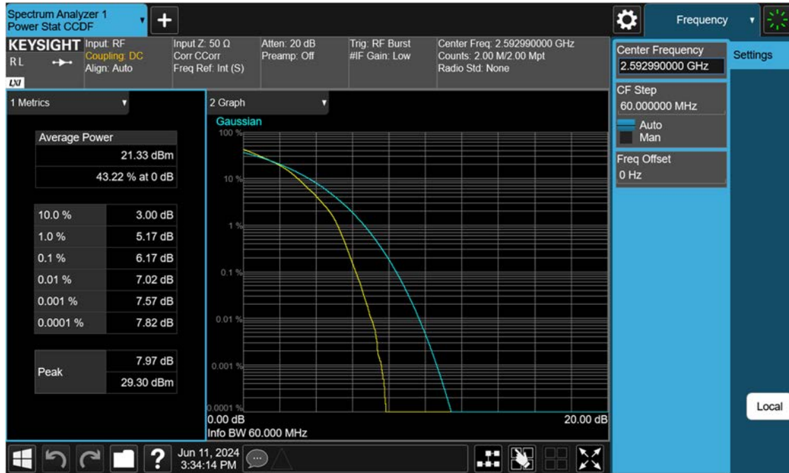
Sub6 n41_60 M_PAR_Mid_16QAM_FullRB
