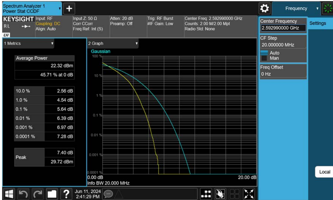
Sub6 n41_20 M_PAR_Mid_QPSK_FullRB
