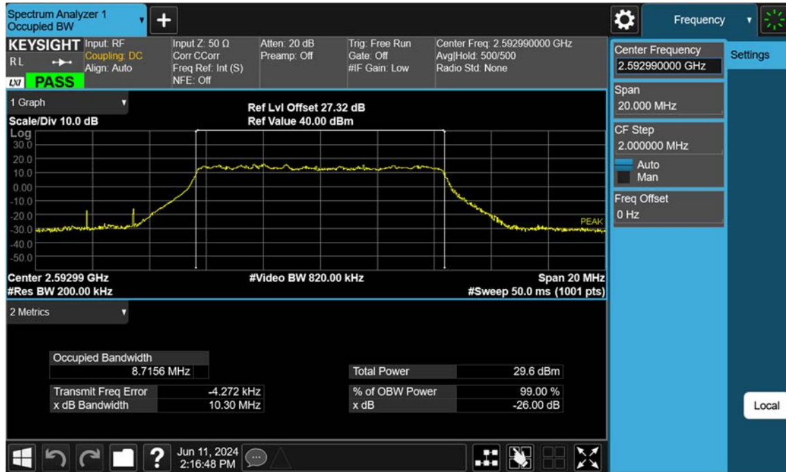
Sub6 n41_10 M_OBW_Mid_64QAM_FullRB
