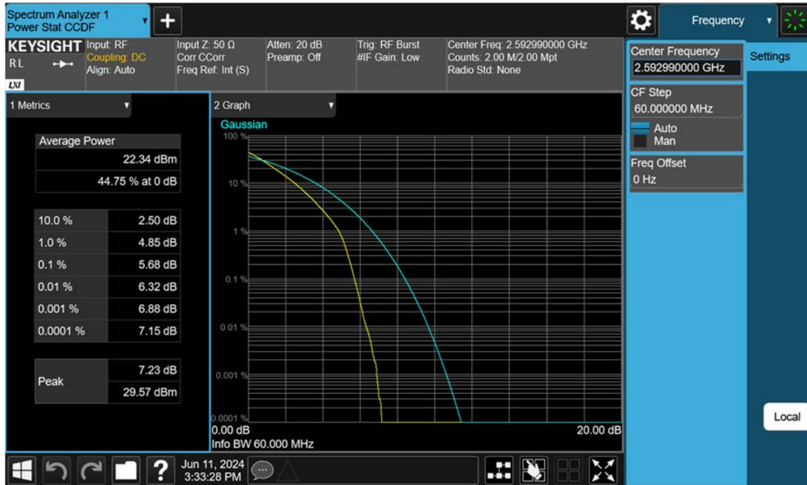
Sub6 n41_60 M_PAR_Mid_QPSK_FullRB
