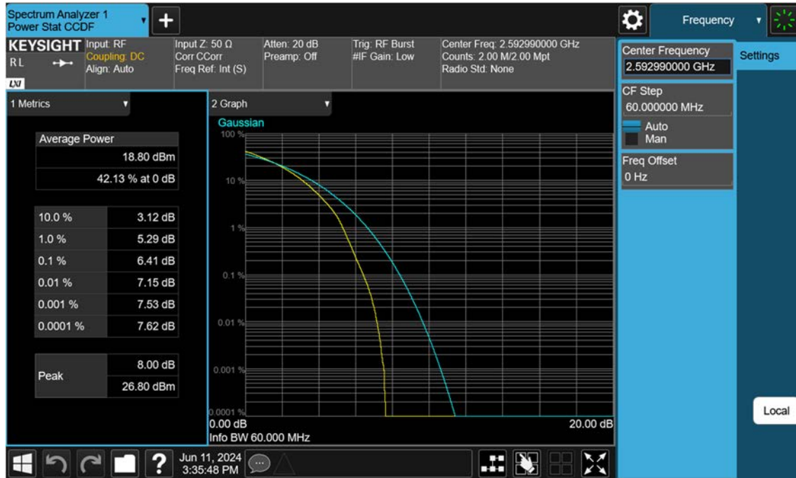
Sub6 n41_60 M_PAR_Mid_256QAM_FullRB
