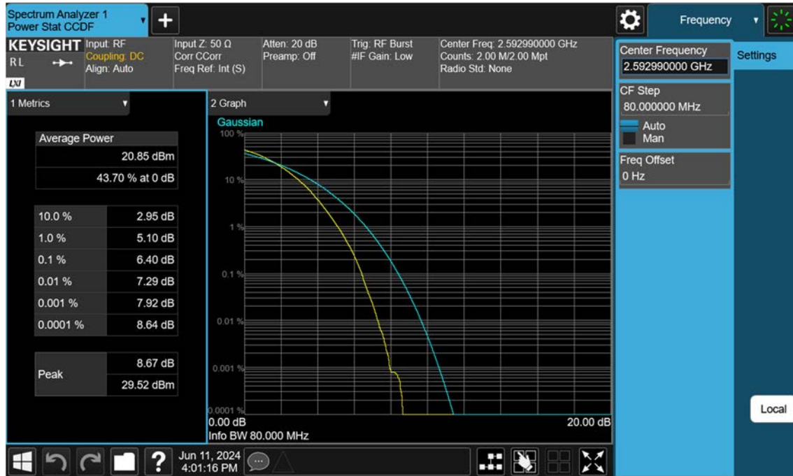
Sub6 n41_80 M_PAR_Mid_64QAM_FullRB
