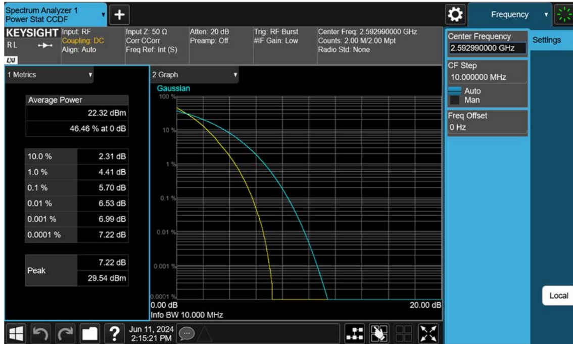
Sub6 n41_10 M_PAR_Mid_QPSK_FullRB
