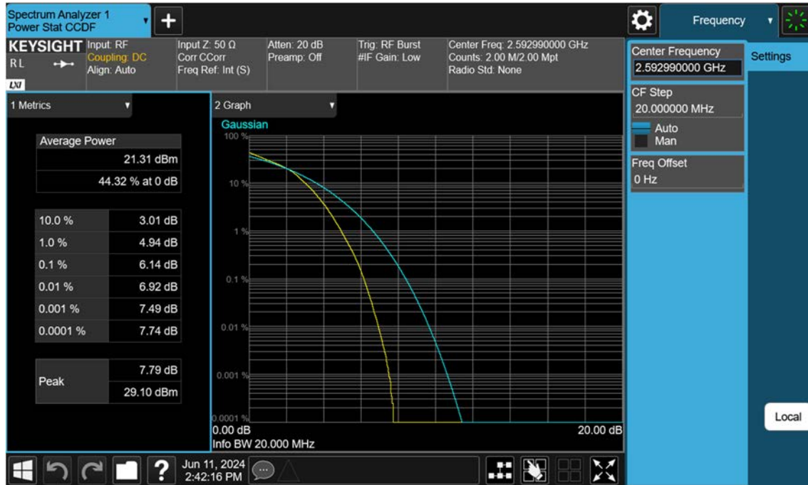
Sub6 n41_20 M_PAR_Mid_16QAM_FullRB
