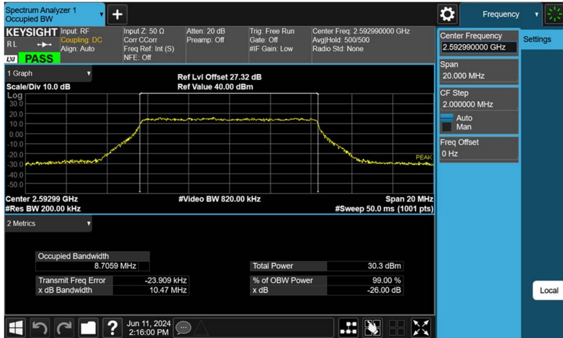
Sub6 n41_10 M_OBW_Mid_16QAM_FullRB
