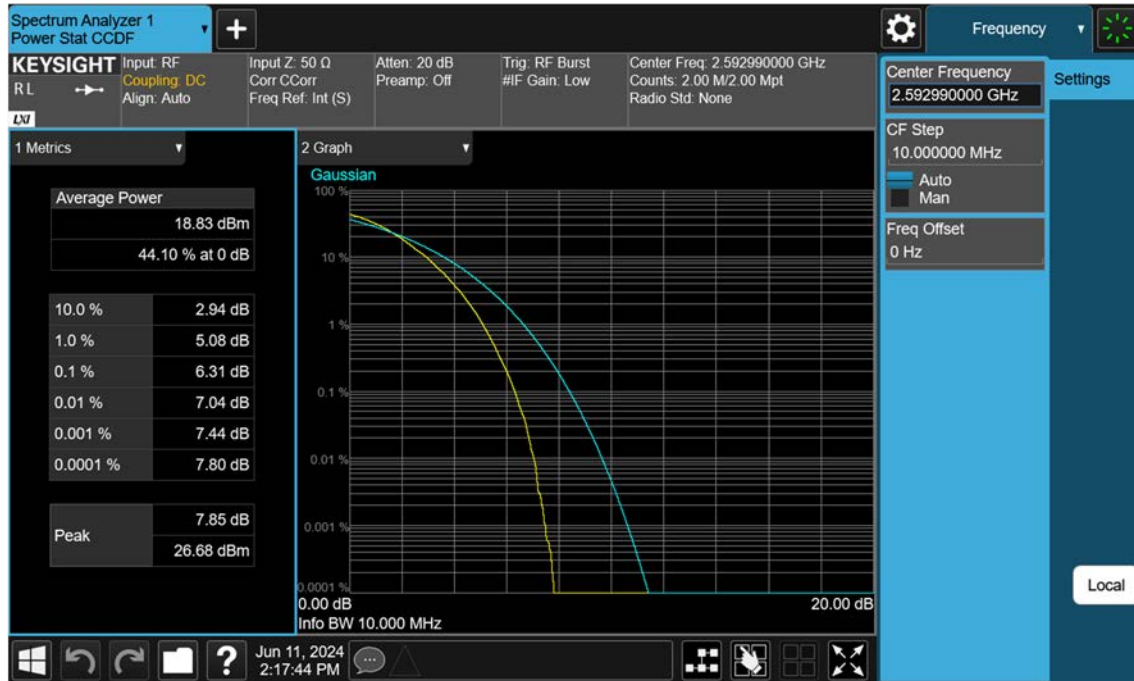
Sub6 n41_10 M_PAR_Mid_256QAM_FullRB
