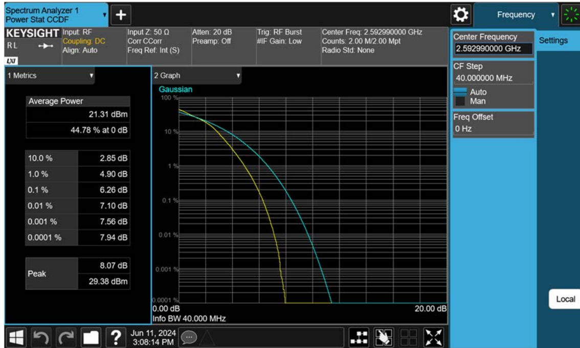
Sub6 n41_40 M_PAR_Mid_16QAM_FullRB
