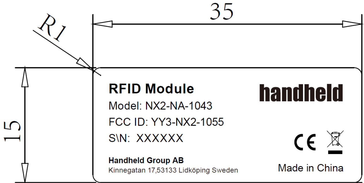
FCC ID Label
