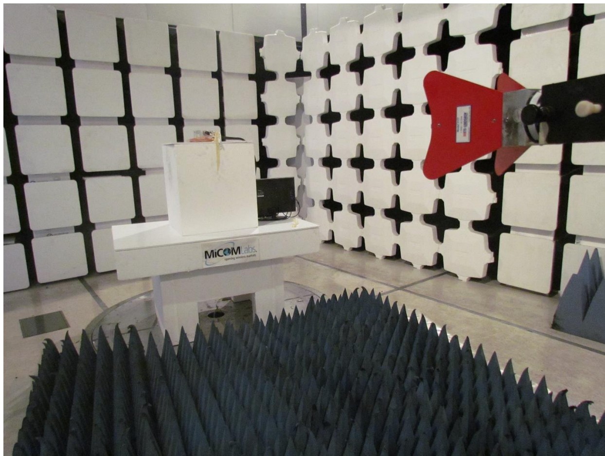
Radiated Emissions Antenna 865-5366-71S
