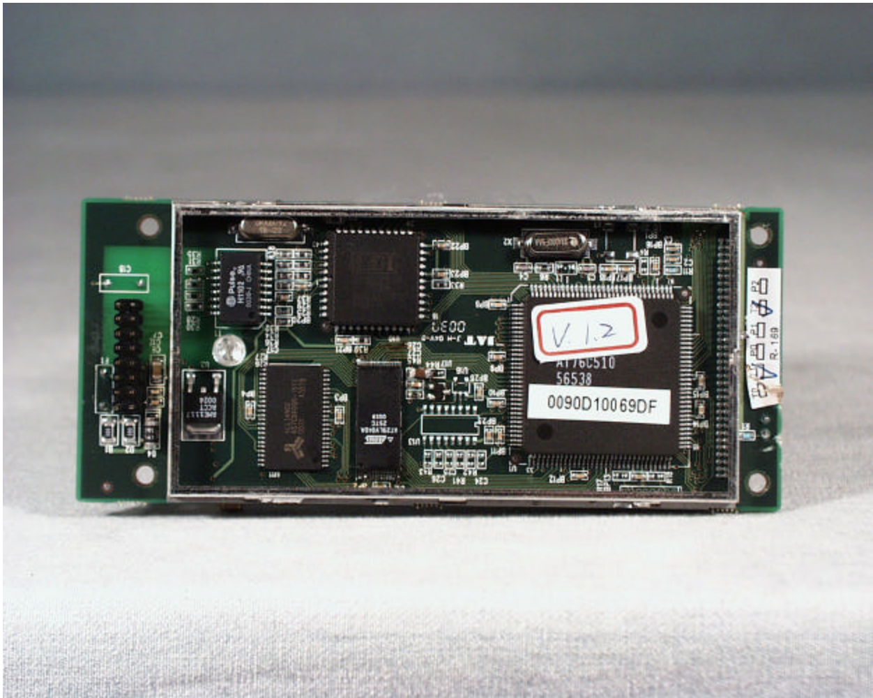
Back view of the complete RF transceiver (RF cans removed)
