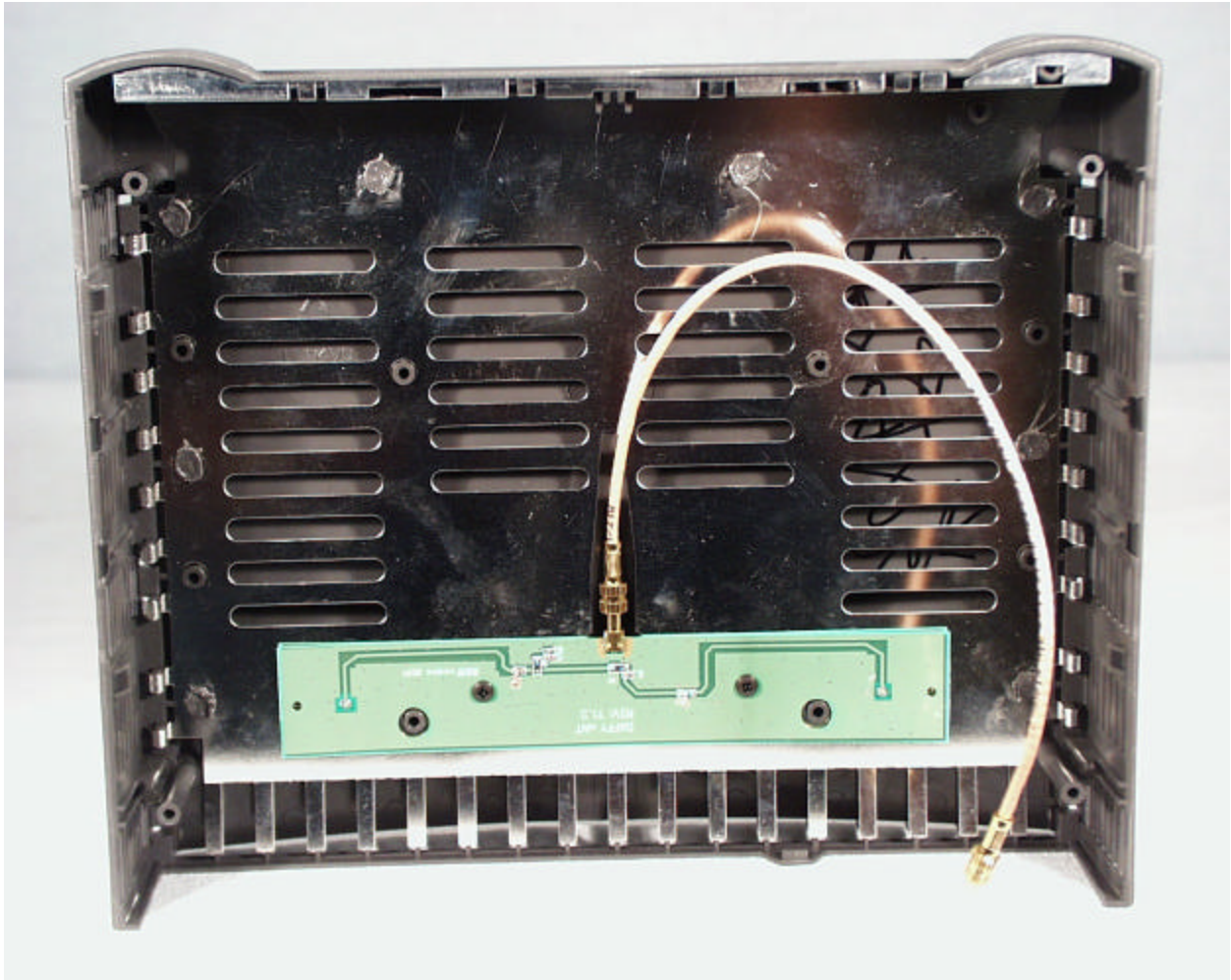
Antenna board
