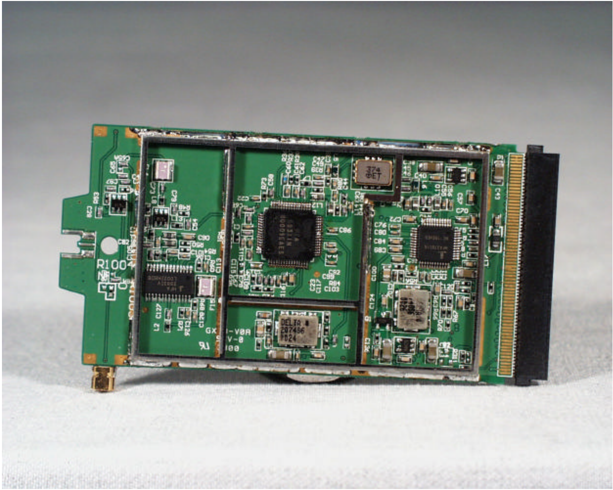
Front view of the Eumitcom PCMPIA RF transceiver (RF cans removed)
