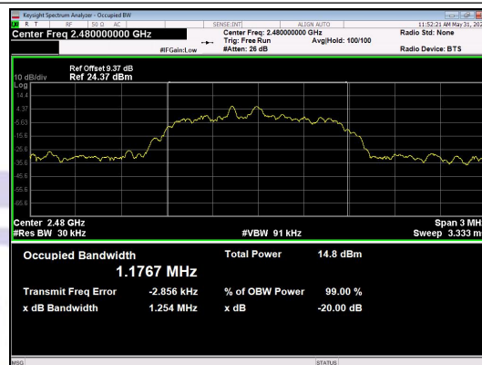
\pi/4 DQPSK_2-DH1_Channel 78
