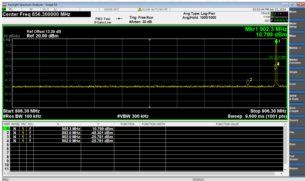
Band Edge NVNT LoRa 902.3MHz Ant1 Emission
