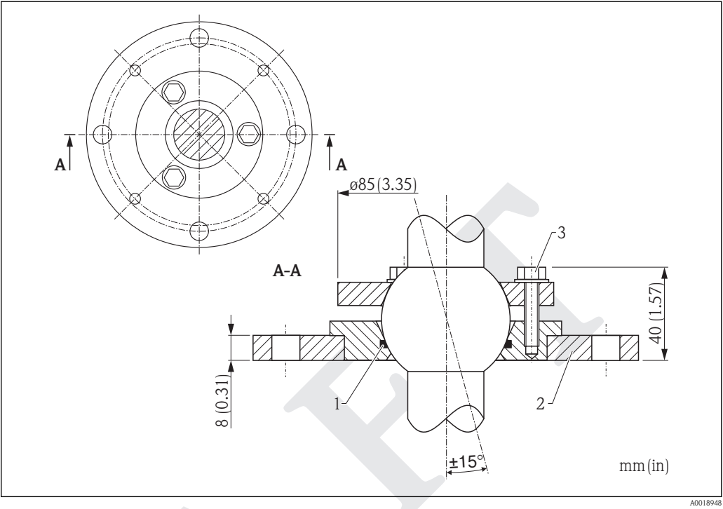
Alignment device with Endress+Hauser UNI flange
