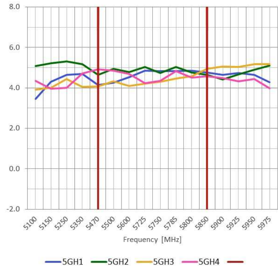
Peak Gain
