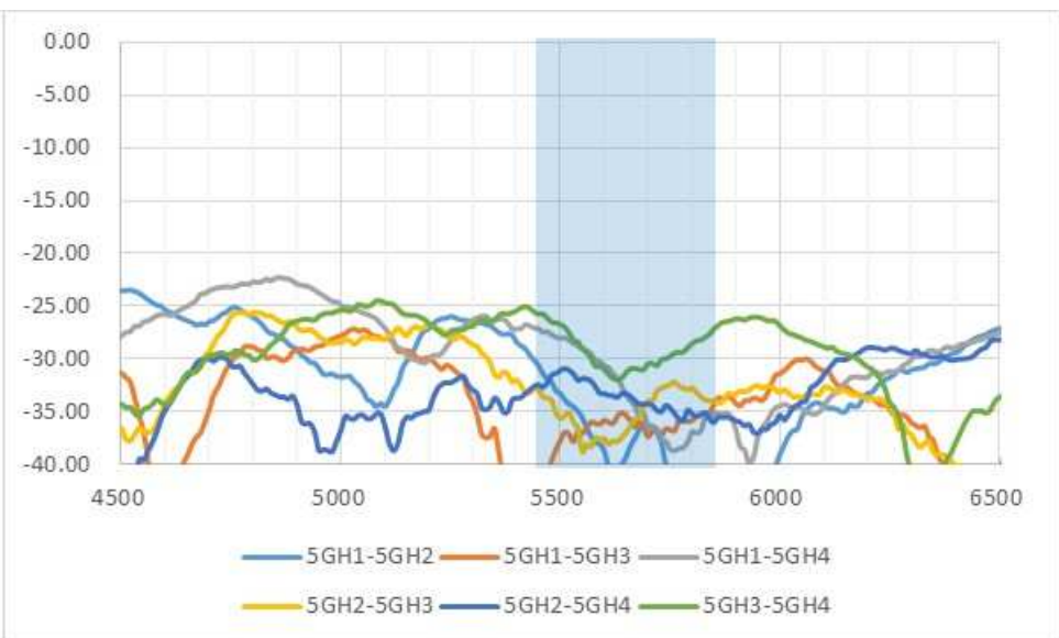
Isolation
