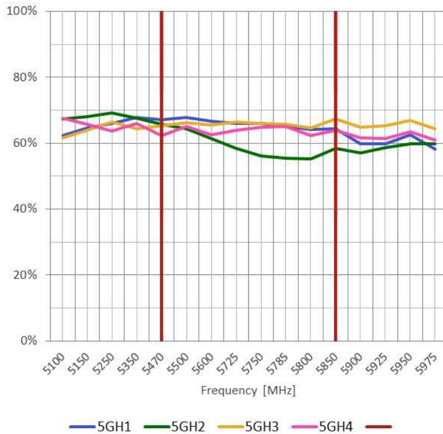
Efficiency
