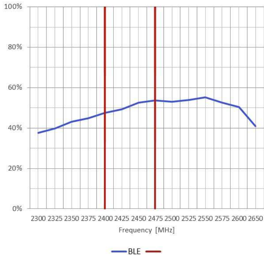
Efficiency
