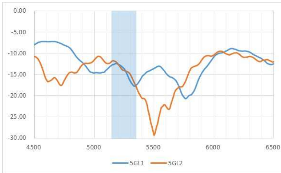
Return Loss
