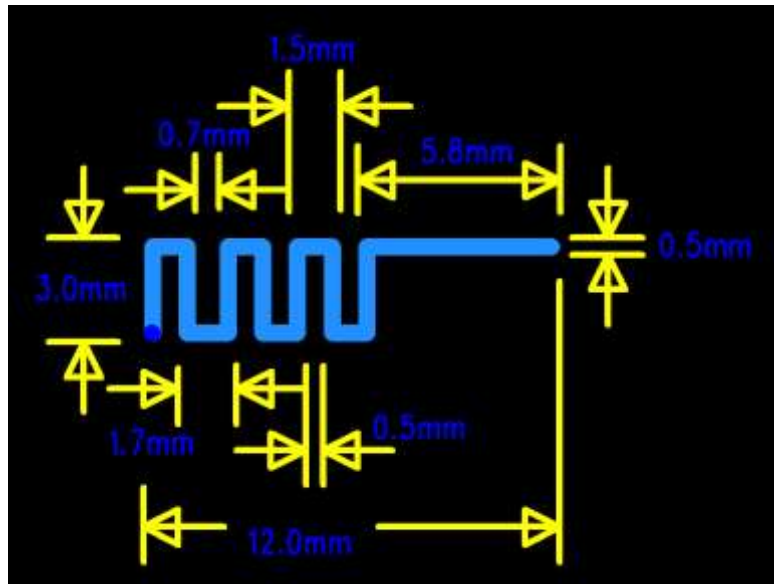
Figure 1 :Mouse Antenna size
