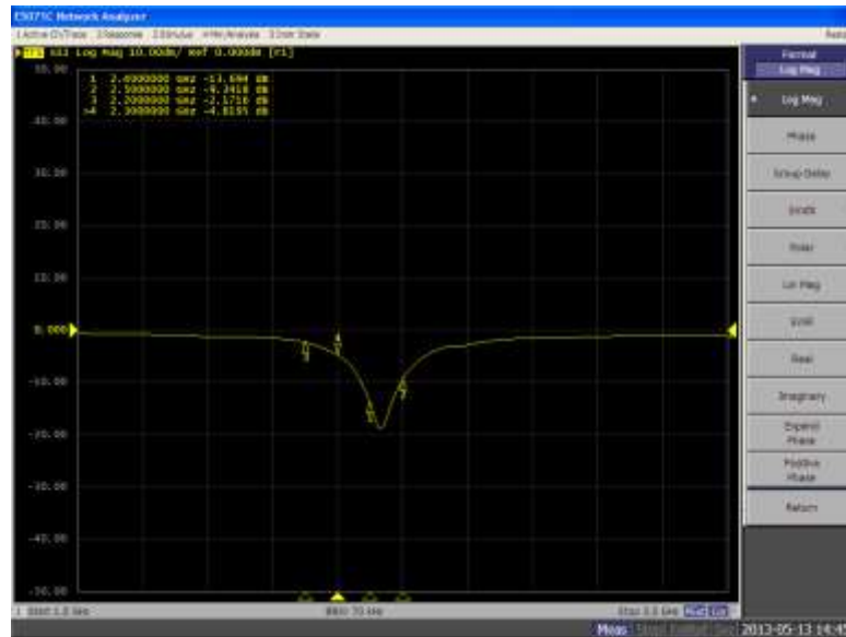
图 3 Mouse Antenna S11
