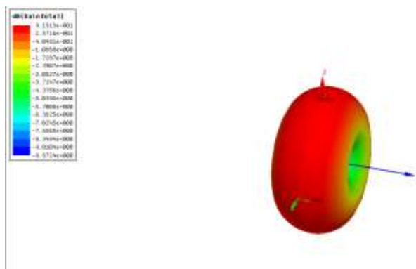
Fig.4 Mouse antenna gain and 3D direction diagram (the Y-axis is the left and right direction of figure 1, and the X-axis is the upper and lower direction of figure 1)
