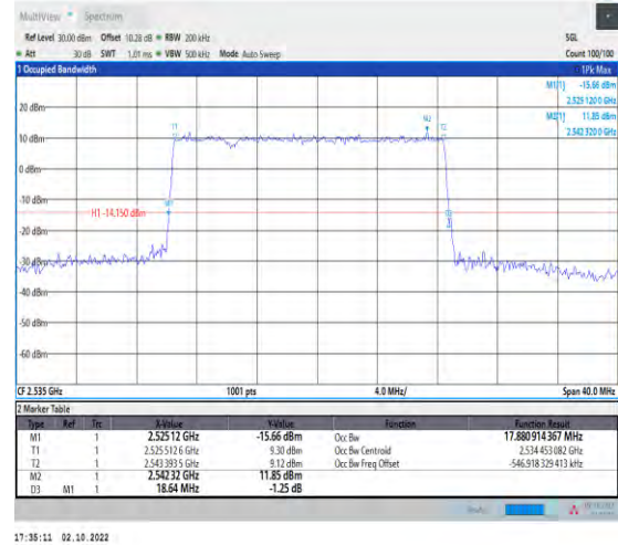
1-N7--15-20-M-4-DFT-64QAM-Outer_Full-100@0-An t1-17.881-18.640-≤20-PASS
