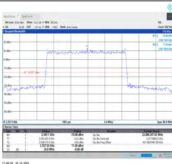
1-N7--15-25-H-5-DFT-256QAM-Outer_Full-128@0-A nt1-22.884-24.000-≤25-PASS
