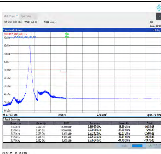
1-N7--15-5-H-2-DFT-PI2BPSK-Edge_1RB_Right-1@24-Ant1-1--PASS-see graph
