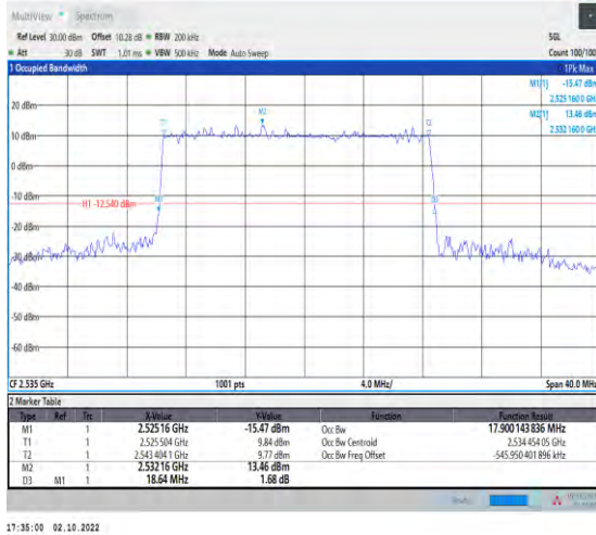
1-N7--15-20-M-3-DFT-16QAM-Outer_Full-100@0-An t1-17.9-18.640-≤20-PASS
