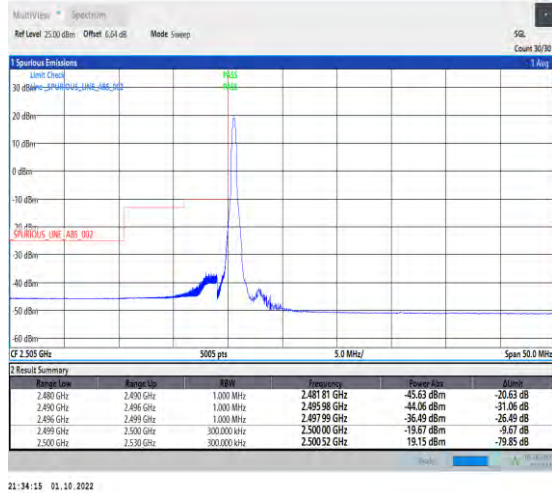
1-N7--15-20-L-1-DFT-PI2BPSK-Edge_1RB_Left-1@0-Ant1-1--PASS-see graph
