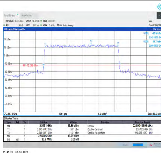
1-N7--15-25-H-6-CP-QPSK-Outer_Full-133@0-Ant1- 49.588-50.000-≤25-PASS
