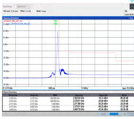
1-N7--15-30-H-5-CP-QPSK-Edge_1RB_Right-1@159-Ant1-1--PASS-see graph
