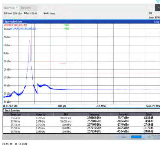
1-N7--15-5-H-5-CP-QPSK-Edge_1RB_Right-1@24-Ant1-1--PASS-see graph
