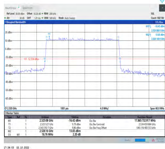
1-N7--15-20-M-6-CP-QPSK-Outer_Full-106@0-Ant1 -39.629-40.000-≤20-PASS
