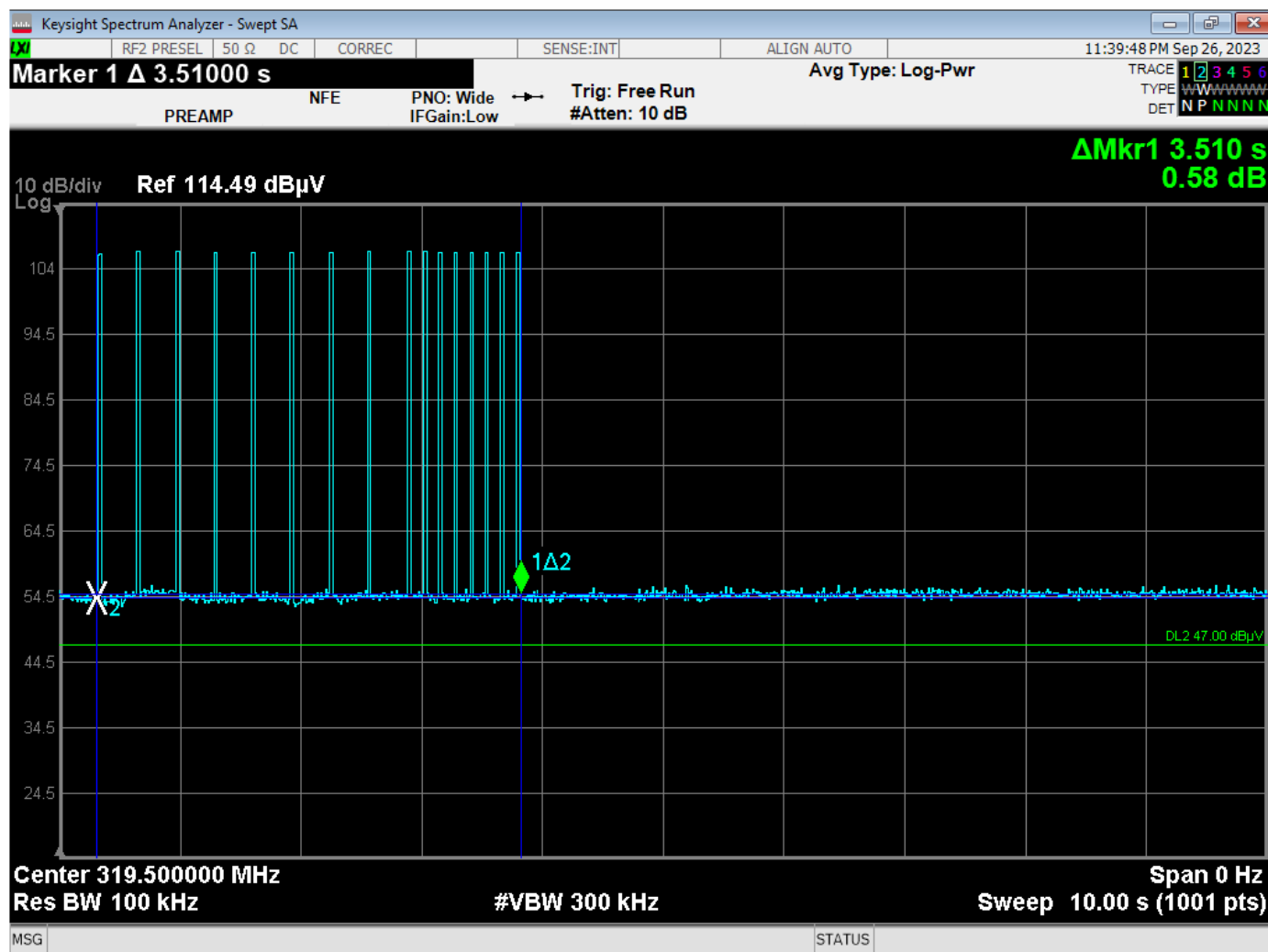
Plot Showing Time of Full Transmission – 3.51 Seconds
