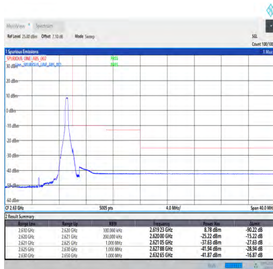
1-N38-30-10-H-5-CP-QPSK-Edge_1RB_Right-1@23-Ant1-1--PASS-see graph
