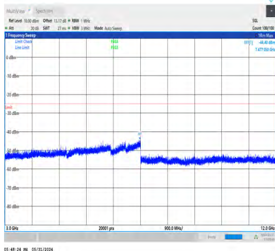
1-N38-30-40-H-1-DFT-PI2BPSK-Inner_1RB_Left-1 @1-3000-12000-Ant1-7477.05--44.40--25-PASS
