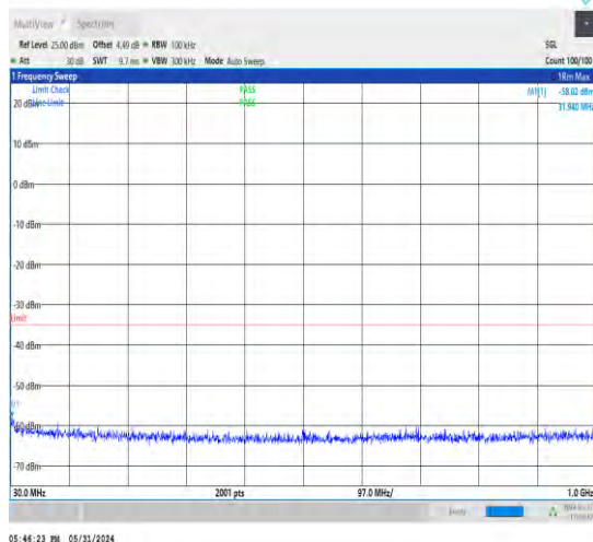
1-N38-30-40-M-1-DFT-PI2BPSK-Inner_1RB_Left-1 @1-30-1000-Ant1-33.88--58.02--35-PASS
