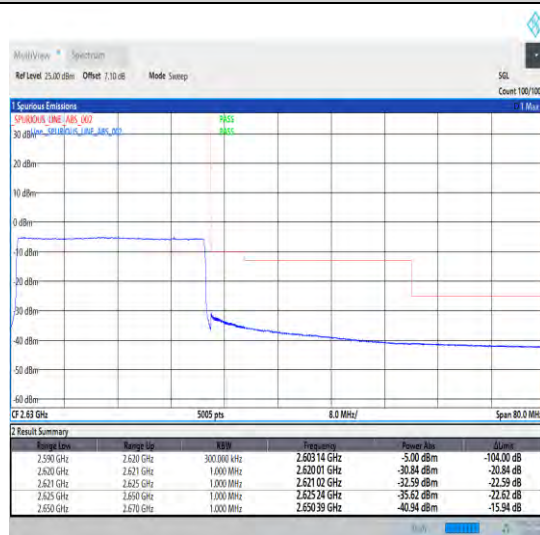
1-N38-30-30-H-6-CP-QPSK-Outer_Full-78@0-Ant1-1--PASS-see graph
