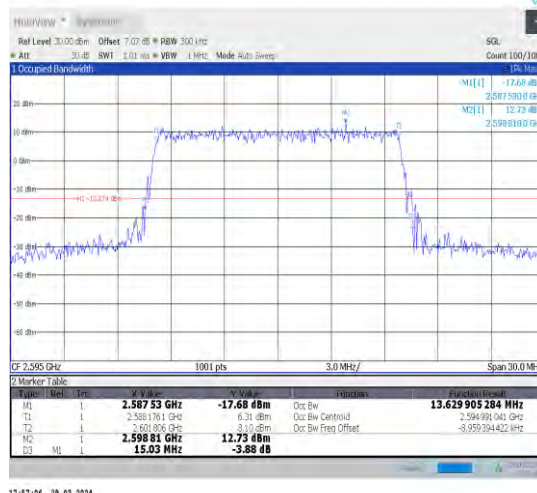
1-N38-30-15-M-9-CP-256QAM-Outer_Full-38@0-Ant1 1-13.63-15.030-≤15-PASS
