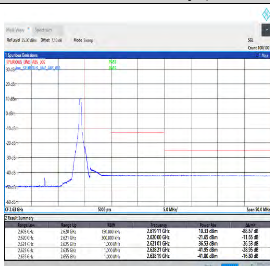
1-N38-30-15-H-5-CP-QPSK-Edge_1RB_Right-1@37-Ant1-1--PASS-see graph
