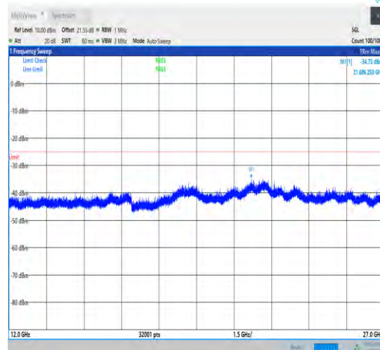
1-N38-30-40-M-1-DFT-PI2BPSK-Inner_1RB_Left-1@ 1-12000-27000-Ant1-21067.50--34.73--25-PASS
