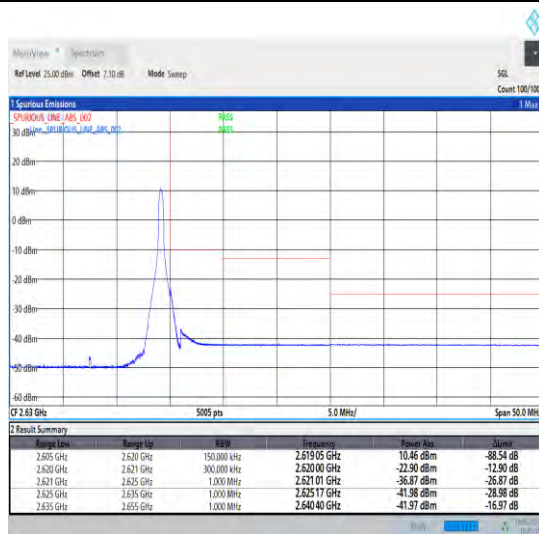
1-N38-30-15-H-2-DFT-PI2BPSK-Edge_1RB_Right-1@37-Ant1-1--PASS-see graph
