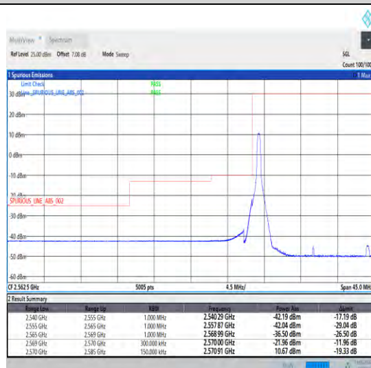
1-N38-30-15-L-6-CP-QPSK-Outer_Full-38@0-Ant1-1--PASS-see graph
