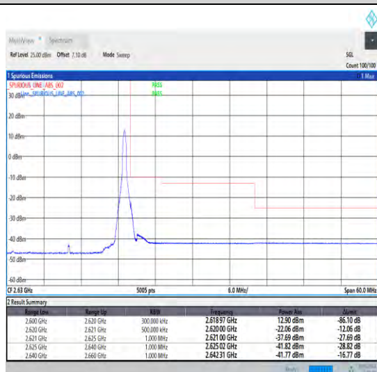
1-N38-30-20-H-5-CP-QPSK-Edge_1RB_Right-1@50-Ant1-1--PASS-see graph
