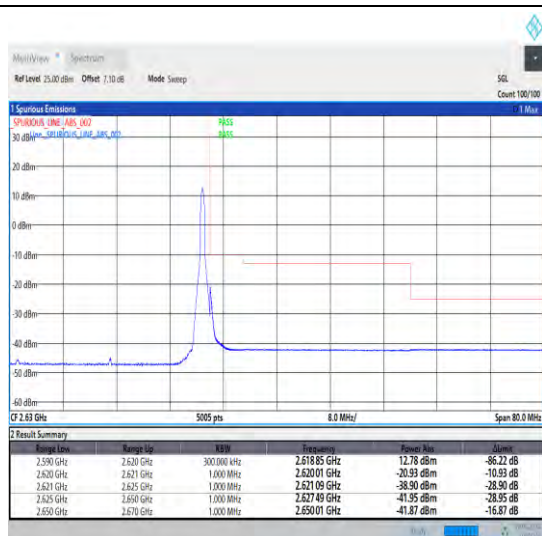
1-N38-30-30-H-2-DFT-PI2BPSK-Edge_1RB_Right-1@77-Ant1-1--PASS-see graph
