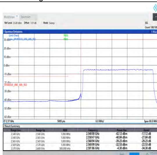
1-N38-30-30-L-3-DFT-PI2BPSK-Outer_Full-75@0-Ant1-1--PASS-see graph
