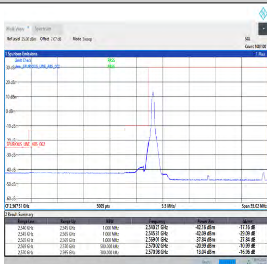
1-N38-30-25-L-4-CP-QPSK-Edge_1RB_Left-1@0-Ant1-1--PASS-see graph
