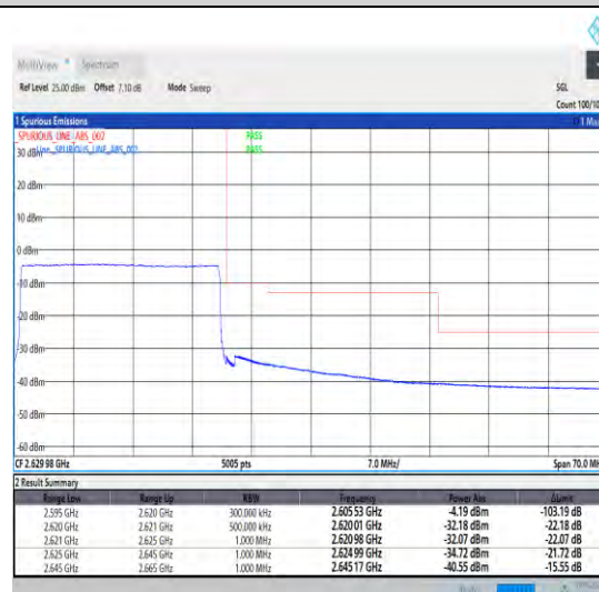
1-N38-30-25-H-6-CP-QPSK-Outer_Full-65@0-Ant1-1--PASS-see graph
