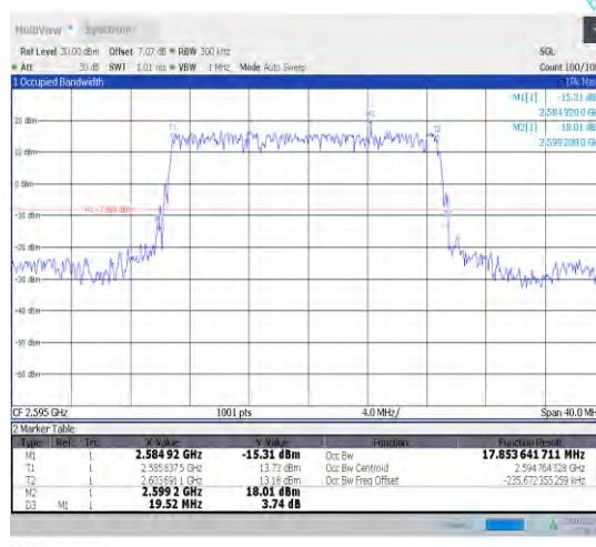
1-N38-30-20-M-2-DFT-PI2BPSK-Outer_Full-50@0-Ant1 1-17.854-19.520-≤20-PASS
