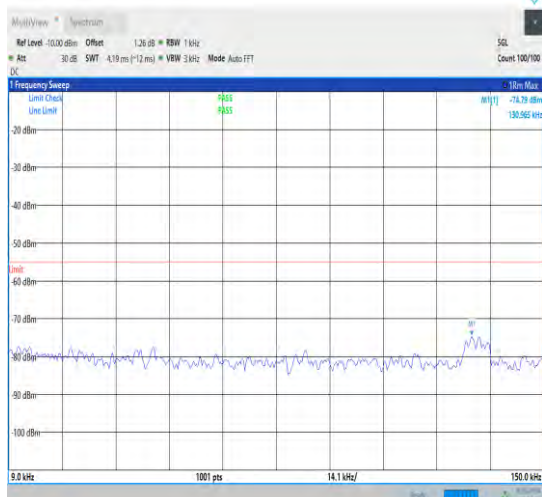
1-N38-30-40-M-1-DFT-PI2BPSK-Inner_1RB_Left-1 @ 1-0.009-0.15-Ant1-0.01--74.79--55-PASS
