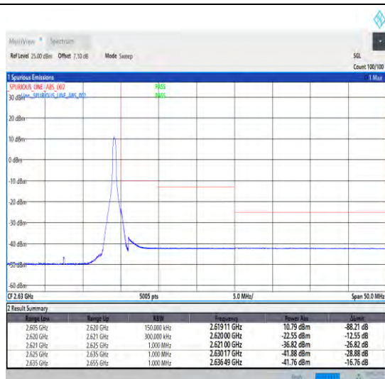
1-N38-30-15-H-2-DFT-PI2BPSK-Edge_1RB_Right-1@37-Ant1-1--PASS-see graph
