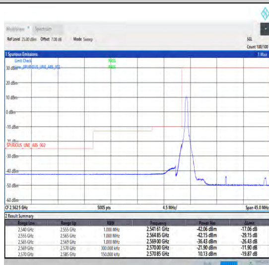
1-N38-30-15-L-4-CP-QPSK-Edge_1RB_Left-1@0-Ant1-1--PASS-see graph
