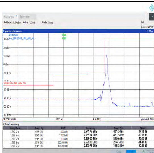
1-N38-30-15-L-1-DFT-PI2BPSK-Edge_1RB_Left-1@0-Ant1-1--PASS-see graph
