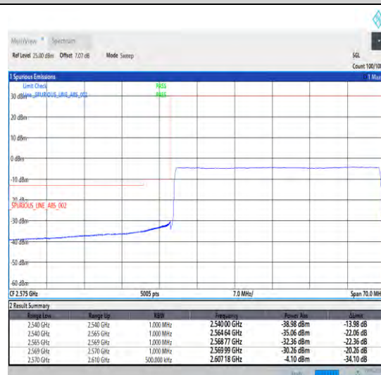
1-N38-30-40-L-6-CP-QPSK-Outer_Full-106@0-Ant1-1--PASS-see graph
