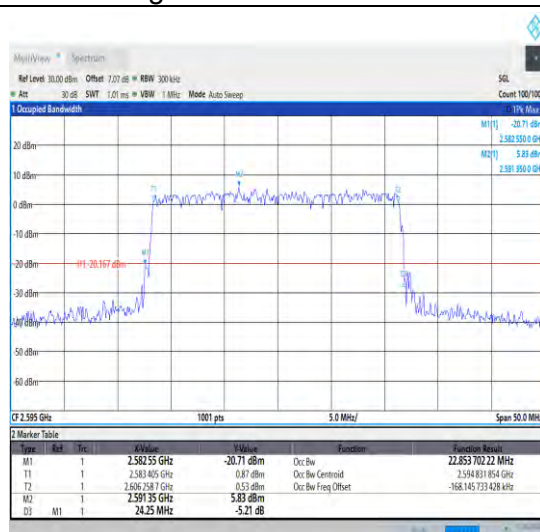
1-N38-30-25-M-3-DFT-16QAM-Outer_Full-75@0-Ant 1-26.718-28.020-≤30-PASS
