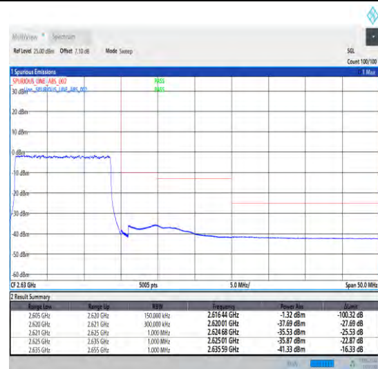
1-N38-30-15-H-3-DFT-PI2BPSK-Outer_Full-36@0-Ant1-1--PASS-see graph
