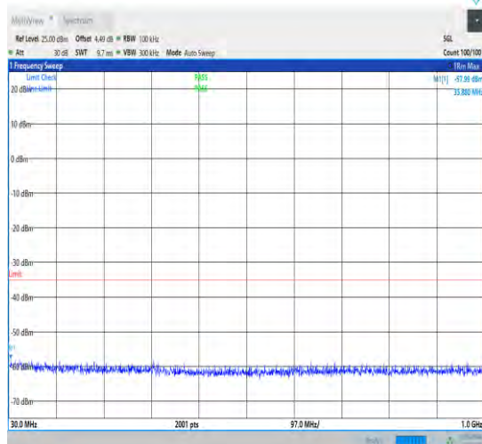
1-N38-30-40-L-1-DFT-PI2BPSK-Inner_1RB_Left-1 @1-30-1000-Ant1-33.88--57.99--35-PASS
