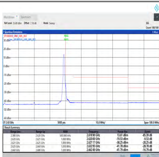
1-N38-30-40-H-5-CP-QPSK-Edge_1RB_Right-1@105-Ant1-1--PASS-see graph
