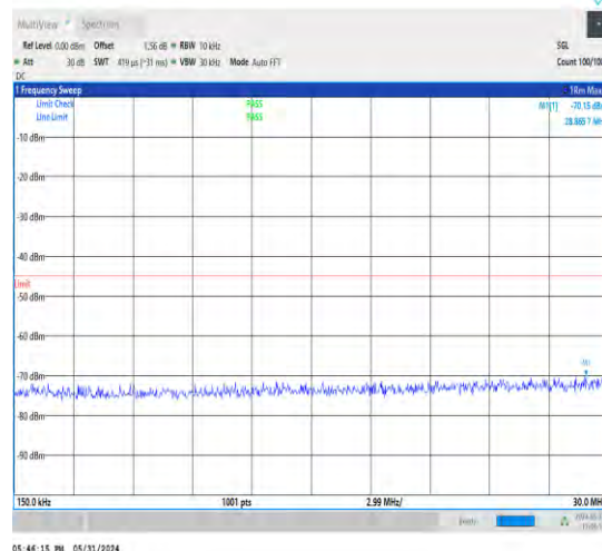
1-N38-30-40-M-1-DFT-PI2BPSK-Inner_1RB_Left-1@ 1-0.15-30-Ant1-28.39--70.15--45-PASS
