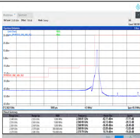
1-N38-30-15-L-4-CP-QPSK-Edge_1RB_Left-1@0-Ant1-1--PASS-see graph
