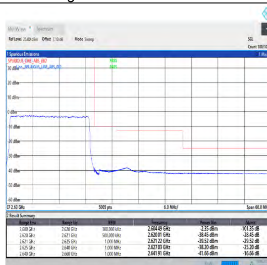
1-N38-30-20-H-3-DFT-PI2BPSK-Outer_Full-50@0-Ant1-1--PASS-see graph
