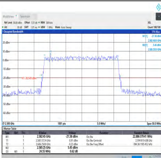
1-N38-30-25-M-4-DFT-64QAM-Outer_Full-75@0-Ant 1-26.738-28.200-≤30-PASS
