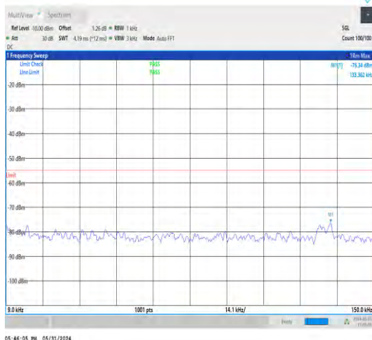
1-N38-30-40-M-1-DFT-PI2BPSK-Inner_1RB_Left-1 @ 1-0.009-0.15-Ant1-0.13--76.34--55-PASS
