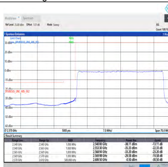
1-N38-30-40-L-3-DFT-PI2BPSK-Outer_Full-100@0-Ant1-1--PASS-see graph
