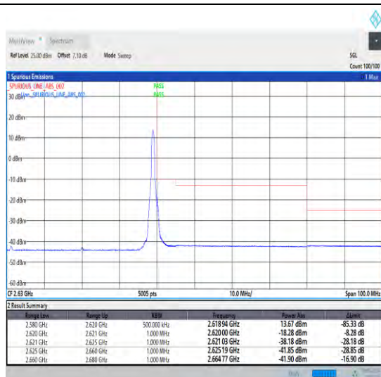
1-N38-30-40-H-2-DFT-PI2BPSK-Edge_1RB_Right-1@105-Ant1-1--PASS-see graph
