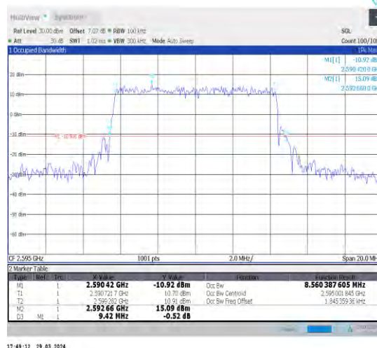
1-N38-30-10-M-2-DFT-PI2BPSK-Outer_Full-24@0-Ant1 -8.56-9.420-≤10-PASS
