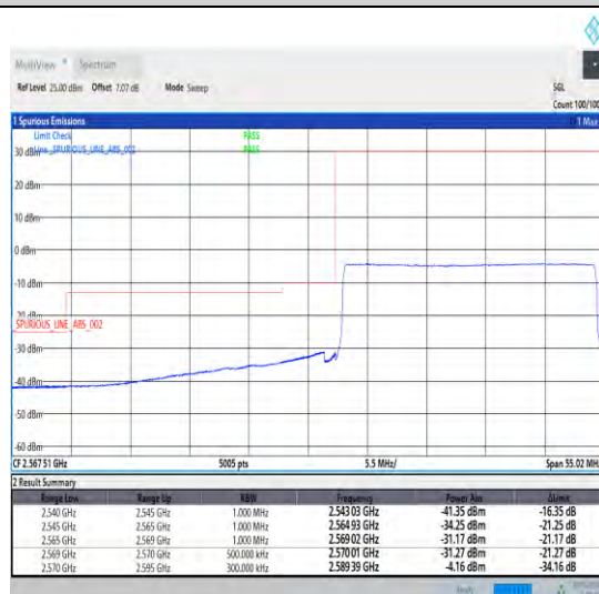
1-N38-30-25-L-6-CP-QPSK-Outer_Full-65@0-Ant1-1--PASS-see graph
