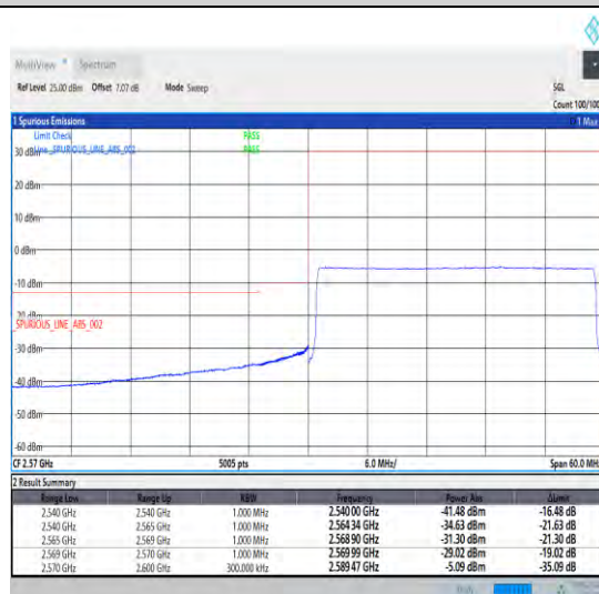
1-N38-30-30-L-6-CP-QPSK-Outer_Full-78@0-Ant1-1--PASS-see graph
