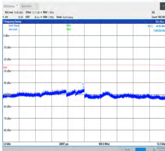
1-N38-30-40-L-1-DFT-PI2BPSK-Inner_1RB_Left-1 @ 1-3000-12000-Ant1-7445.55--44.56--25-PASS
