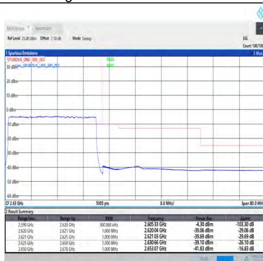
1-N38-30-30-H-3-DFT-PI2BPSK-Outer_Full-75@0-Ant1-1--PASS-see graph
