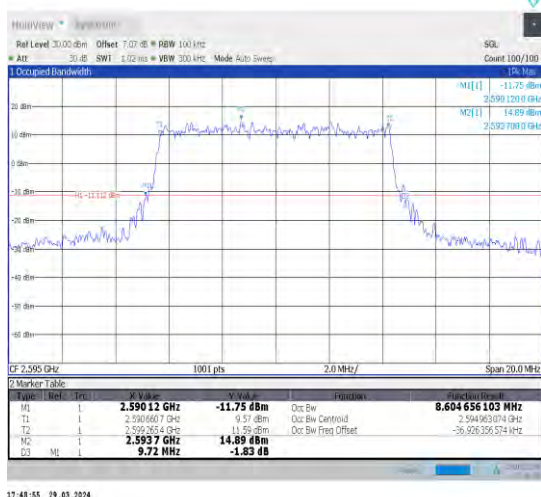
1-N38-30-10-M-1-DFT-QPSK-Outer_Full-24@0-Ant1 -8.605-9.720-≤10-PASS
