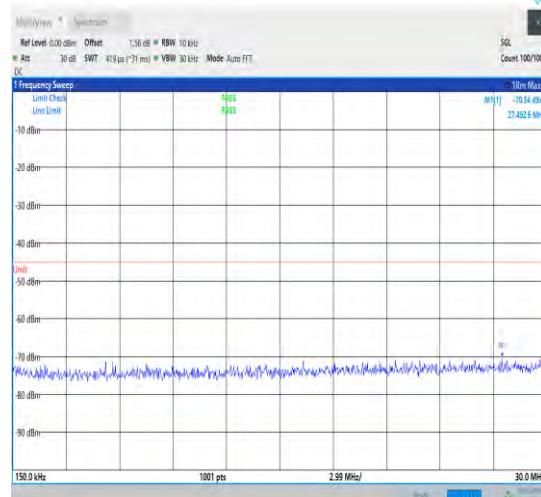
1-N38-30-40-M-1-DFT-PI2BPSK-Inner_1RB_Left-1@ 1-0.15-30-Ant1-21.79--70.54--45-PASS
