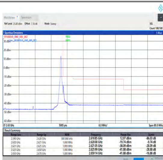
1-N38-30-30-H-5-CP-QPSK-Edge_1RB_Right-1@77-Ant1-1--PASS-see graph
