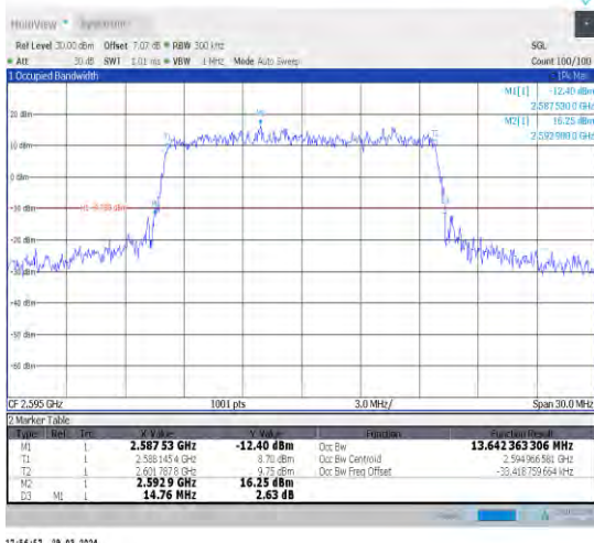
1-N38-30-15-M-8-CP-64QAM-Outer_Full-38@0-Ant1 -13.642-14.760-≤15-PASS
