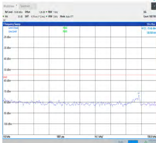
1-N38-30-40-L-1-DFT-PI2BPSK-Inner_1RB_Left-1 @1-0.009-0.15-Ant1-0.13--75.48--55-PASS
