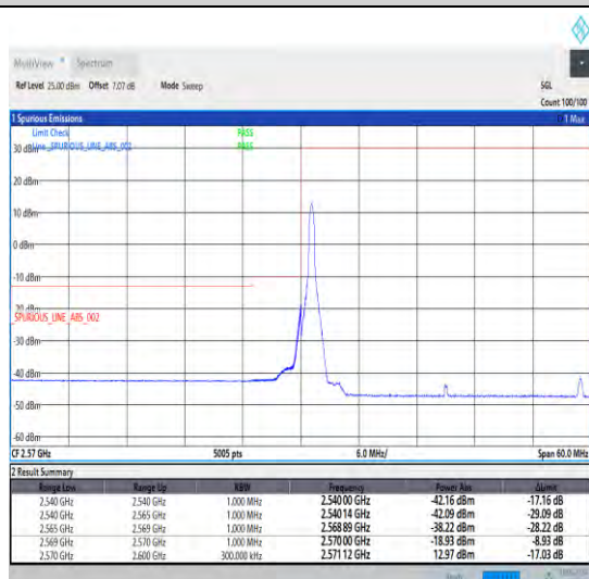
1-N38-30-30-L-4-CP-QPSK-Edge_1RB_Left-1@0-Ant1-1--PASS-see graph
