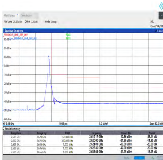
1-N38-30-15-H-5-CP-QPSK-Edge_1RB_Right-1@37-Ant1-1--PASS-see graph
