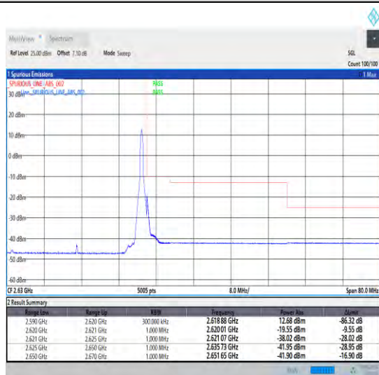
1-N38-30-30-H-5-CP-QPSK-Edge_1RB_Right-1@77-Ant1-1--PASS-see graph
