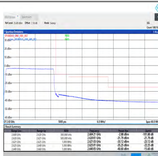
1-N38-30-20-H-6-CP-QPSK-Outer_Full-51@0-Ant1-1--PASS-see graph
