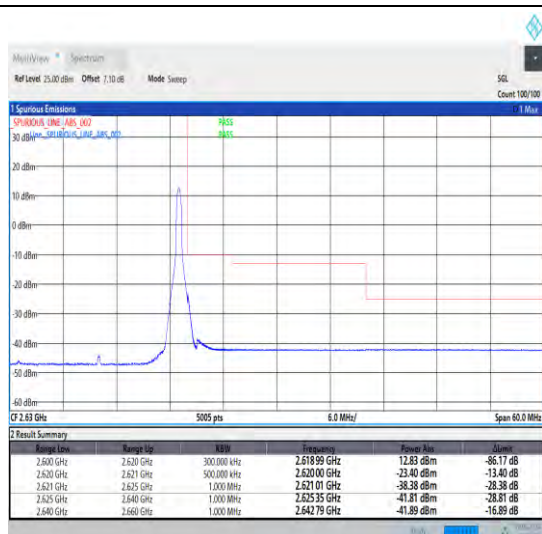
1-N38-30-20-H-2-DFT-PI2BPSK-Edge_1RB_Right-1@50-Ant1-1--PASS-see graph
