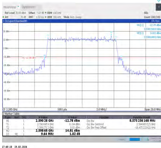
1-N38-30-10-M-3-DFT-16QAM-Outer_Full-24@0-Ant 1-8.575-9.640-≤10-PASS
