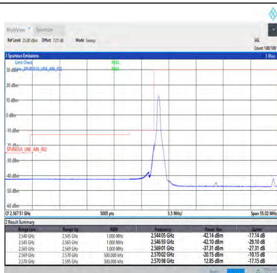
1-N38-30-25-L-1-DFT-PI2BPSK-Edge_1RB_Left-1@0-Ant1-1--PASS-see graph
