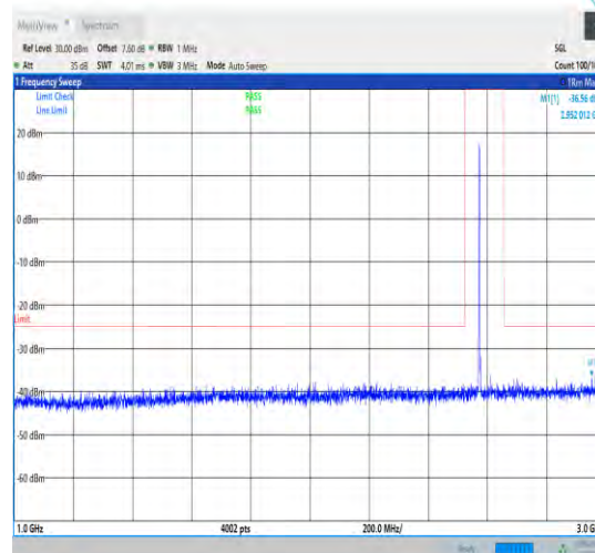
1-N38-30-40-L-1-DFT-PI2BPSK-Inner_1RB_Left-1@ 1-1000-3000-Ant1-2952.01--36.56--25-PASS
