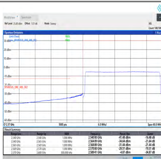
1-N38-30-30-L-6-CP-QPSK-Outer_Full-78@0-Ant1-1--PASS-see graph
