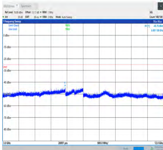
1-N38-30-40-H-1-DFT-PI2BPSK-Inner_1RB_Left-1 @1-3000-12000-Ant1-3517.50--43.70--25-PASS
