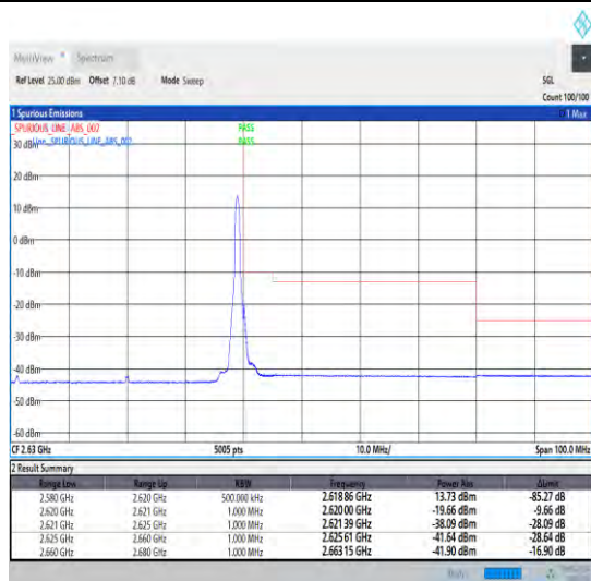
1-N38-30-40-H-5-CP-QPSK-Edge_1RB_Right-1@105-Ant1-1--PASS-see graph
