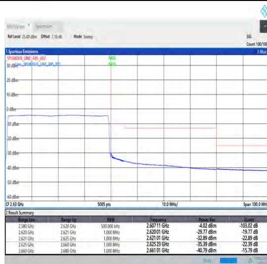
1-N38-30-40-H-6-CP-QPSK-Outer_Full-106@0-Ant1-1--PASS-see graph
