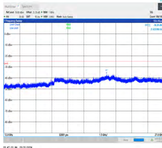
1-N38-30-40-M-1-DFT-PI2BPSK-Inner_1RB_Left-1@ 1-12000-27000-Ant1-22168.59--36.39--25-PASS
