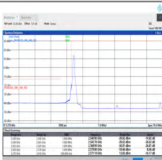
1-N38-30-40-L-4-CP-QPSK-Edge_1RB_Left-1@0-Ant1-1--PASS-see graph
