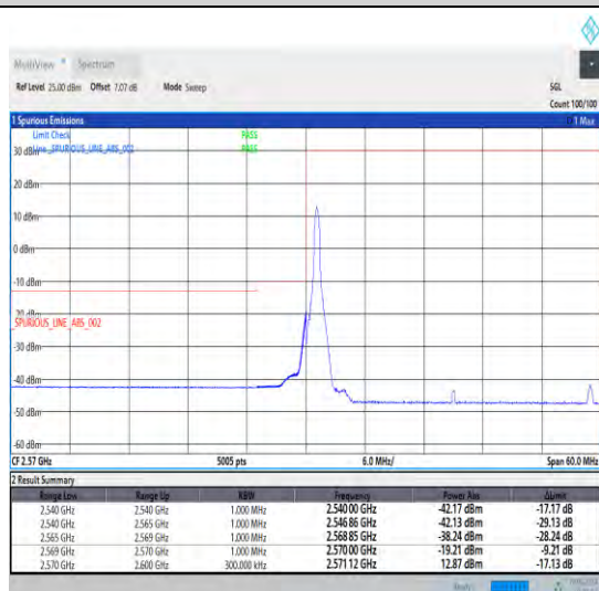
1-N38-30-30-L-4-CP-QPSK-Edge_1RB_Left-1@0-Ant1-1--PASS-see graph
