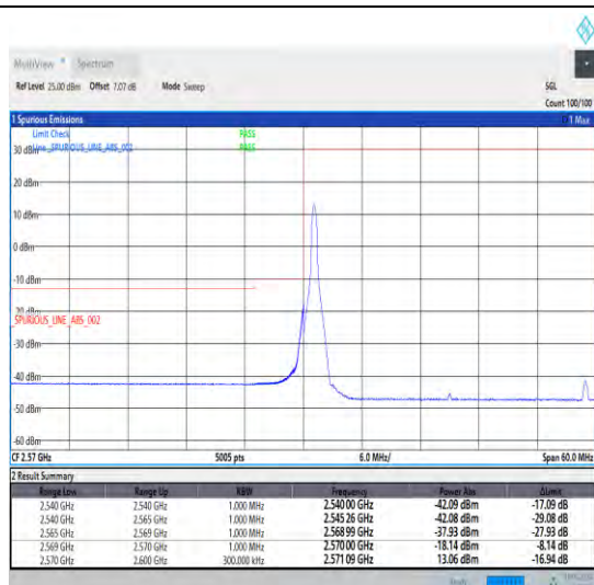
1-N38-30-30-L-1-DFT-PI2BPSK-Edge_1RB_Left-1@0-Ant1-1--PASS-see graph
