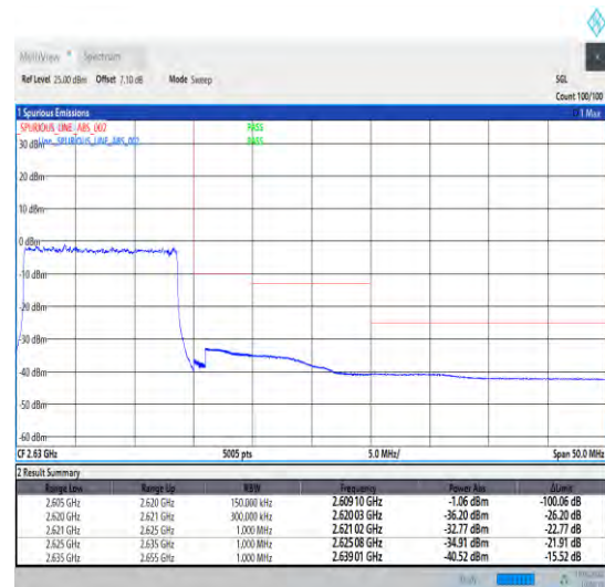
1-N38-30-15-H-6-CP-QPSK-Outer_Full-38@0-Ant1-1--PASS-see graph
