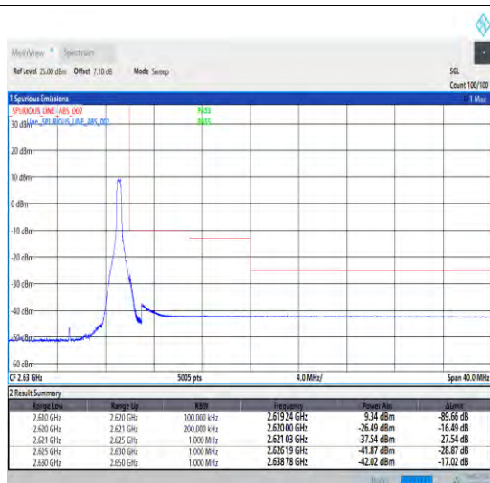
1-N38-30-10-H-2-DFT-PI2BPSK-Edge_1RB_Right-1@23-Ant1-1--PASS-see graph
