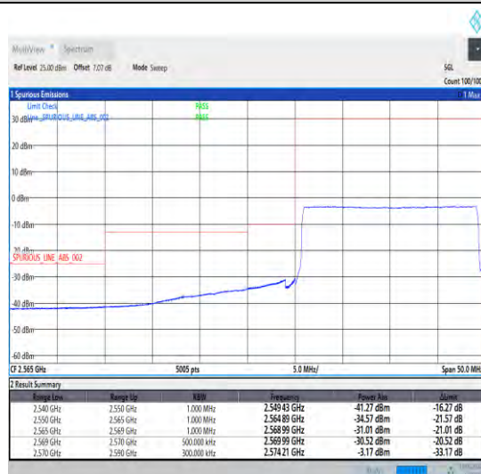
1-N38-30-20-L-6-CP-QPSK-Outer_Full-51@0-Ant1-1--PASS-see graph
