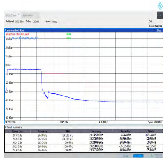
1-N38-30-10-H-6-CP-QPSK-Outer_Full-24@0-Ant1-1--PASS-see graph
