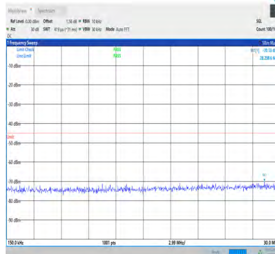
1-N38-30-40-L-1-DFT-PI2BPSK-Inner_1RB_Left-1@ 1-0.15-30-Ant1-28.30--70.13--45-PASS
