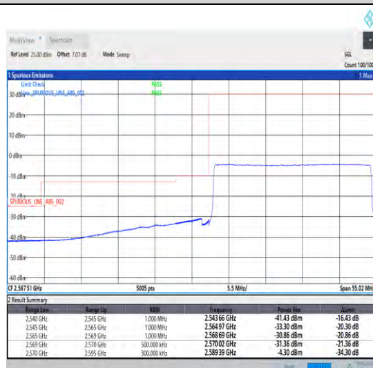
1-N38-30-25-L-6-CP-QPSK-Outer_Full-65@0-Ant1-1--PASS-see graph
