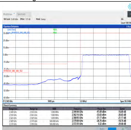
1-N38-30-20-L-3-DFT-PI2BPSK-Outer_Full-50@0-Ant1-1--PASS-see graph
