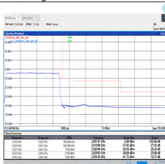
1-N38-30-25-H-3-DFT-PI2BPSK-Outer_Full-64@0-Ant1-1--PASS-see graph
