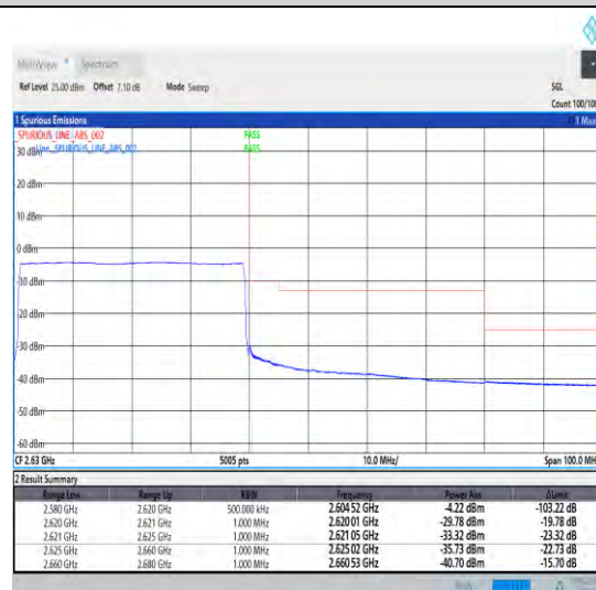
1-N38-30-40-H-6-CP-QPSK-Outer_Full-106@0-Ant1-1--PASS-see graph
