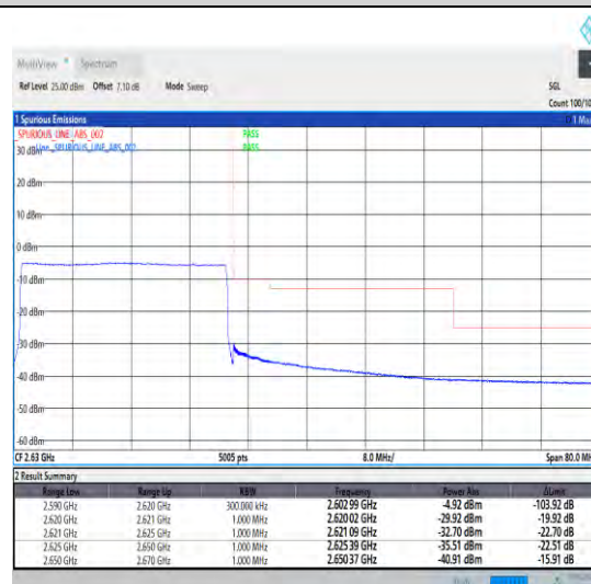
1-N38-30-30-H-6-CP-QPSK-Outer_Full-78@0-Ant1-1--PASS-see graph
