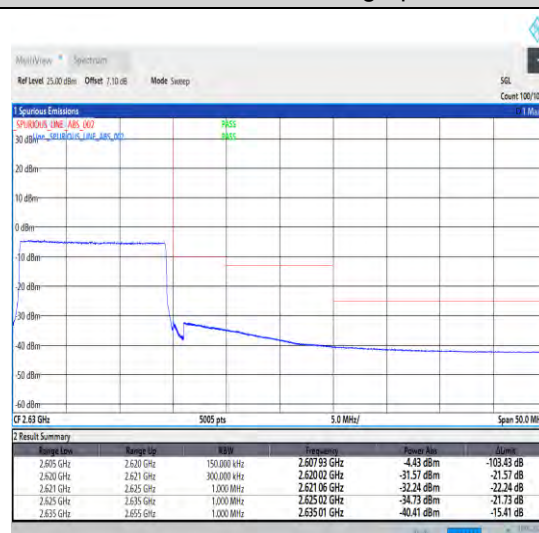
1-N38-30-15-H-6-CP-QPSK-Outer_Full-38@0-Ant1-1--PASS-see graph
