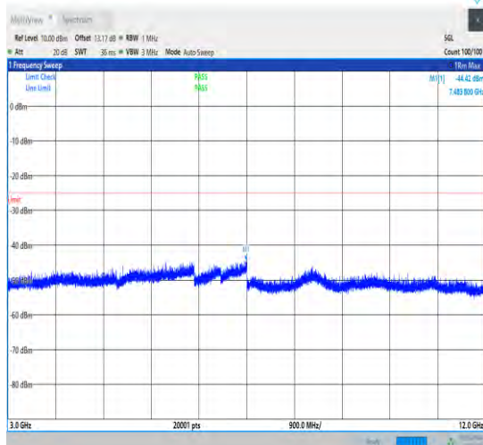
1-N38-30-40-M-1-DFT-PI2BPSK-Inner_1RB_Left-1 @1-3000-12000-Ant1-3629.55--44.42--25-PASS
