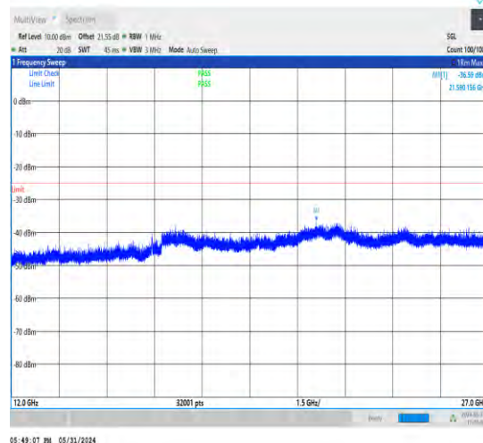
1-N38-30-40-H-1-DFT-PI2BPSK-Inner_1RB_Left-1@ 1-12000-27000-Ant1-21590.16--36.59--25-PASS
