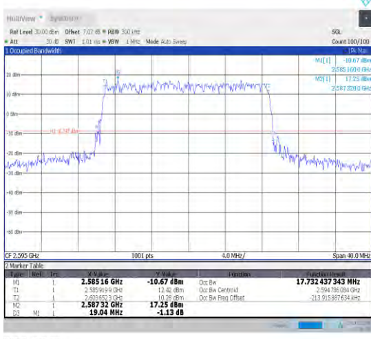
1-N38-30-20-M-1-DFT-QPSK-Outer_Full-50@0-Ant1 -17.732-19.040-≤20-PASS
