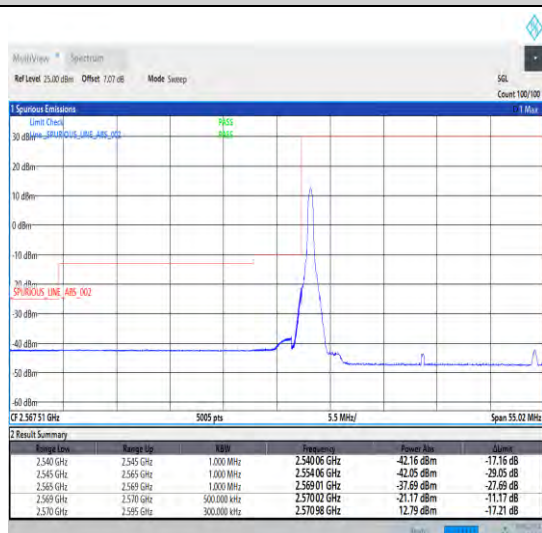
1-N38-30-25-L-4-CP-QPSK-Edge_1RB_Left-1@0-Ant1-1--PASS-see graph
