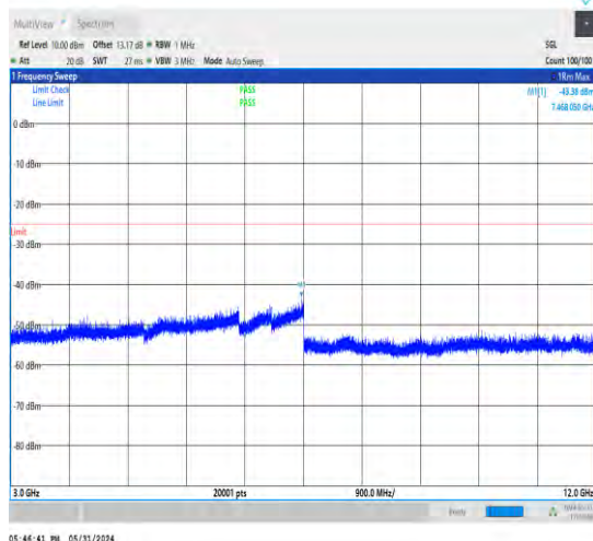
1-N38-30-40-M-1-DFT-PI2BPSK-Inner_1RB_Left-1 @1-3000-12000-Ant1-7491.45--43.38--25-PASS
