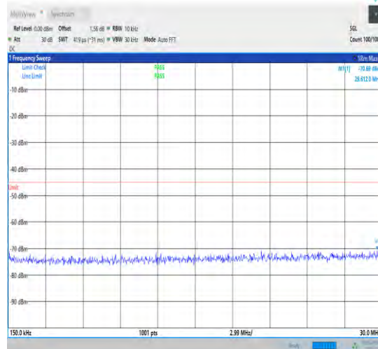
1-N38-30-40-H-1-DFT-PI2BPSK-Inner_1RB_Left-1@ 1-0.15-30-Ant1-23.43--70.69--45-PASS
