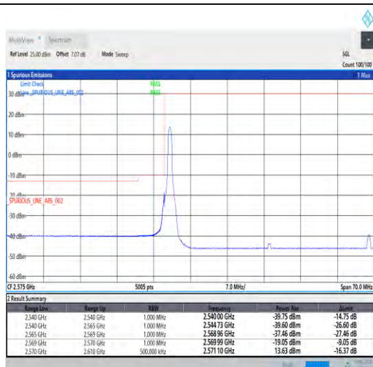
1-N38-30-40-L-1-DFT-PI2BPSK-Edge_1RB_Left-1@0-Ant1-1--PASS-see graph
