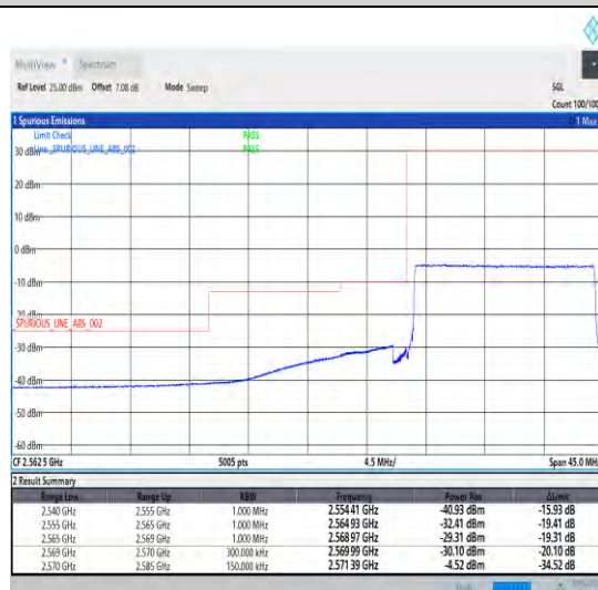
1-N38-30-15-L-6-CP-QPSK-Outer_Full-38@0-Ant1-1--PASS-see graph
