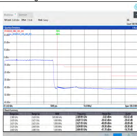
1-N38-30-40-H-3-DFT-PI2BPSK-Outer_Full-100@0-Ant1-1--PASS-see graph
