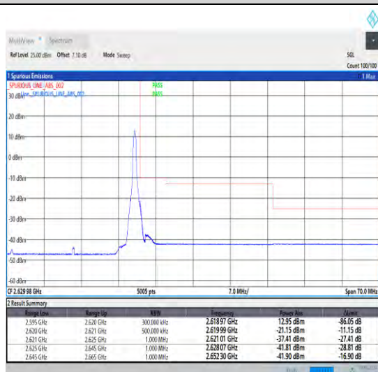
1-N38-30-25-H-5-CP-QPSK-Edge_1RB_Right-1@64-Ant1-1--PASS-see graph
