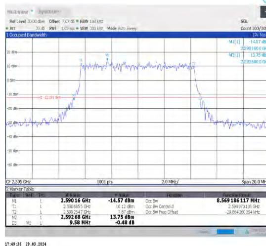
1-N38-30-10-M-4-DFT-64QAM-Outer_Full-24@0-Ant 1-8.569-9.580-≤10-PASS
