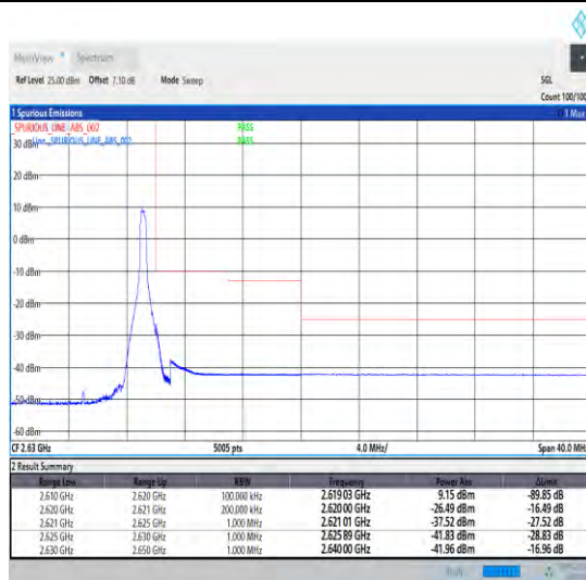
1-N38-30-10-H-2-DFT-PI2BPSK-Edge_1RB_Right-1@23-Ant1-1--PASS-see graph
