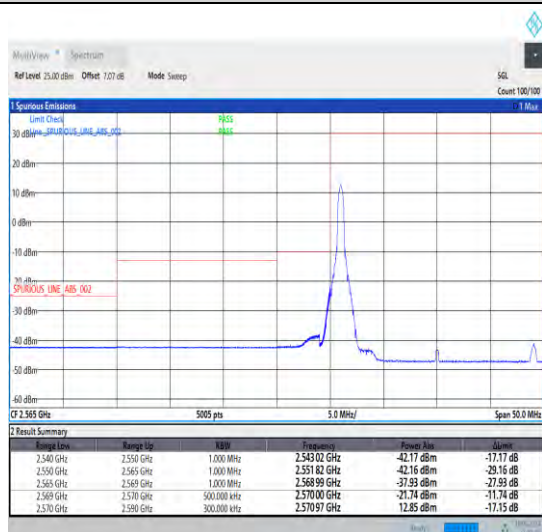
1-N38-30-20-L-4-CP-QPSK-Edge_1RB_Left-1@0-Ant1-1--PASS-see graph
