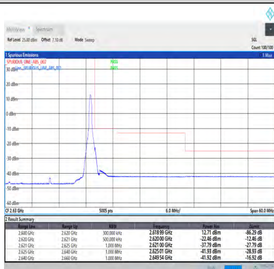
1-N38-30-20-H-5-CP-QPSK-Edge_1RB_Right-1@50-Ant1-1--PASS-see graph
