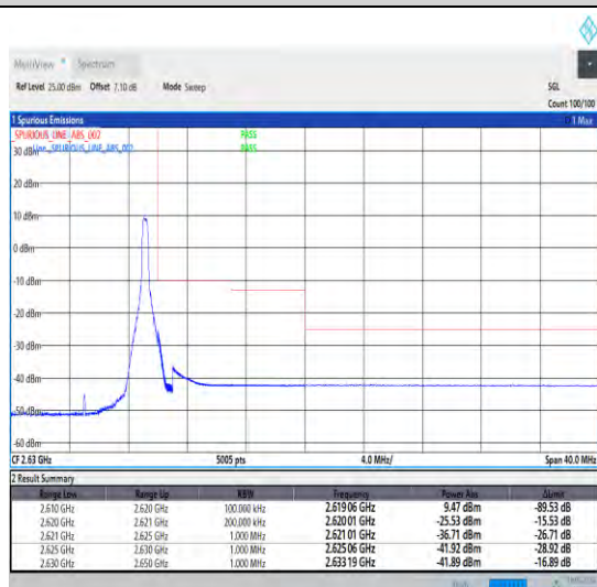
1-N38-30-10-H-5-CP-QPSK-Edge_1RB_Right-1@23-Ant1-1--PASS-see graph
