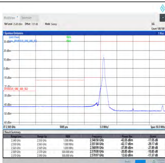
1-N38-30-20-L-1-DFT-PI2BPSK-Edge_1RB_Left-1@0-Ant1-1--PASS-see graph
