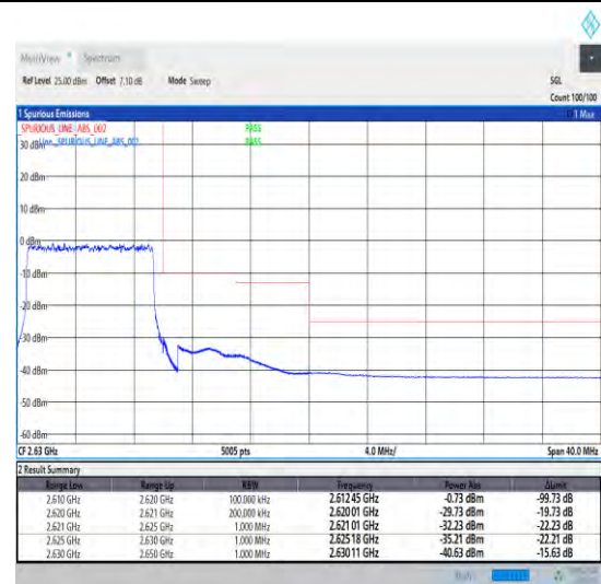
1-N38-30-10-H-3-DFT-PI2BPSK-Outer_Full-24@0-Ant1-1--PASS-see graph
