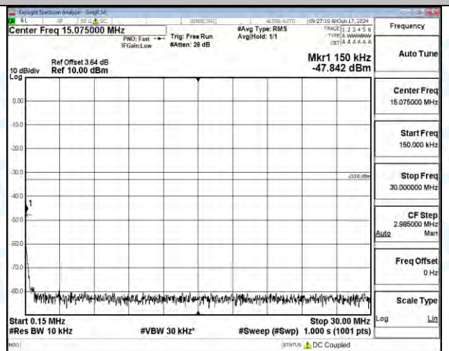
Band2_10MHz_16QAM_19150_1RB#49_1000~3000_1000~3000
