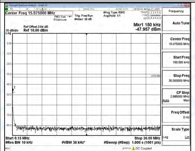
Band2_5MHz_16QAM_18900_25RB#0_1000~3000_1000~3000
