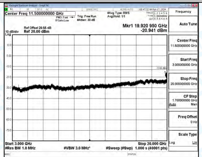
Band2_5MHz_QPSK_18625_25RB#0_0.15~0.30_0.15~0.30
