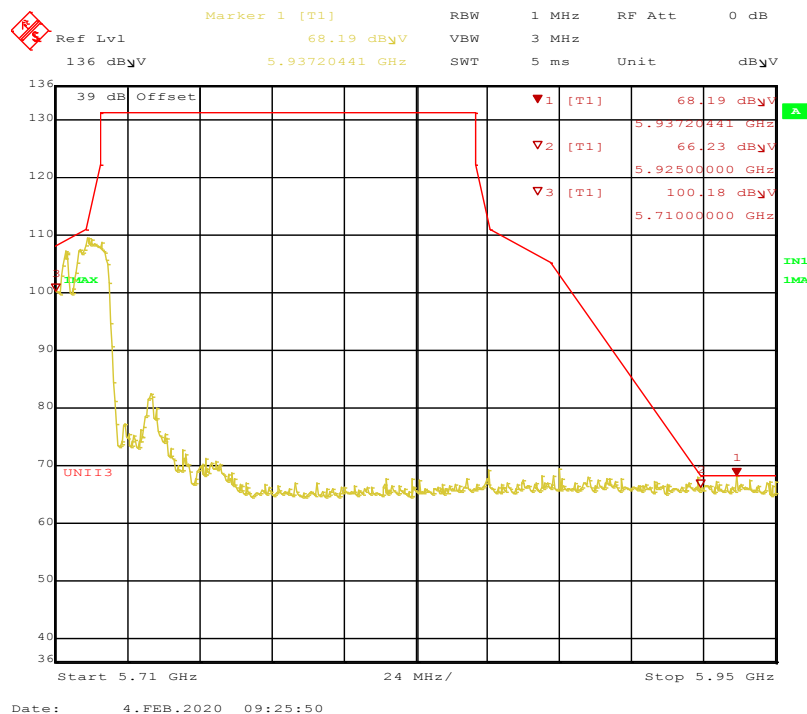
Figure 107: 802.11ac VHT40-MCS0-TP18.5-5710MHz-Peak-Horizontal-2x2
