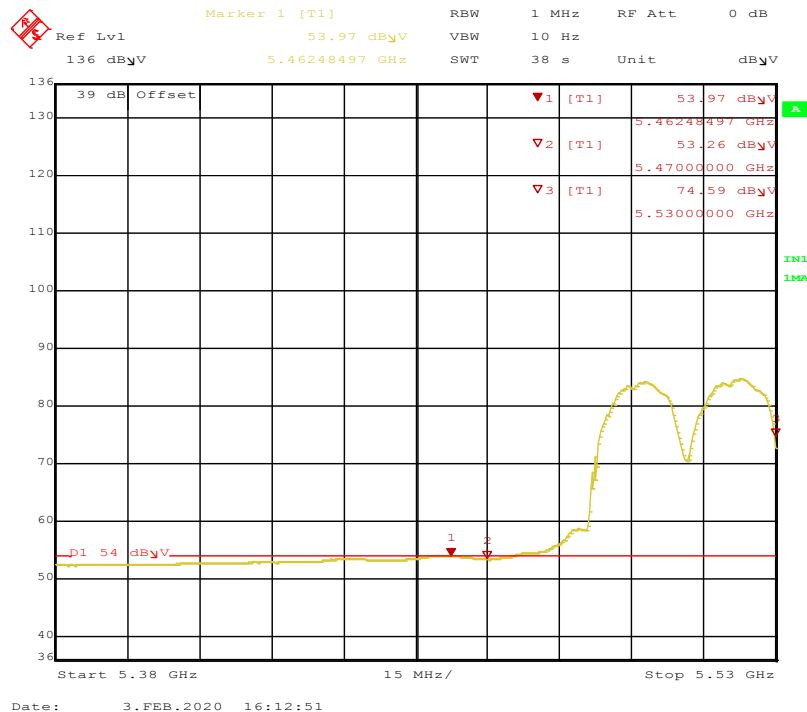
Figure 101: 802.11ac VHT80-MCS0-TP17-5530MHz-Average-Vertical-2x2
