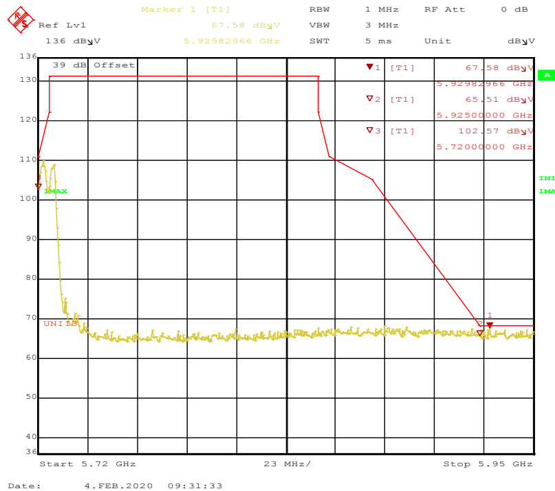
Figure 105: 802.11a-6Mbps-TP17-5720MHz-Peak-Horizontal-2x2
