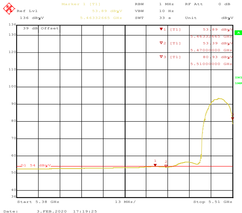
Figure 99: 802.11ac VHT40-MCS0-TP16.5-5510MHz-Average-Horizontal-2x2
