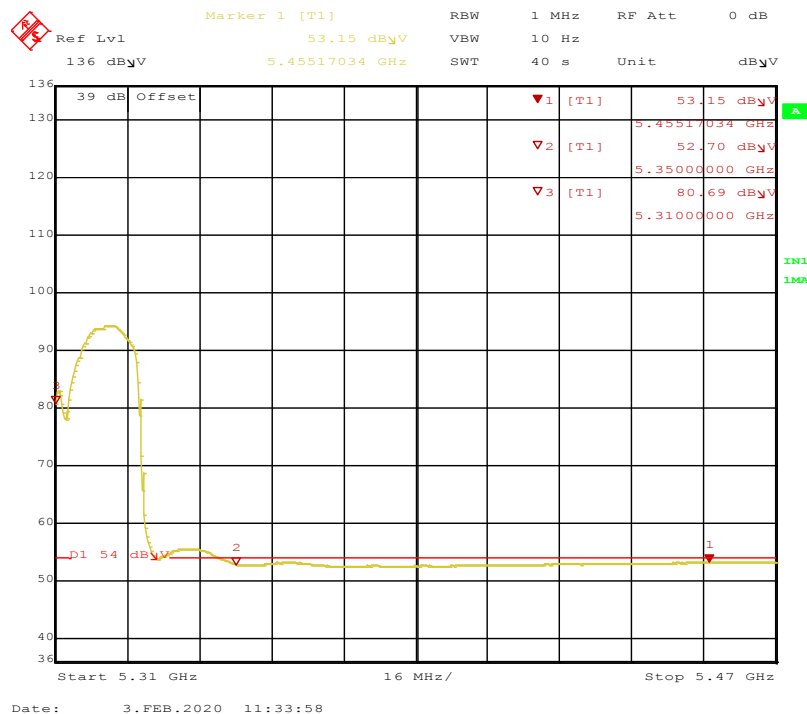
Figure 87: 802.11ac VHT40-MCS0-TP16.5-5310MHz-Average-Horizontal-2x2
