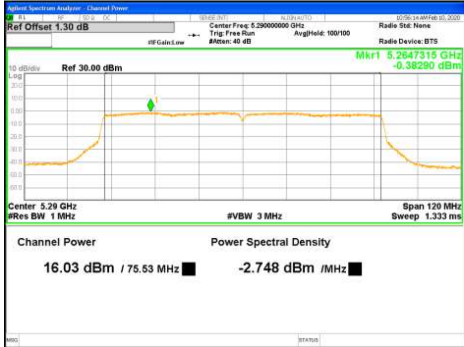
Figure 44: RMS Max Power-5290MHz-802.11ac VHT80-MCS0-TP17-2x2-CH1 (FCC)
