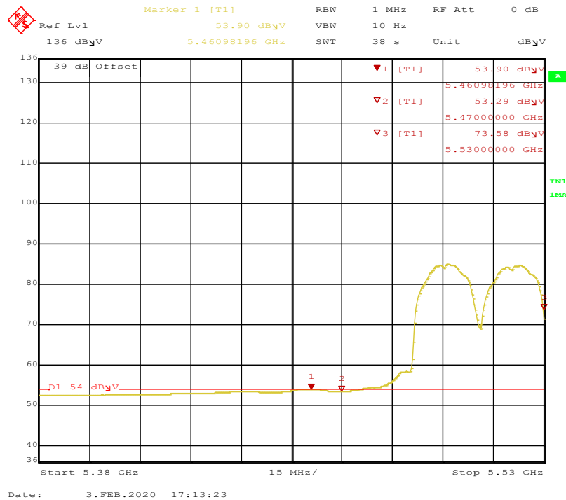
Figure 103: 802.11ac VHT80-MCS0-TP17-5530MHz-Average-Horizontal-2x2
