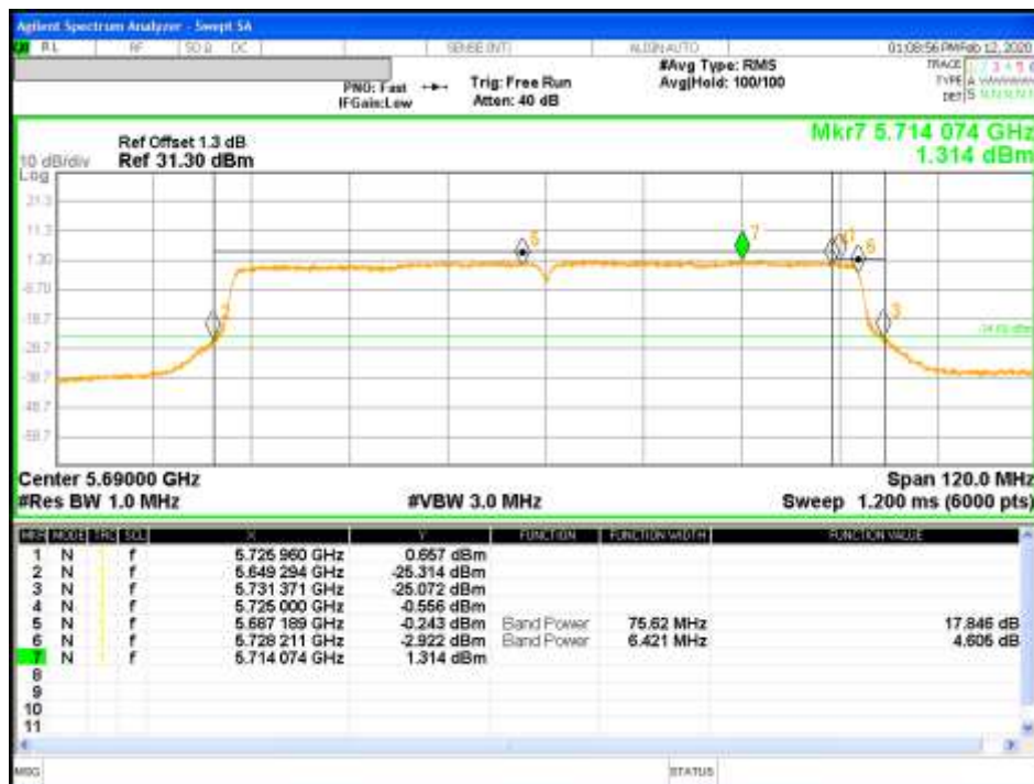
Figure 51: RMS Max Power & PSD-5690MHz-802.11ac VHT80-MCS0-TP19-2x2-CH1 (Straddle Channel in UNII2C & UNII3C)
