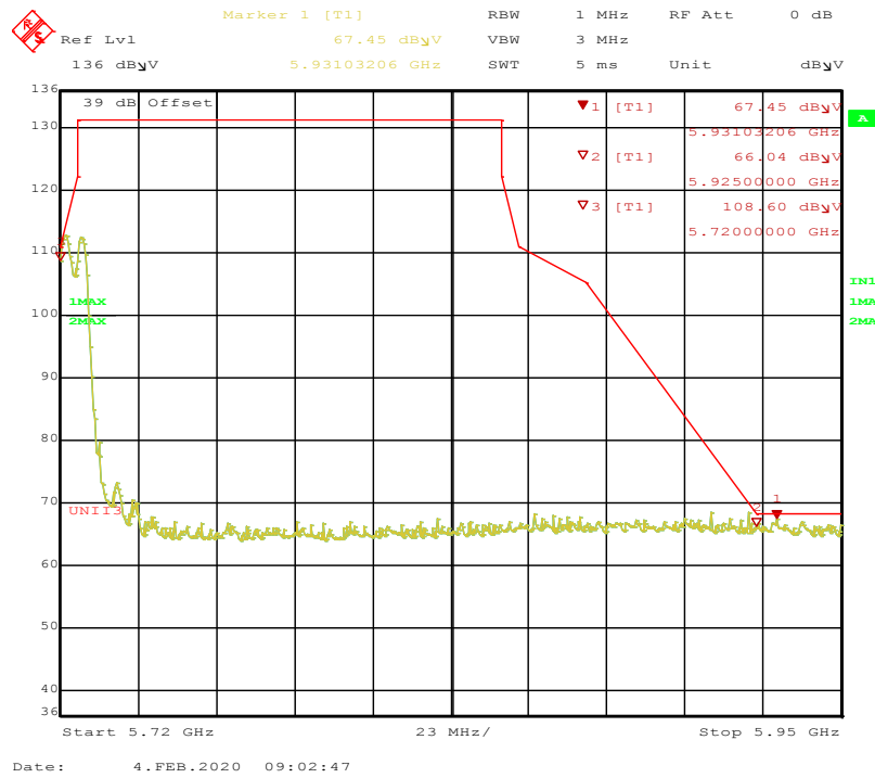
Figure 104: 802.11a-6Mbps-TP17-5720MHz-Peak-Vertical-2x2
