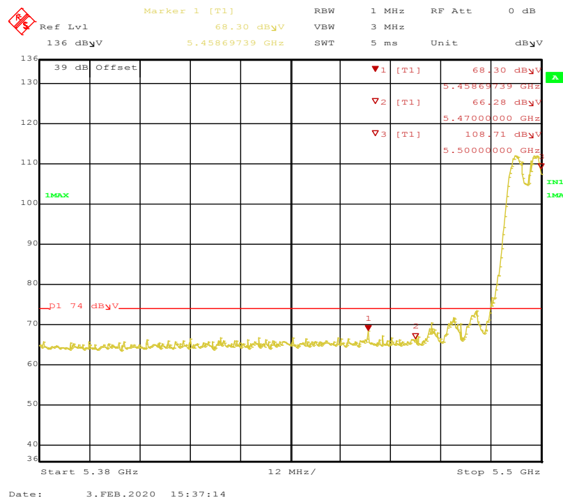
Figure 92: 802.11a-6Mbps-TP17-5500MHz-Peak-Vertical-2x2
