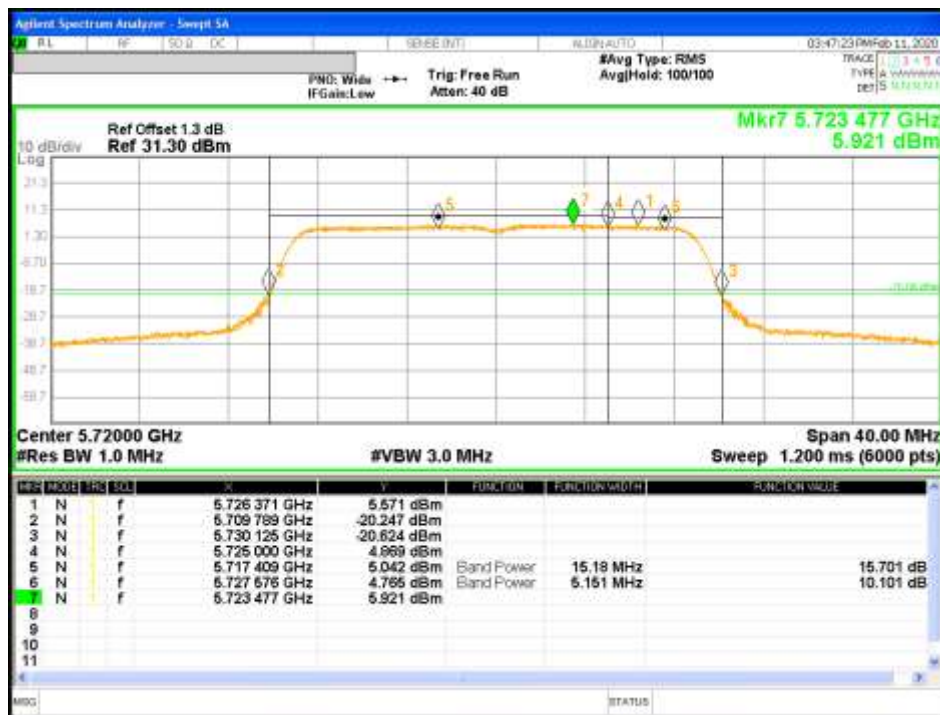
Figure 49: RMS Max Power & PSD-5720MHz-802.11ac VHT20-MCS0-TP17-2x2-CH1 (Straddle Channel in UNII2C & UNII3)
