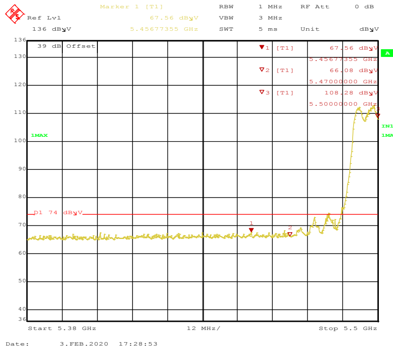
Figure 94: 802.11a-6Mbps-TP17-5500MHz-Peak-Horizontal-2x2
