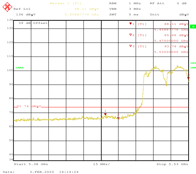
Figure 100: 802.11ac VHT80-MCS0-TP17-5530MHz-Peak-Vertical-2x2
