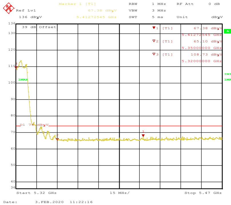
Figure 82: 802.11a-6Mbps-5320MHz-TP17-Peak-Horizontal-2x2
