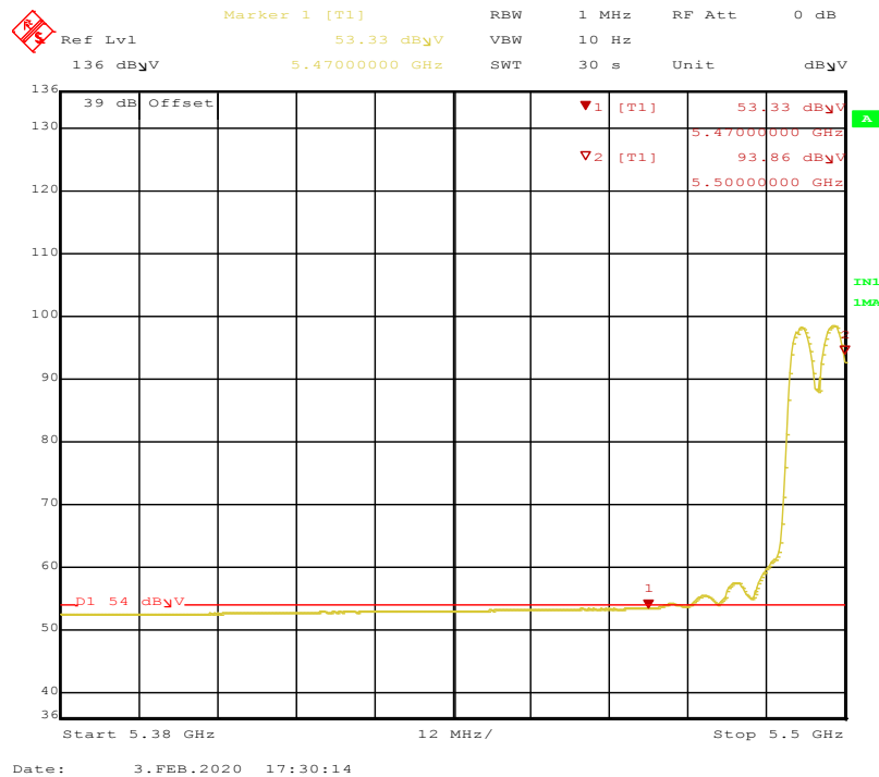
Figure 95: 802.11a-6Mbps-TP17-5500MHz-Average-Horizontal-2x2
