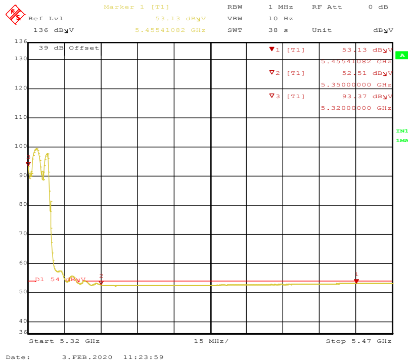
Figure 83: 802.11a-6Mbps-5320MHz-TP17-Average-Horizontal-2x2
