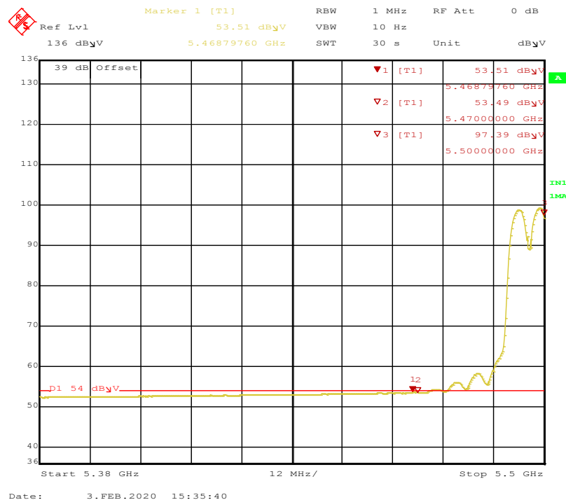
Figure 93: 802.11a-6Mbps-TP17-5500MHz-Average-Vertical-2x2
