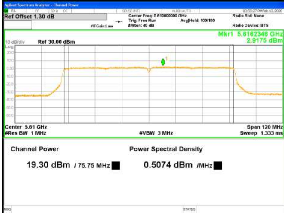
Figure 26: RMS Max Power-5610MHz-802.11ac VHT80-MCS0-TP20.5-1x2-CH1
