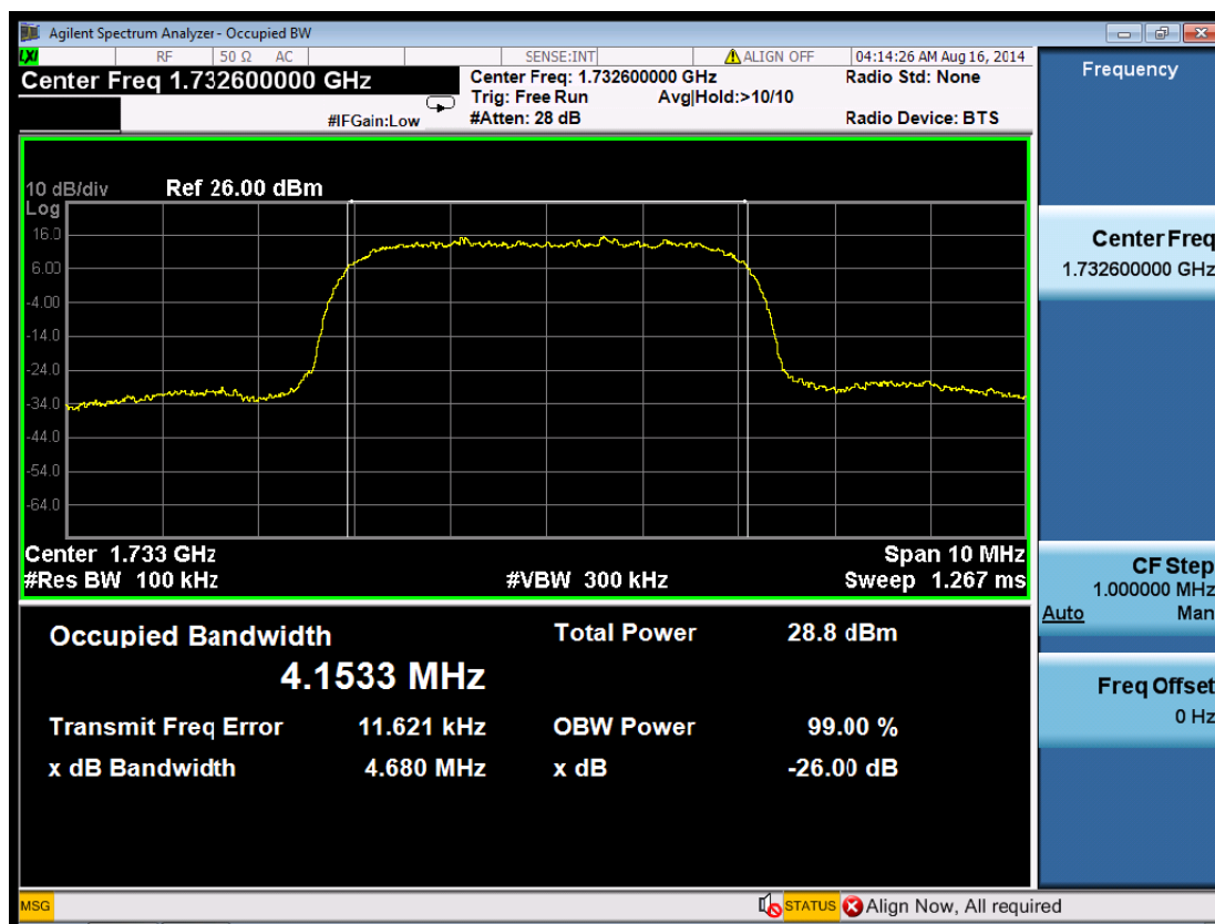
(Plot 5.3.2 B: Channel 1413: 1732.6MHz WCDMA Band IV)
