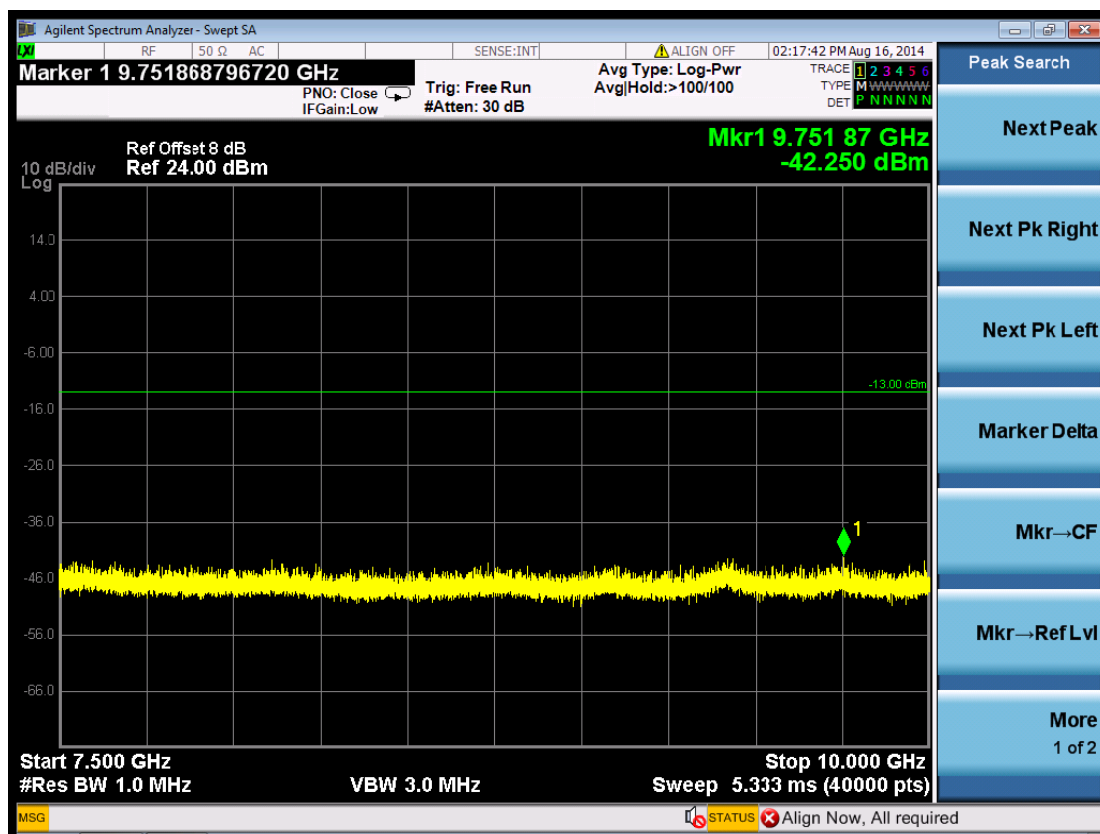
(Plot 5.5.3 B6: Channel 1413: 1732.6MHz @ Traffic WCDMA Band IV)
