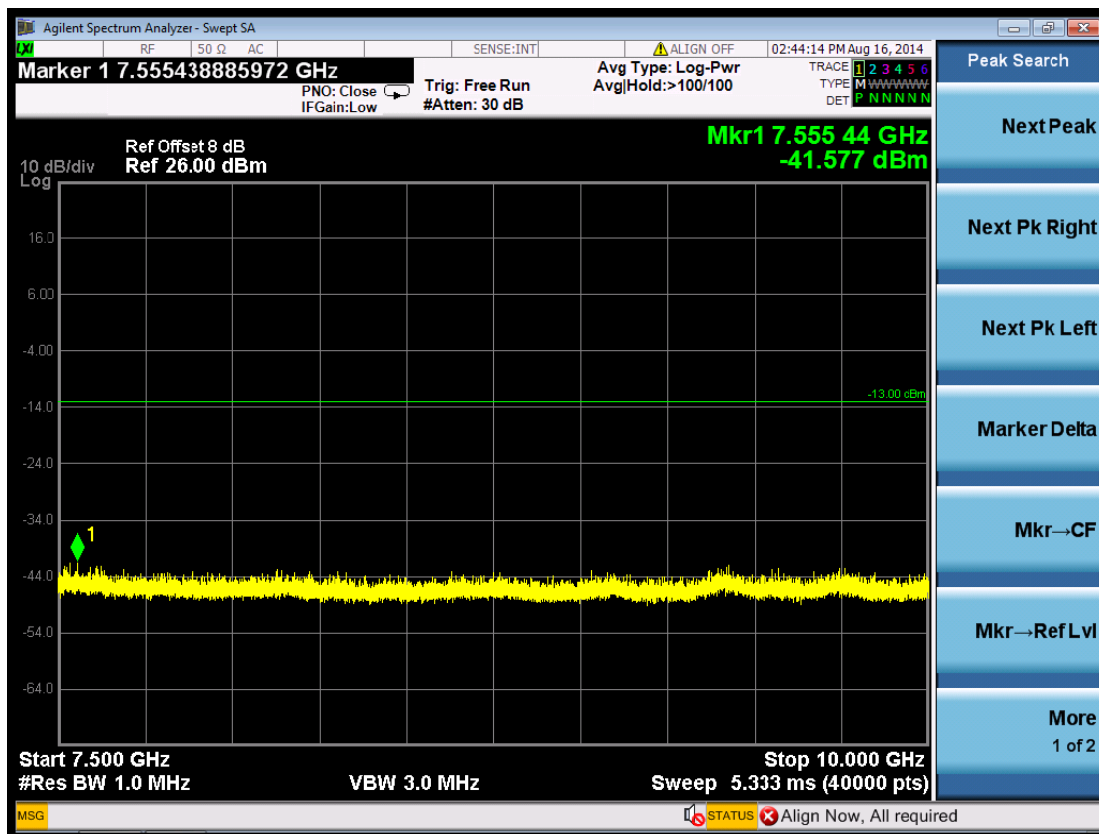
(Plot 5.5.1 B6: Channel 9400: 1880.0MHz @ Traffic WCDMA Band II)
