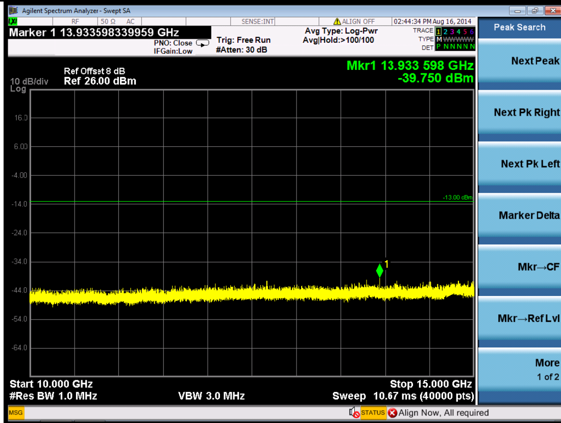
(Plot 5.5.1 B7: Channel 9400: 1880.0MHz @ Traffic WCDMA Band II)
