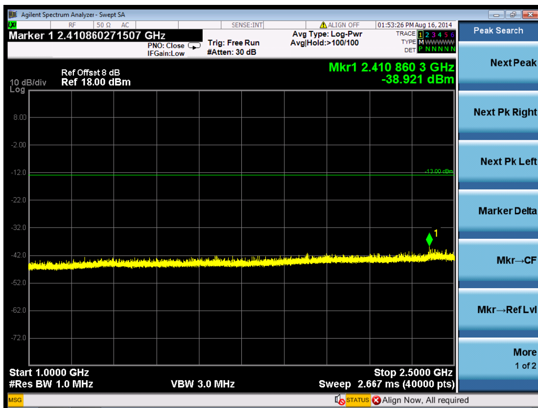
(Plot 5.5.2 D4: Idle @ WCDMA Band V)
