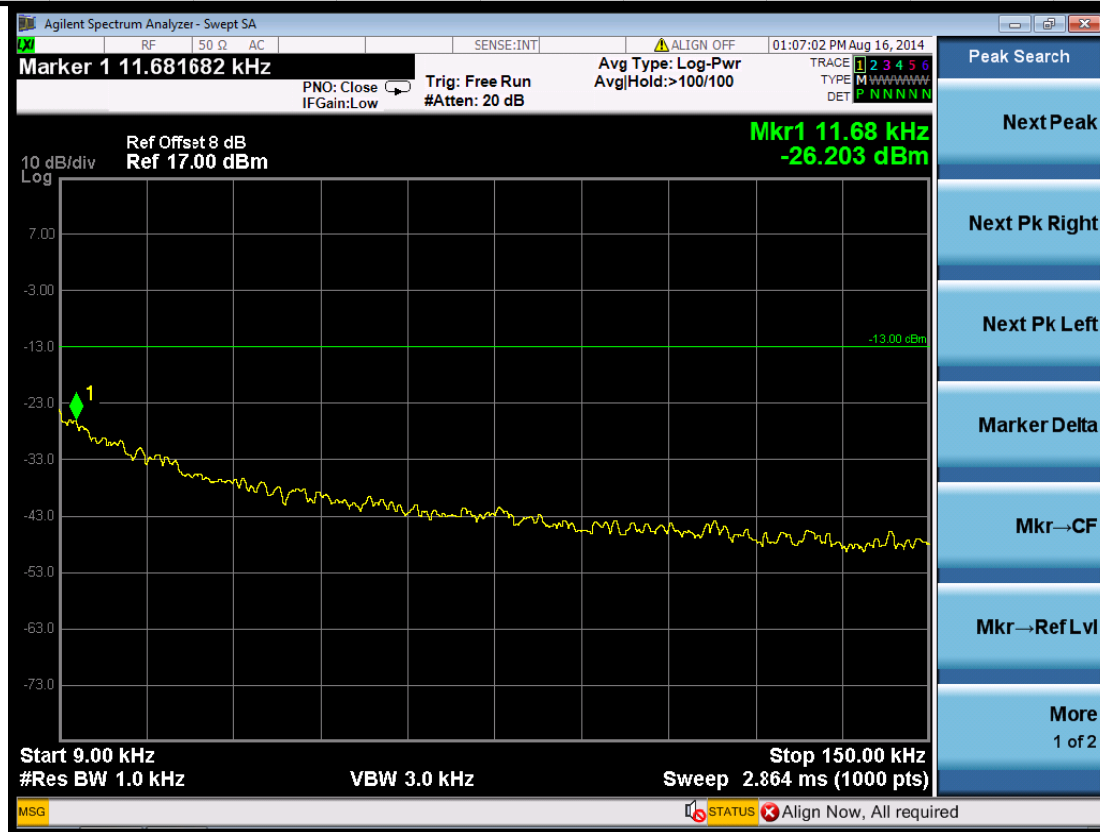
(Plot 5.5.2 C1: Channel 4233: 846.60 MHz @ WCDMA Band V)
