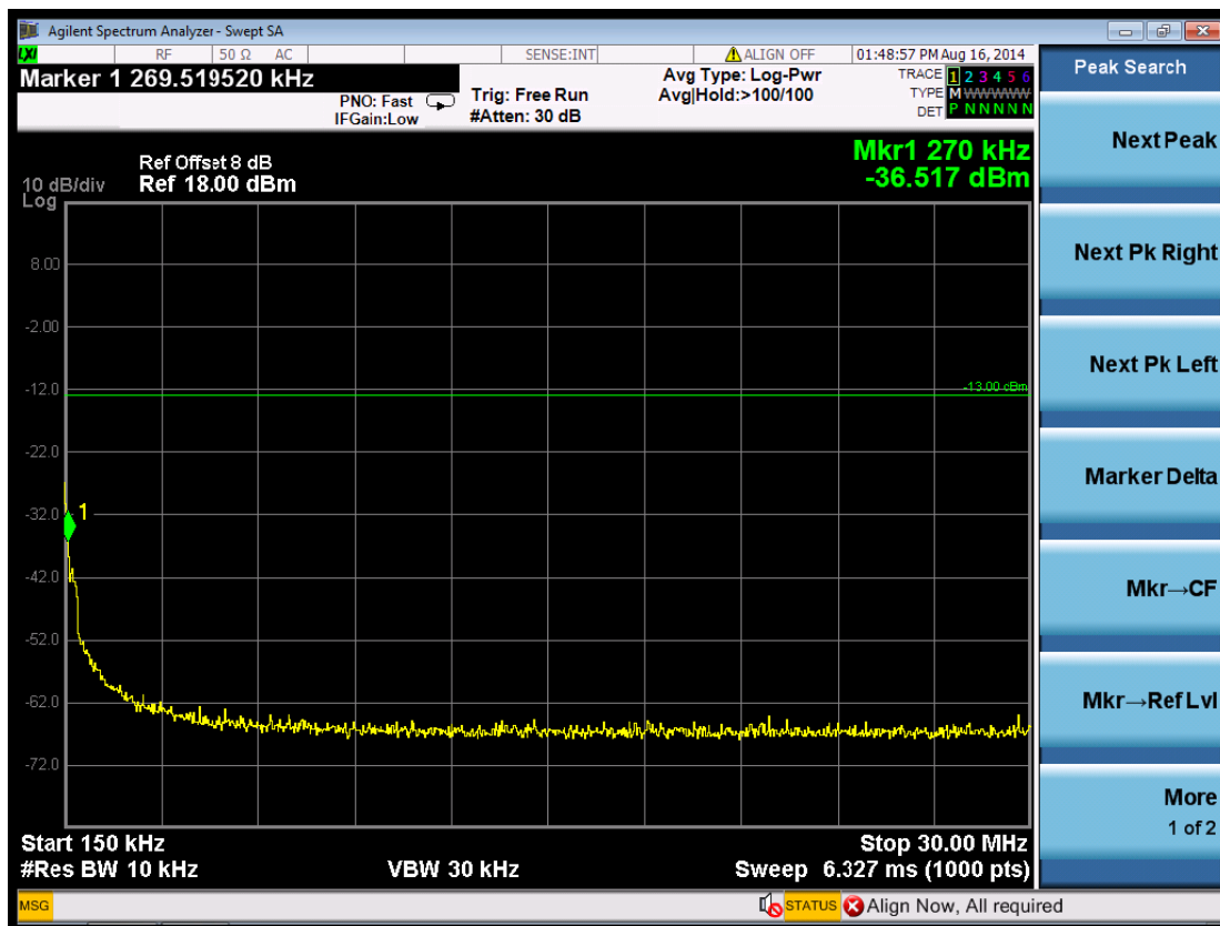
(Plot 5.5.2 D2: Idle @ WCDMA Band V)
