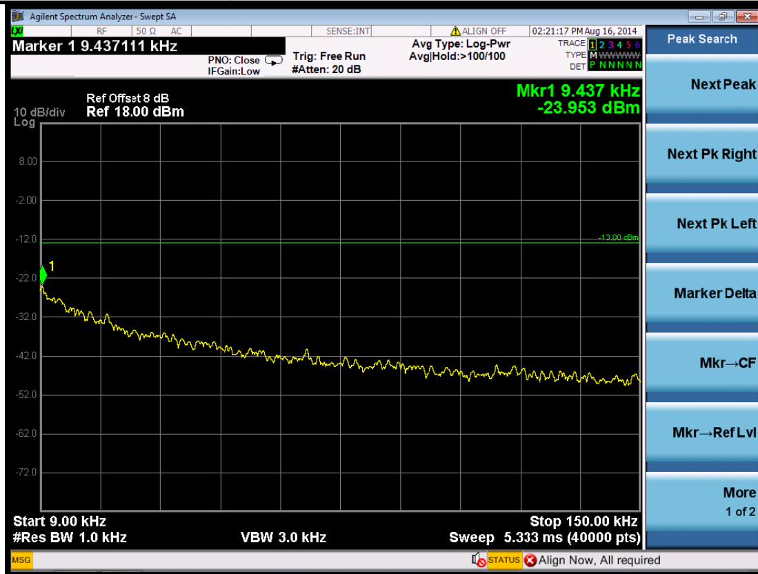
(Plot 5.5.3 C1: Channel 1513: 1752.6MHz @ Traffic WCDMA Band IV)
