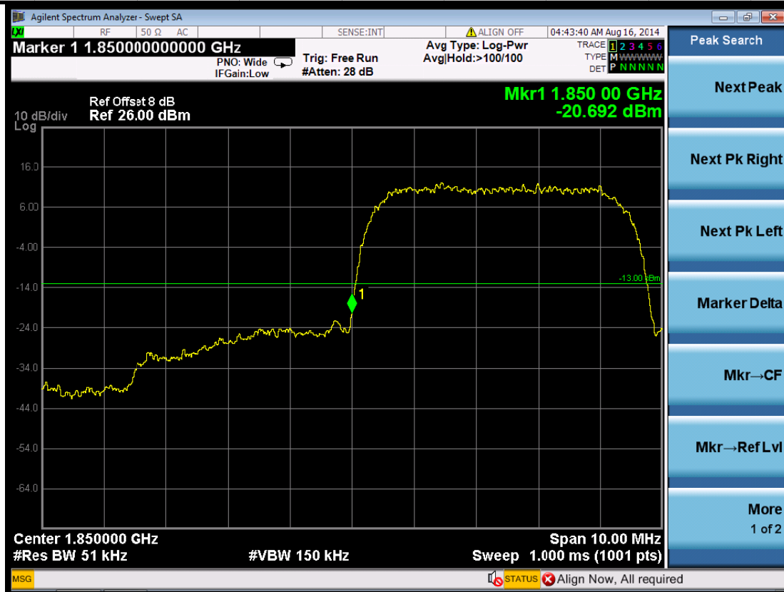
(Plot 5.4.1 A: Channel 9262: 1852.4MHz WCDMA Band II)
