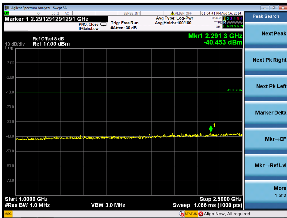
(Plot 5.5.2 B4: Channel 4183: 836.60 MHz @ WCDMA Band V)
