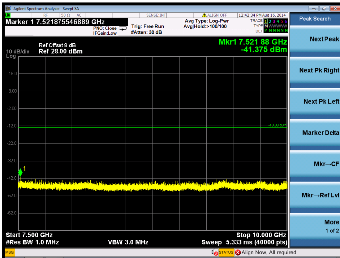
(Plot 5.5.2 A6: Channel 4132: 826.40 MHz @ WCDMA Band V)
