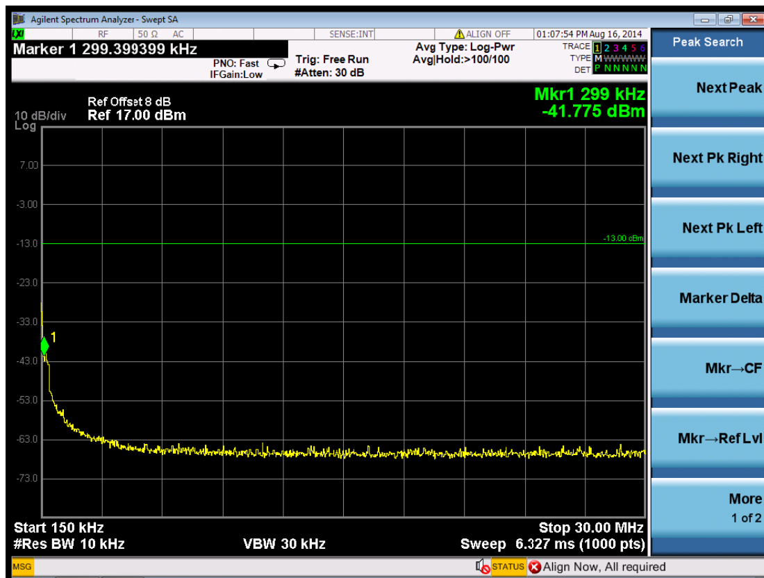
(Plot 5.5.2 C2: Channel 4233: 846.60 MHz @ WCDMA Band V)
