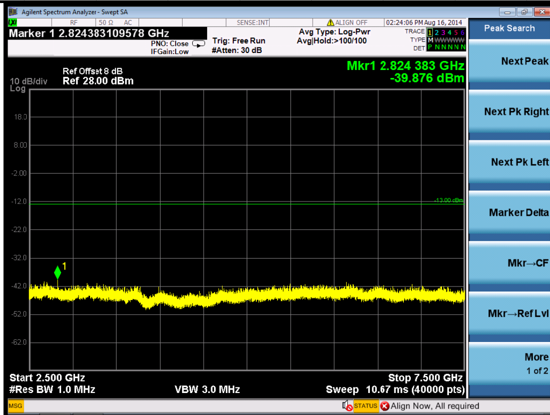
(Plot 5.5.3 C5: Channel 1513: 1752.6MHz @ Traffic WCDMA Band IV)
