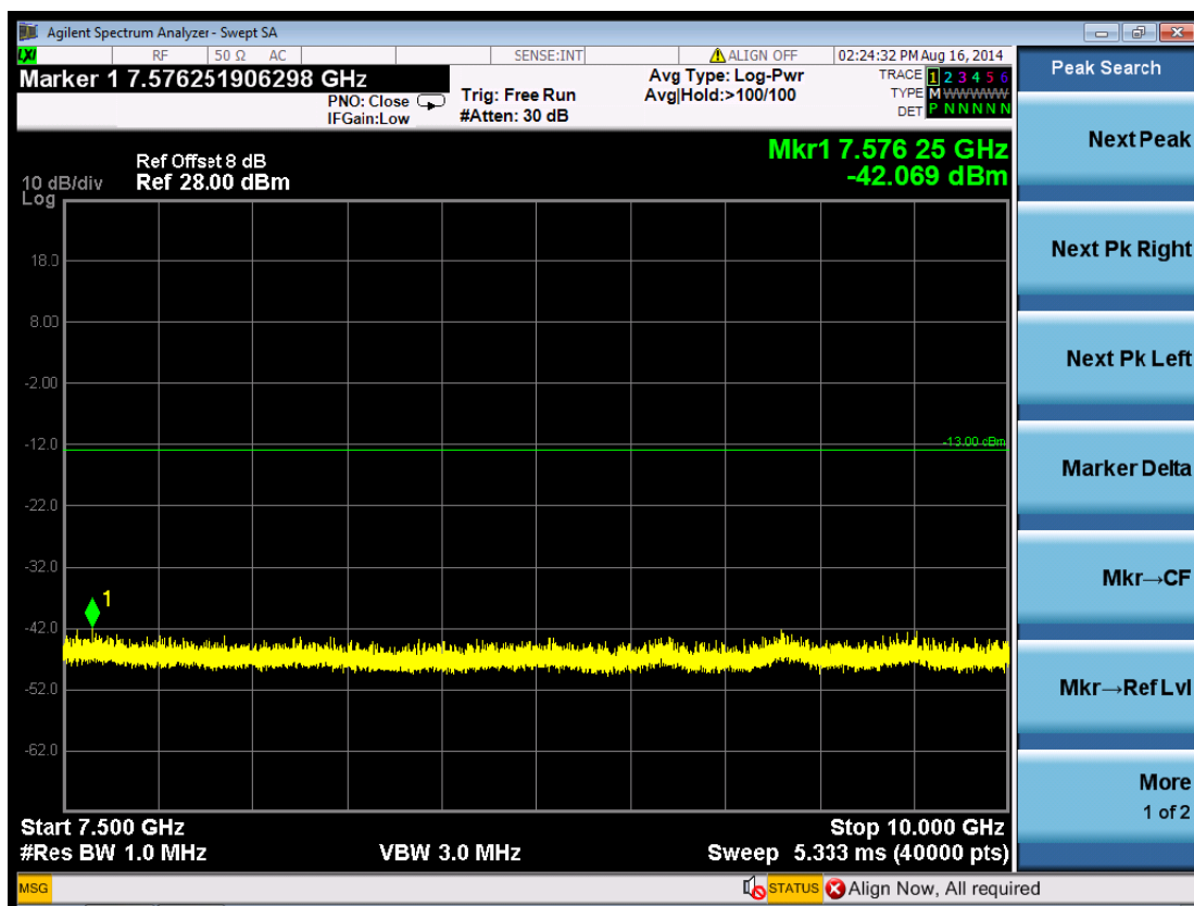
(Plot 5.5.3 C6: Channel 1513: 1752.6MHz @ Traffic WCDMA Band IV)
