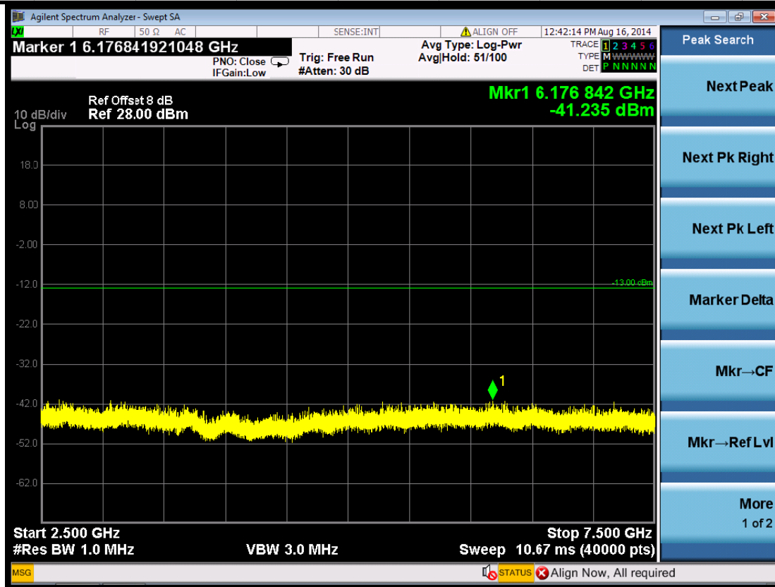
(Plot 5.5.2 A5: Channel 4132: 826.40 MHz @ WCDMA Band V)
