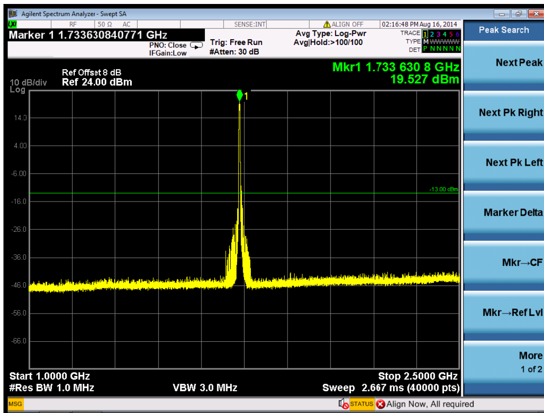
(Plot 5.5.3 B4: Channel 1413: 1732.6MHz @ Traffic WCDMA Band IV)
