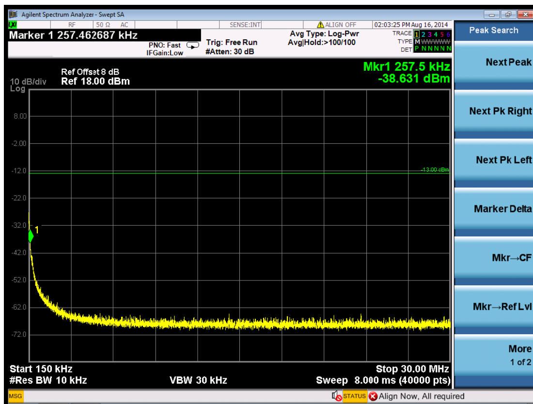
(Plot 5.5.3 D2: Idle WCDMA Band IV)
