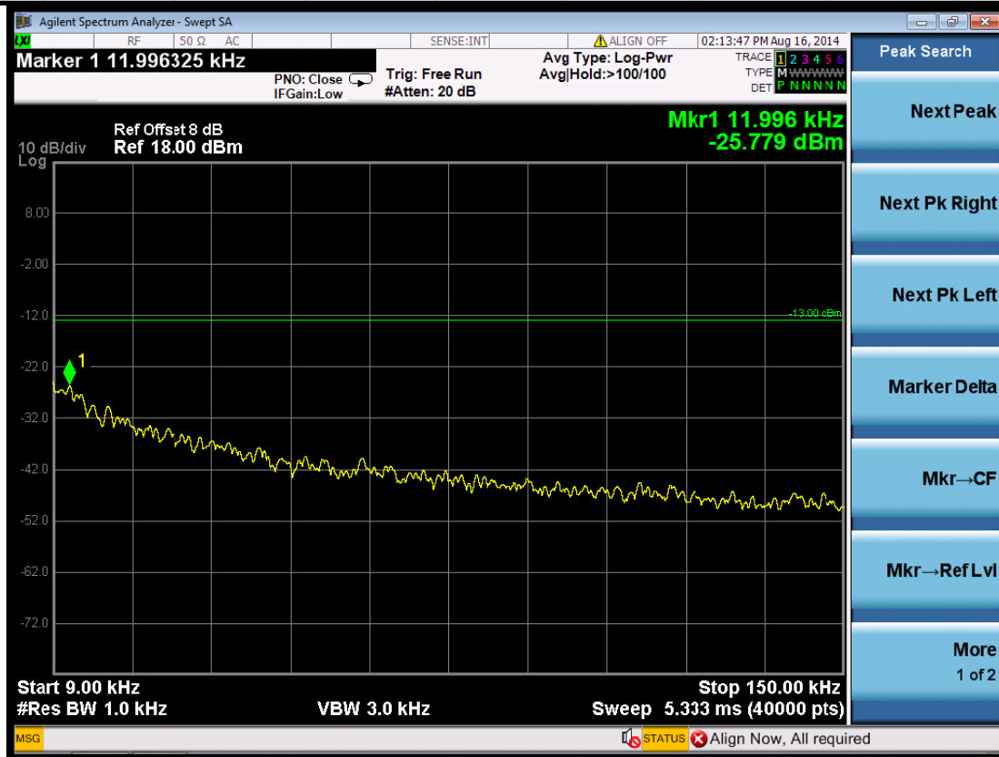
(Plot 5.5.3 B1: Channel 1413: 1732.6MHz @ Traffic WCDMA Band IV)
