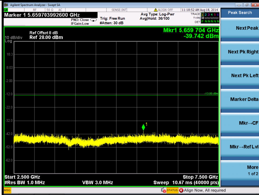
(Plot 5.5.1 C5: Channel 9538: 1907.6MHz @ Traffic WCDMA Band II)
