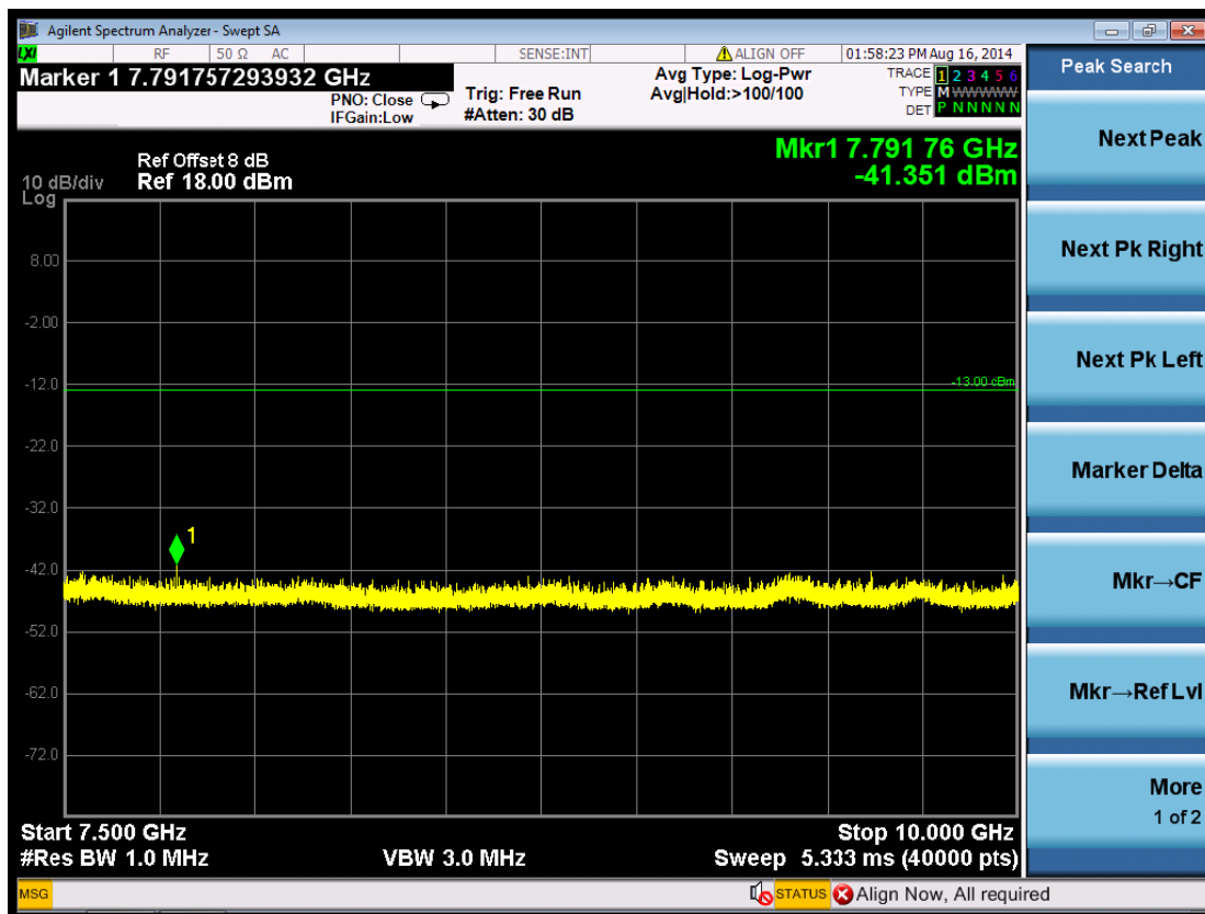
(Plot 5.5.2 D6: Idle @ WCDMA Band V)
