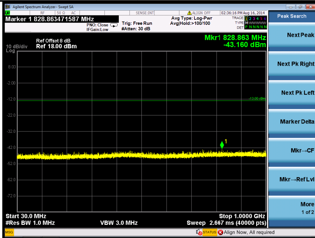
(Plot 5.5.1 A3: Channel 9262: 1852.4MHz @ Traffic WCDMA Band II)
