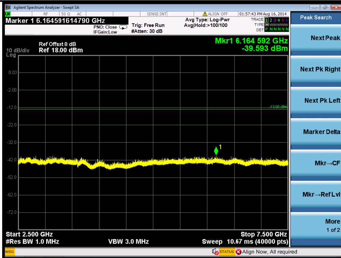
(Plot 5.5.2 D5: Idle @ WCDMA Band V)
