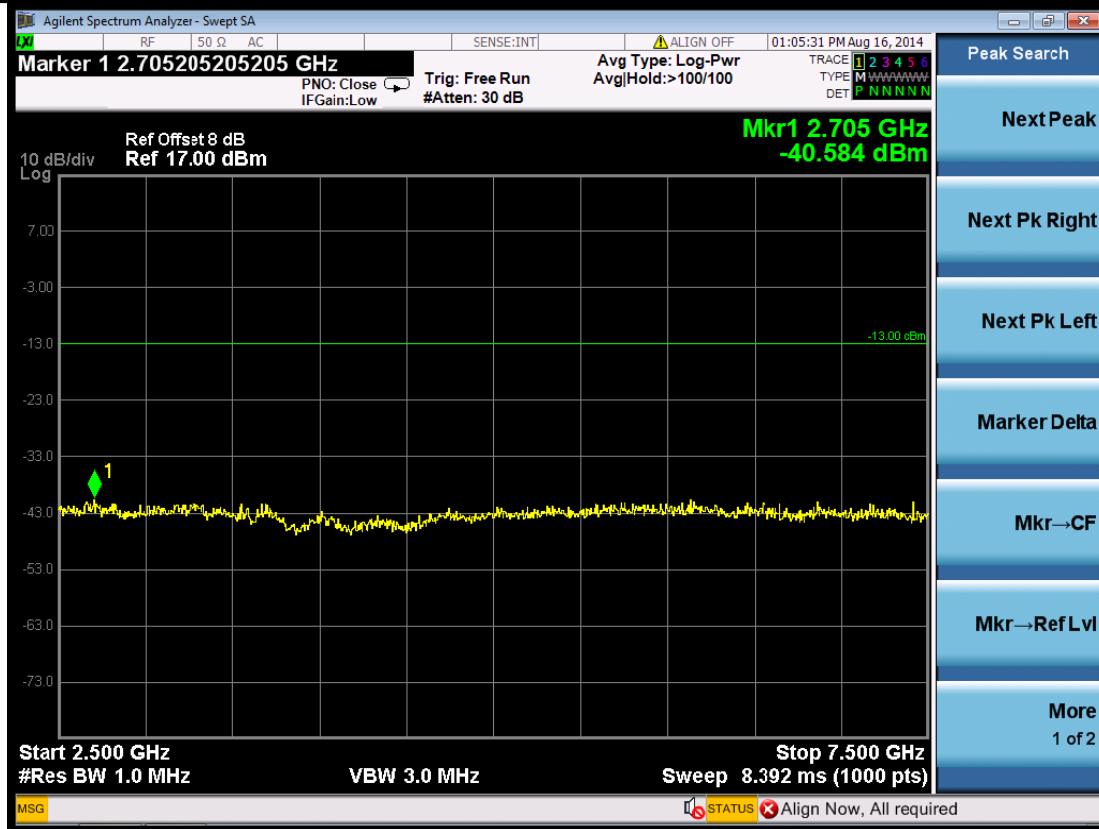
(Plot 5.5.2 B5: Channel 4183: 836.60 MHz @ WCDMA Band V)
