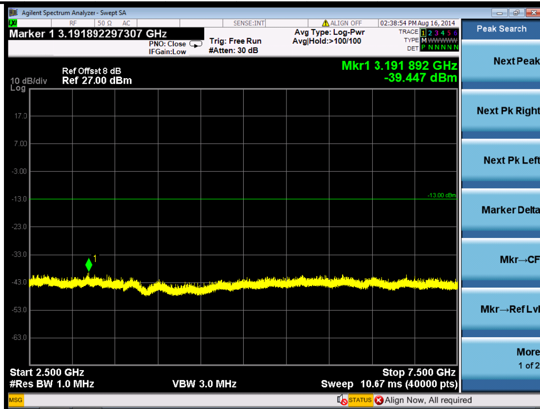
(Plot 5.5.1 A5: Channel 9262: 1852.4MHz @ Traffic WCDMA Band II)
