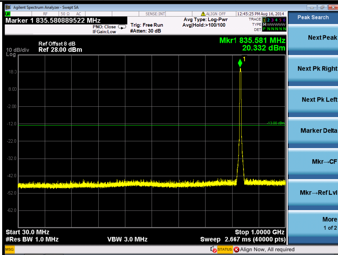
(Plot 5.5.2 B3: Channel 4183: 836.60 MHz @ WCDMA Band V)
