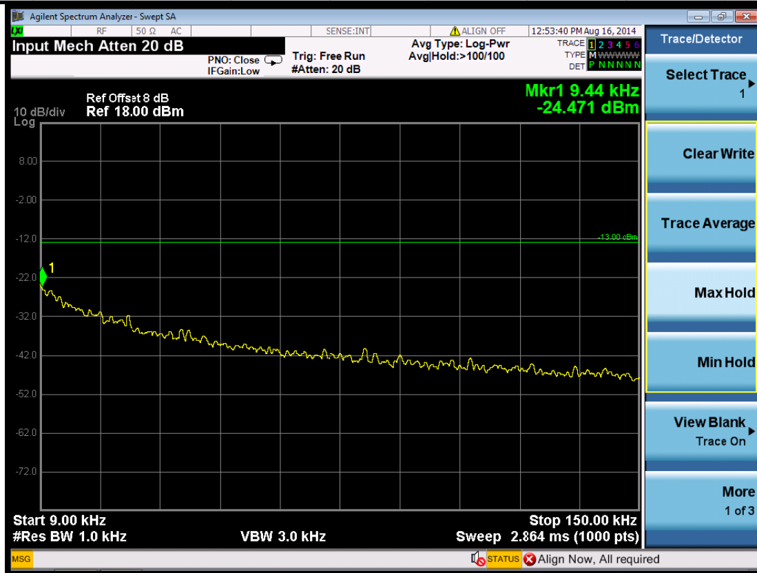
(Plot 5.5.2 B1: Channel 4183: 836.60 MHz @ WCDMA Band V)
