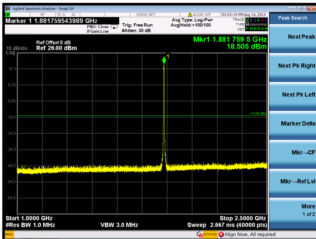
(Plot 5.5.1 B4: Channel 9400: 1880.0MHz @ Traffic WCDMA Band II)
