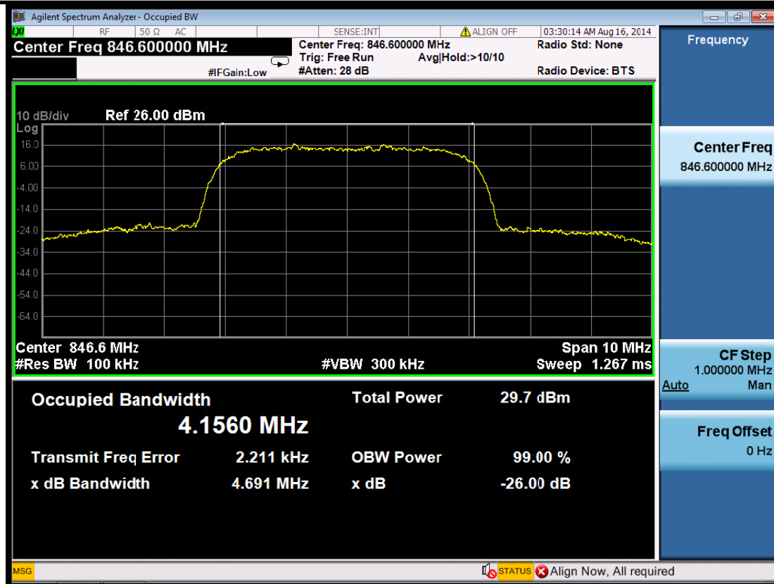
(Plot 5.3.3 C: Channel 4233:846.6MHz @ WCDMA Band V)
