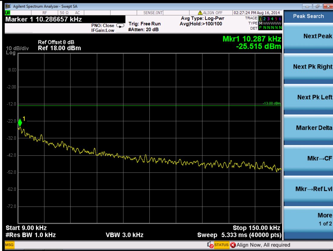
(Plot 5.5.1 D1: Idle WCDMA Band II)
