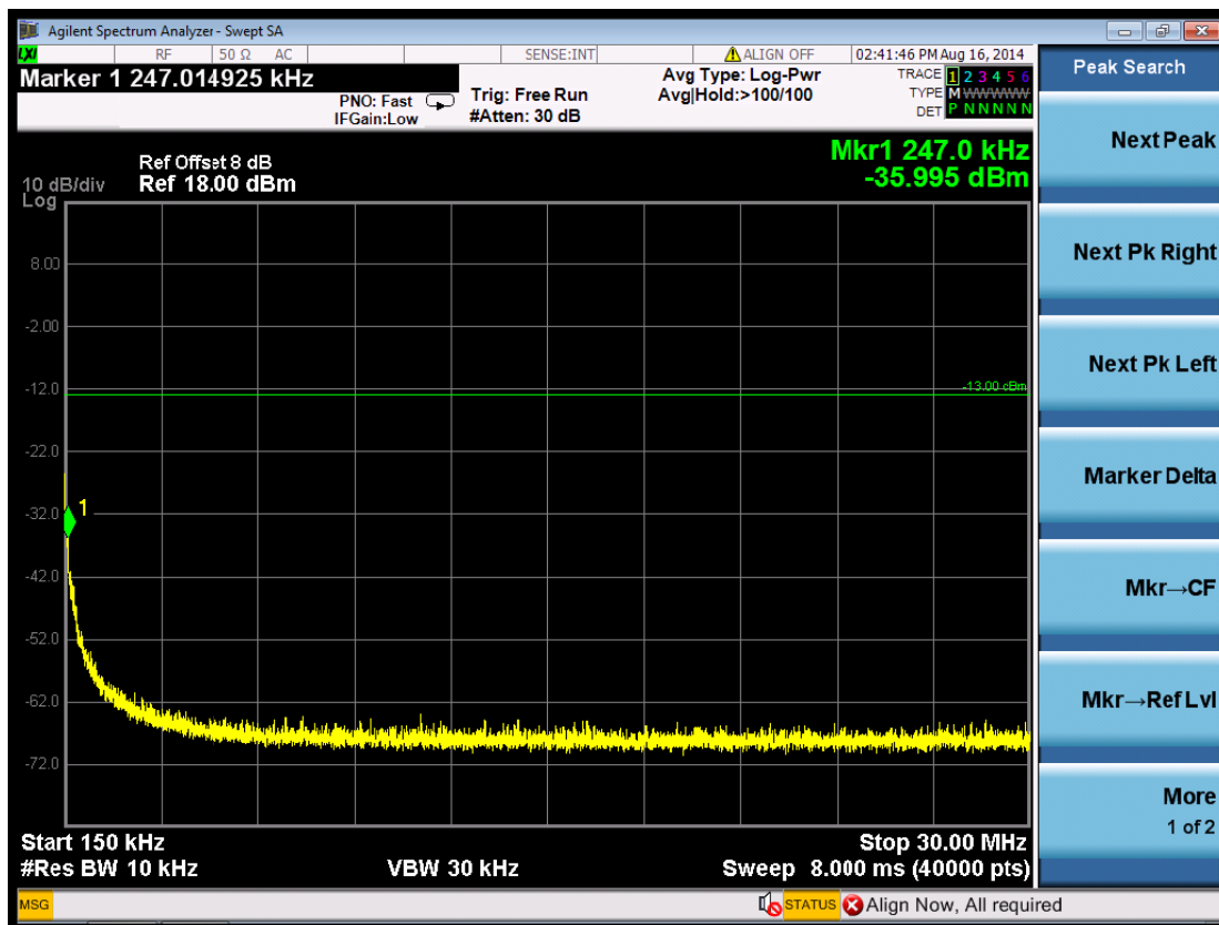
(Plot 5.5.1 B2: Channel 9400: 1880.0MHz @ Traffic WCDMA Band II)
