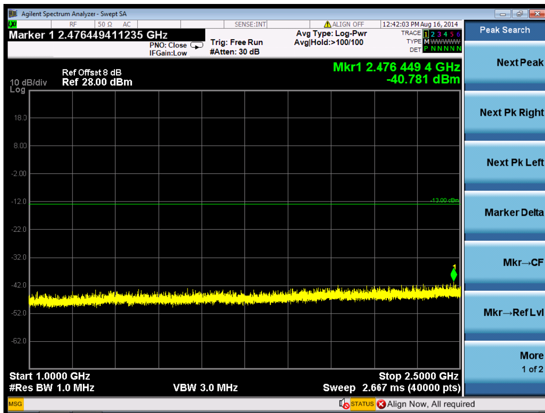
(Plot 5.5.2 A4: Channel 4132: 826.40 MHz @ WCDMA Band V)
