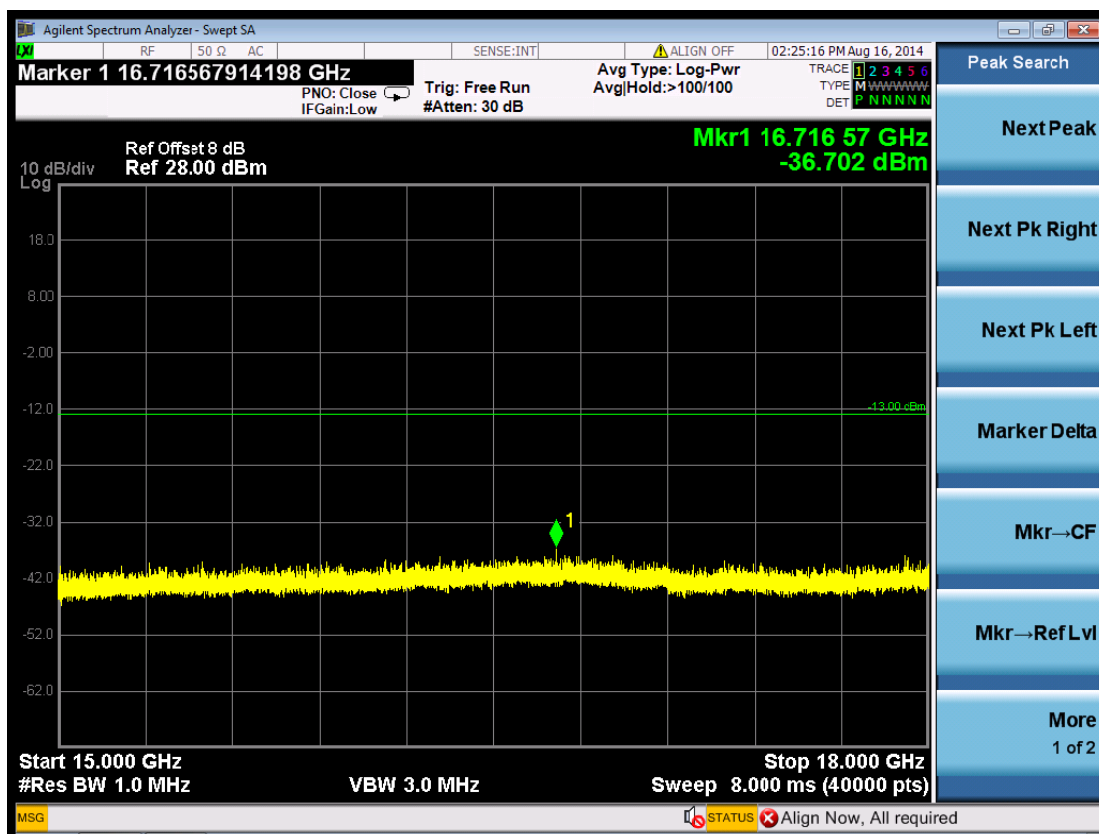
(Plot 5.5.3 C8: Channel 1513: 1752.6MHz @ Traffic WCDMA Band IV)
