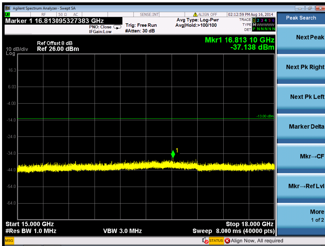
(Plot 5.5.3 A8: Channel 1312: 1712.4MHz @ Traffic WCDMA Band IV)
