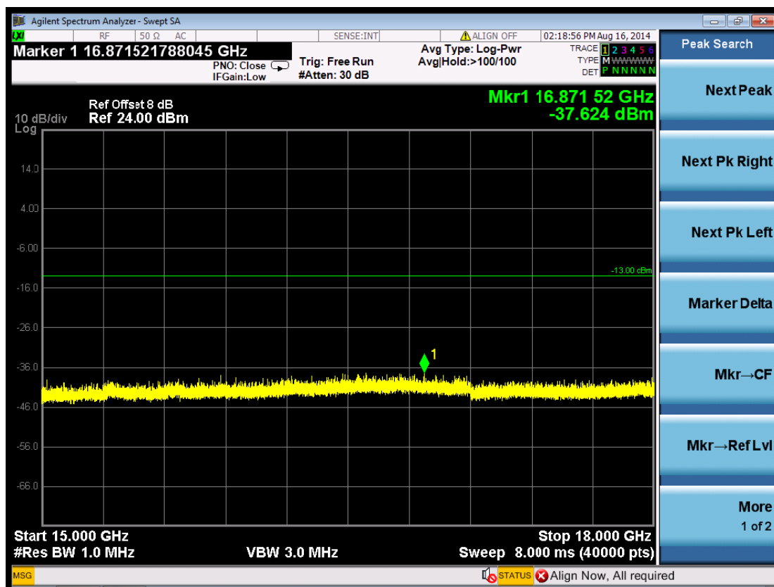
(Plot 5.5.3 B8: Channel 1413: 1732.6MHz @ Traffic WCDMA Band IV)
