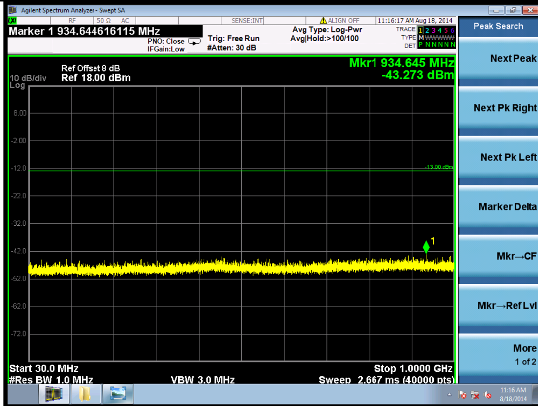
(Plot 5.5.1 C3: Channel 9538: 1907.6MHz @ Traffic WCDMA Band II)
