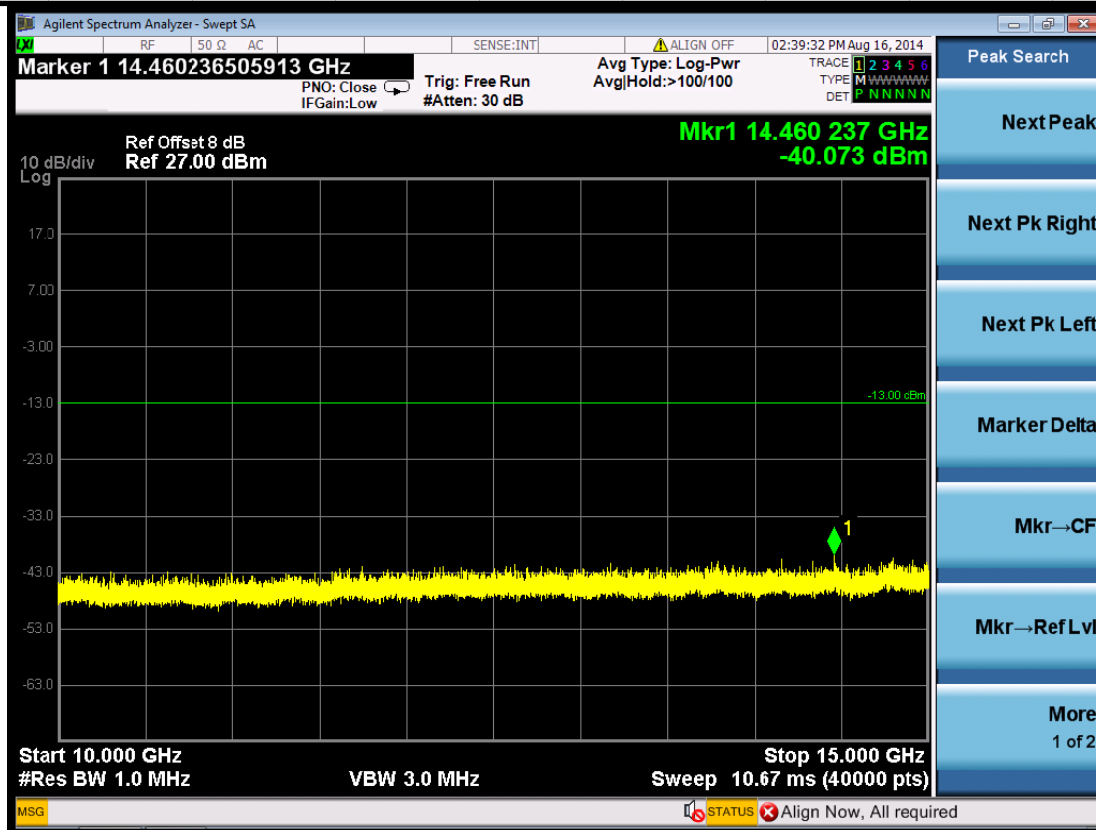
(Plot 5.5.1 A7: Channel 9262: 1852.4MHz @ Traffic WCDMA Band II)
