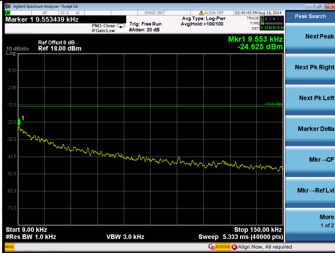
(Plot 5.5.1 B1: Channel 9400: 1880.0MHz @ Traffic WCDMA Band II)
