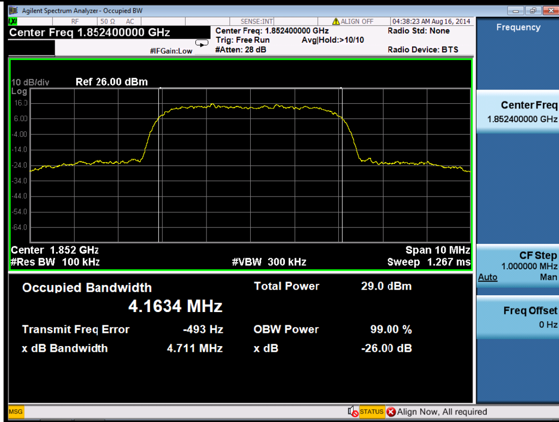
(Plot 5.3.1 A: Channel 9262: 1852.4MHz WCDMA Band II)
