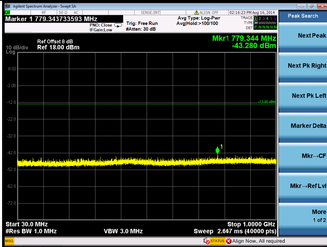
(Plot 5.5.3 B3: Channel 1413: 1732.6MHz @ Traffic WCDMA Band IV)
