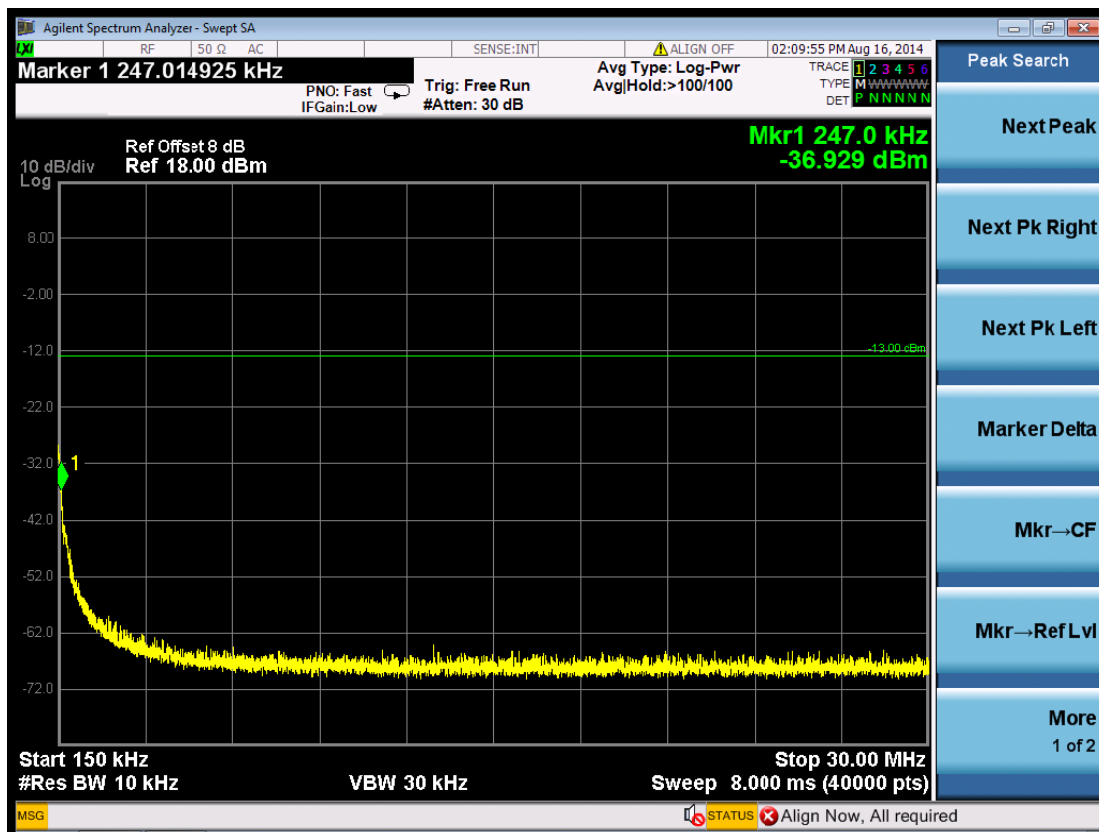
(Plot 5.5.3 A2: Channel 1312: 1712.4MHz @ Traffic WCDMA Band IV)
