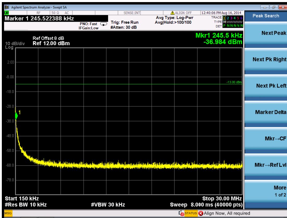
(Plot 5.5.2 A2: Channel 4132: 826.40 MHz @ WCDMA Band V)
