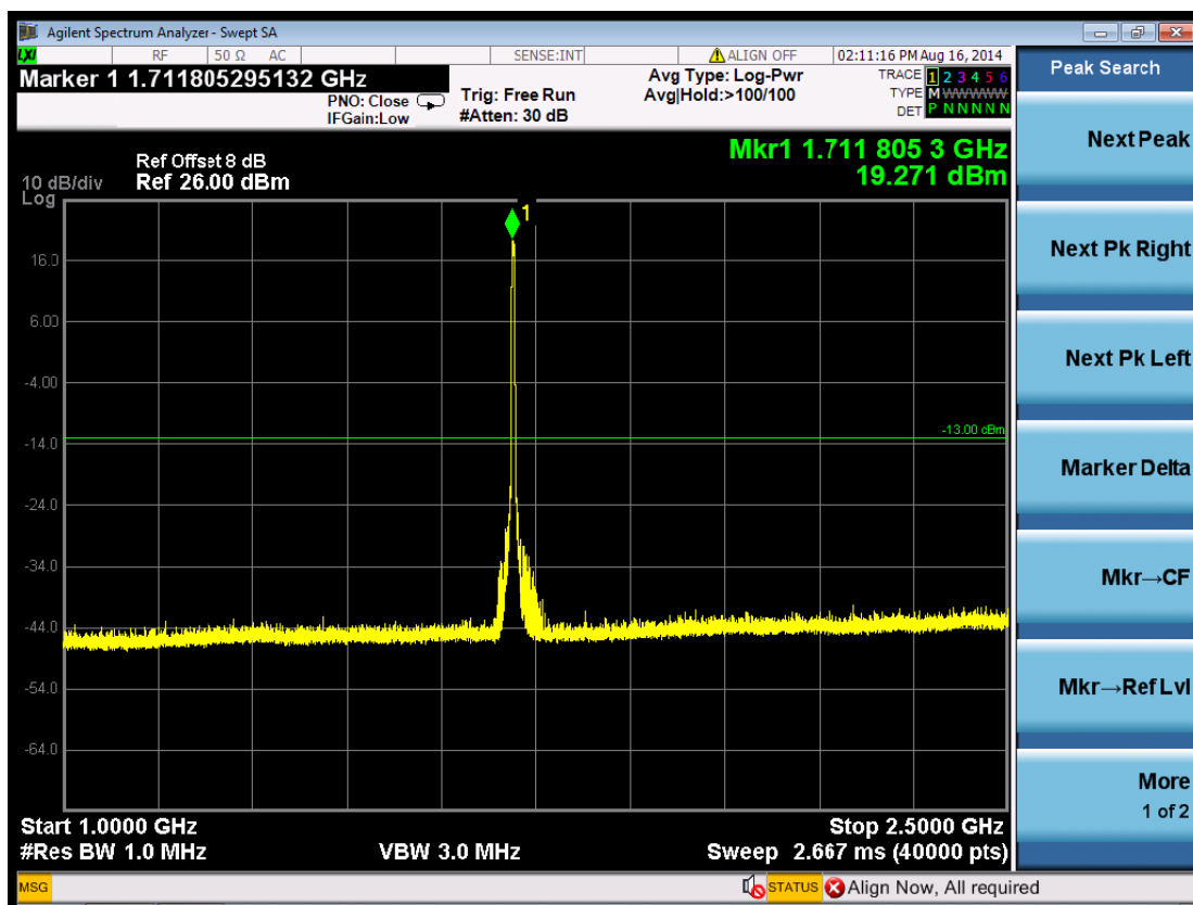
(Plot 5.5.3 A4: Channel 1312: 1712.4MHz @ Traffic WCDMA Band IV)
