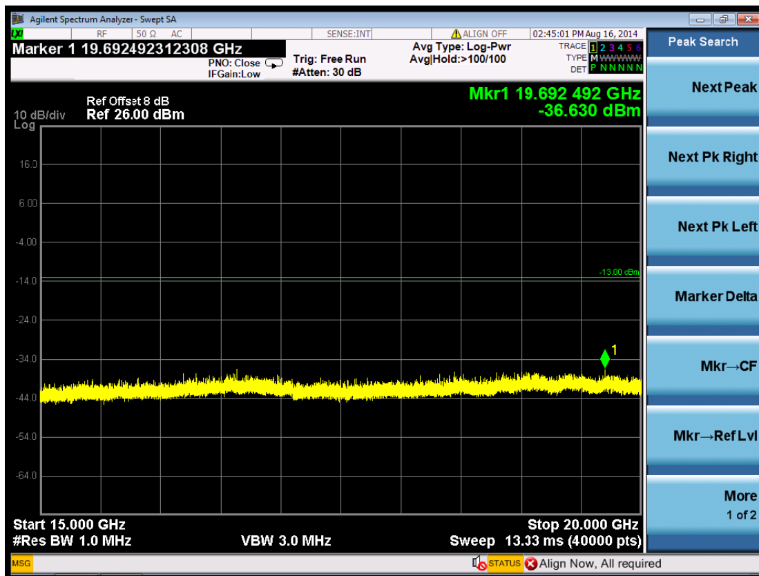
(Plot 5.5.1 B8: Channel 9400: 1880.0MHz @ Traffic WCDMA Band II)
