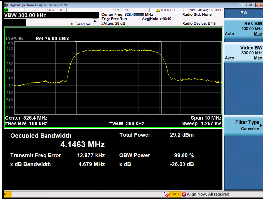
(Plot 5.3.3 A: Channel 4132:826.4MHz @ WCDMA Band V)
