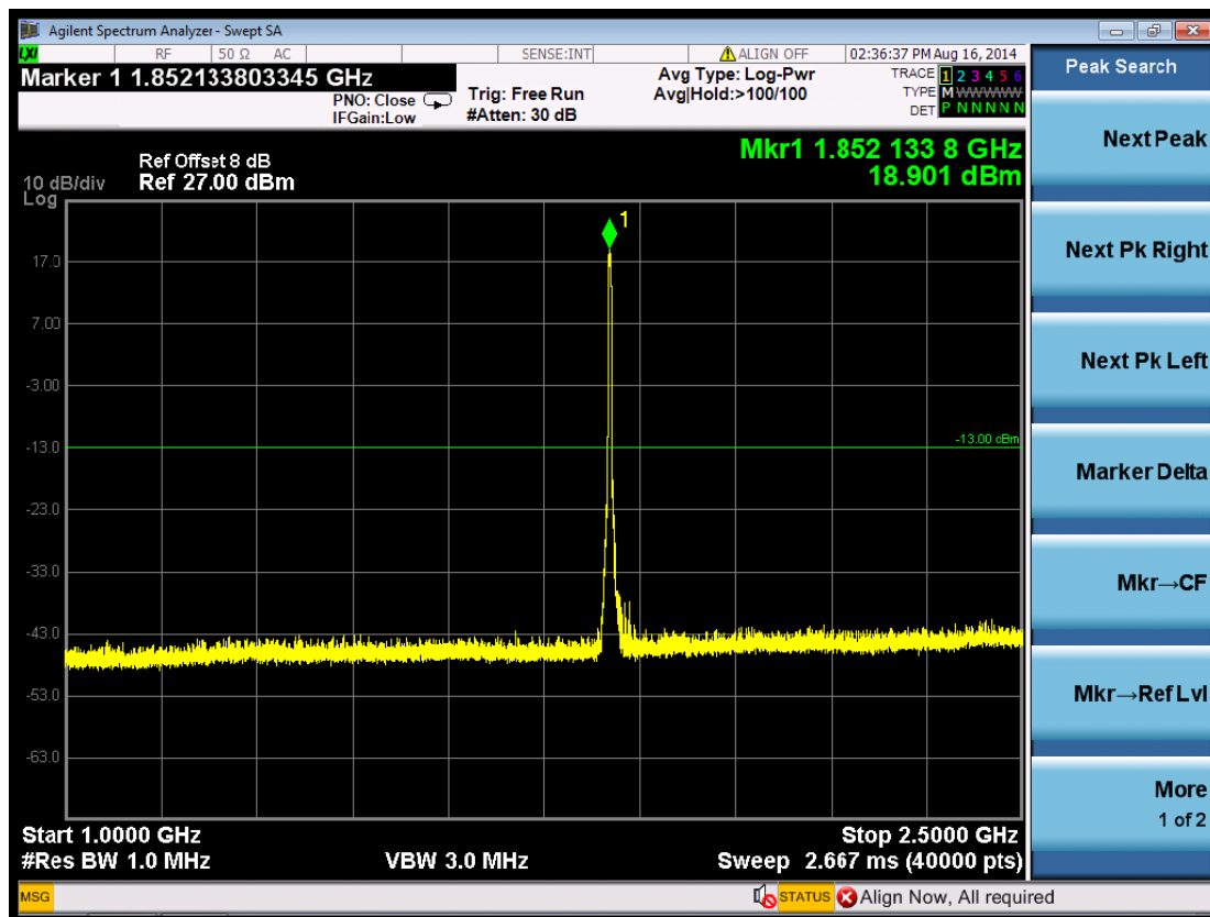
(Plot 5.5.1 A4: Channel 9262: 1852.4MHz @ Traffic WCDMA Band II)
