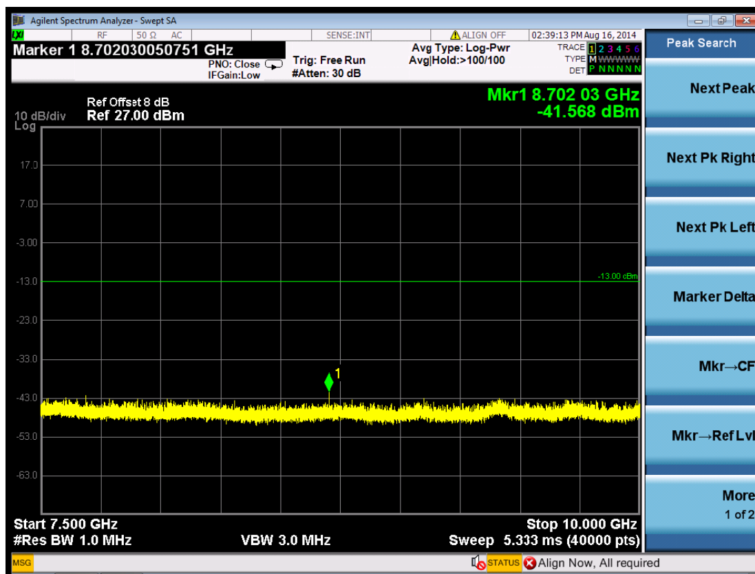
(Plot 5.5.1 A6: Channel 9262: 1852.4MHz @ Traffic WCDMA Band II)
