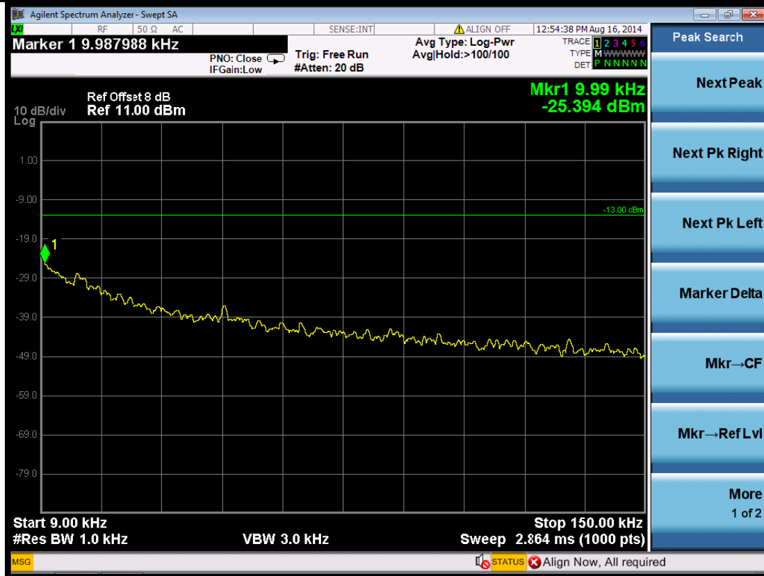
(Plot 5.5.2 A1: Channel 4132: 826.40 MHz @ WCDMA Band V)
