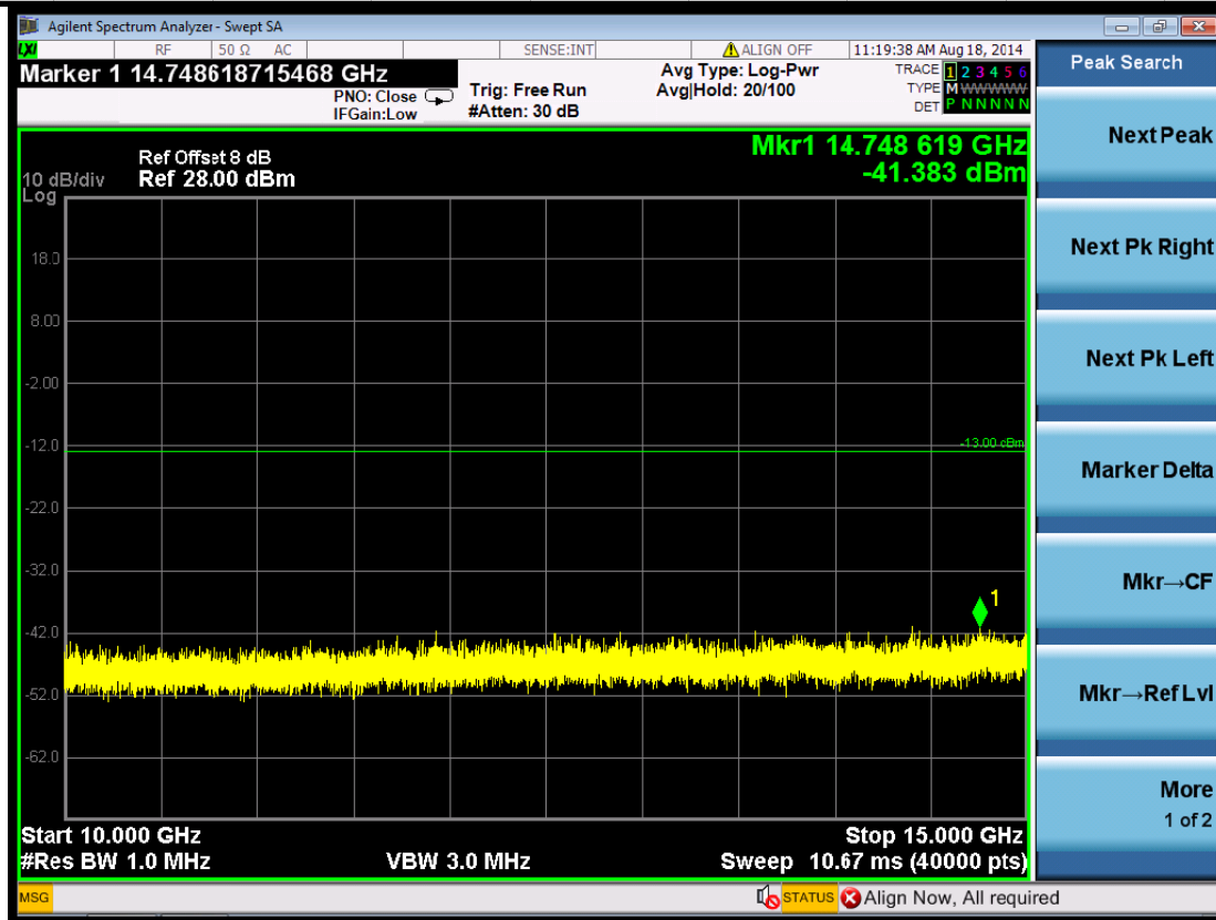
(Plot 5.5.1 C7: Channel 9538: 1907.6MHz @ Traffic WCDMA Band II)
