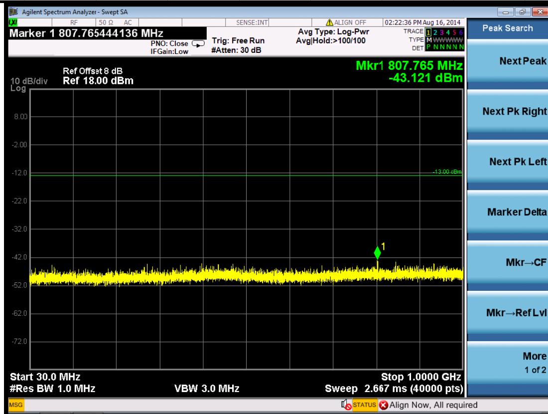
(Plot 5.5.3 C3: Channel 1513: 1752.6MHz @ Traffic WCDMA Band IV)
