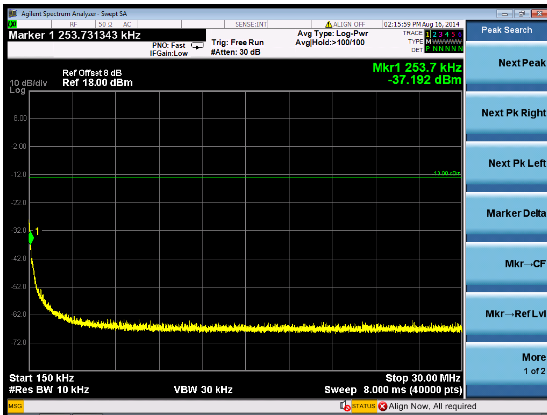
(Plot 5.5.3 B2: Channel 1413: 1732.6MHz @ Traffic WCDMA Band IV)
