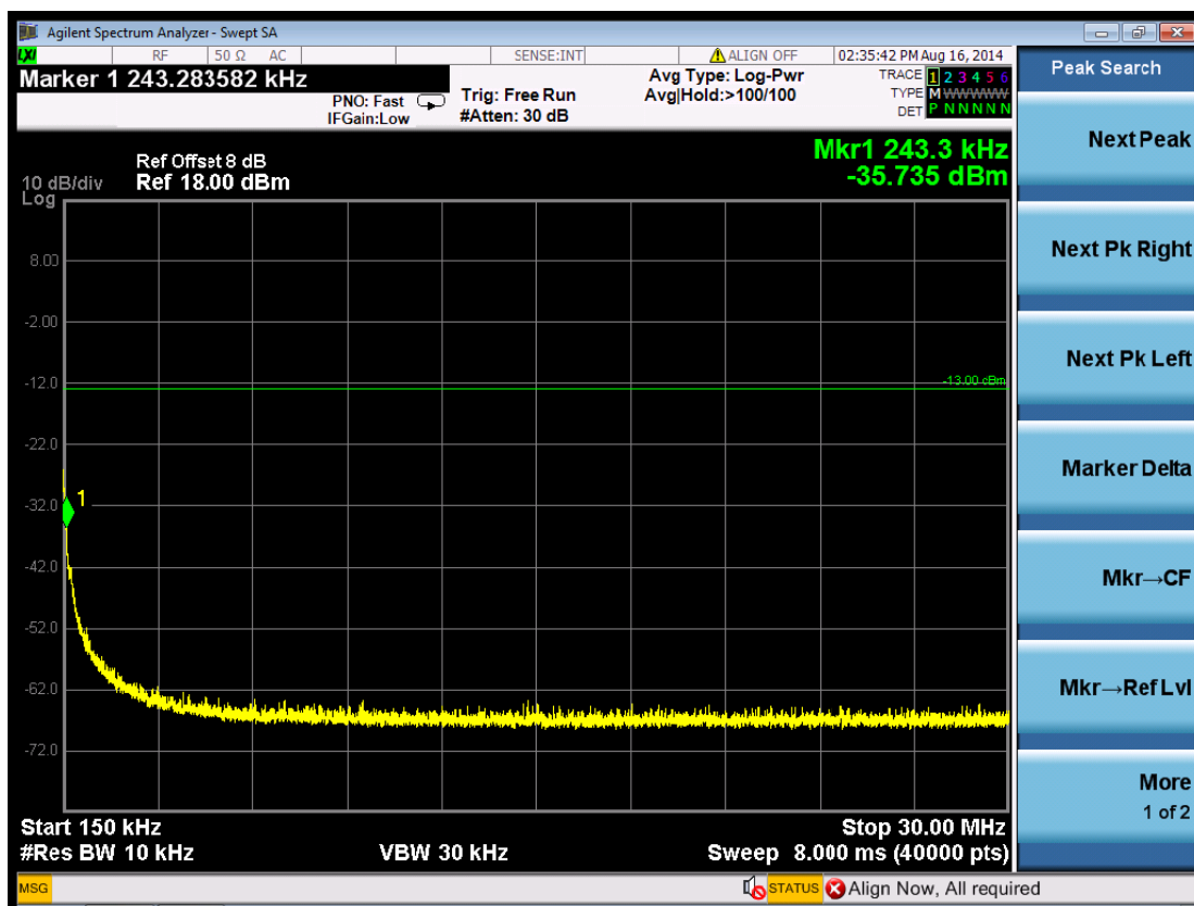
(Plot 5.5.1 A2: Channel 9262: 1852.4MHz @ Traffic WCDMA Band II)
