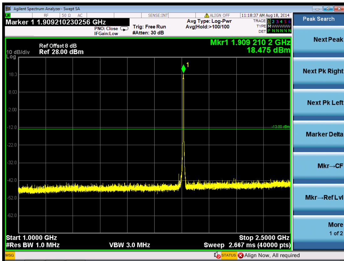
(Plot 5.5.1 C4: Channel 9538: 1907.6MHz @ Traffic WCDMA Band II)
