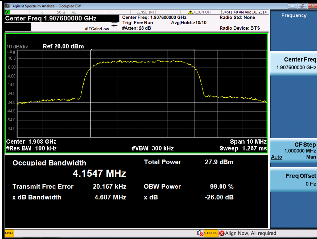
(Plot 5.3.1 C: Channel 9538: 1907.6MHz WCDMA Band II)
