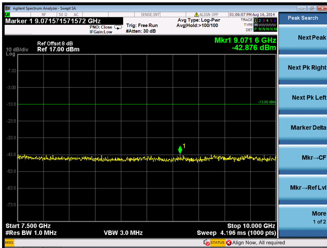
(Plot 5.5.2 B6: Channel 4183: 836.60 MHz @ WCDMA Band V)
