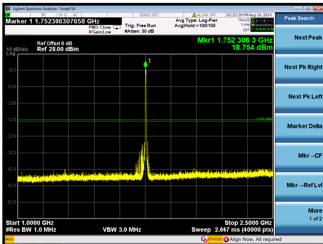
(Plot 5.5.3 C4: Channel 1513: 1752.6MHz @ Traffic WCDMA Band IV)
