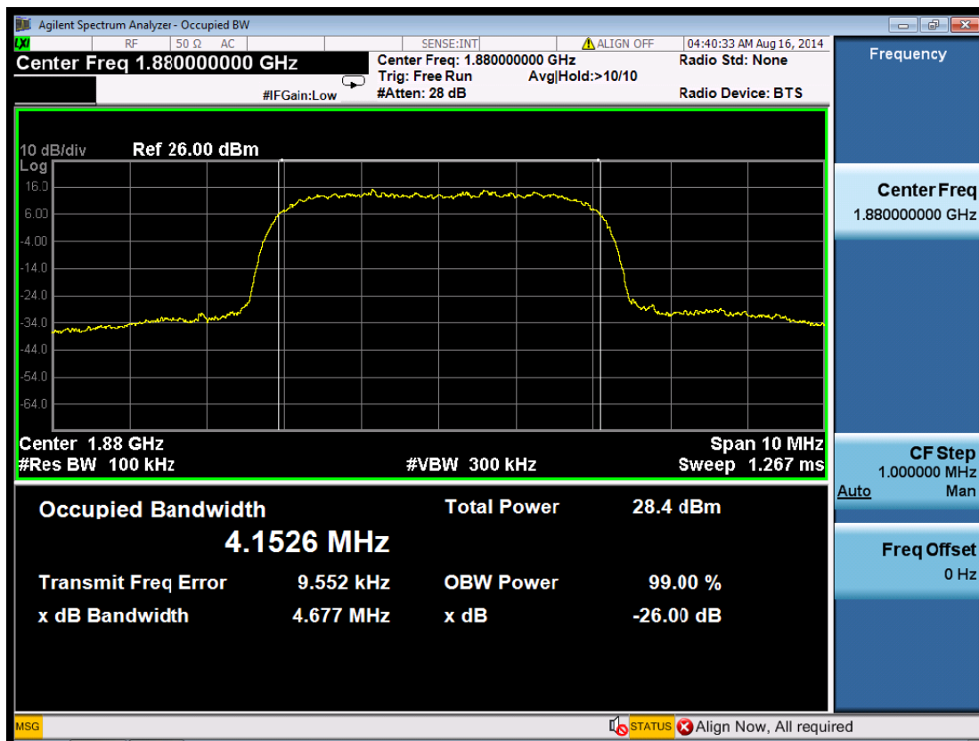
(Plot 5.3.1 B: Channel 9400: 1880.0MHz WCDMA Band II)
