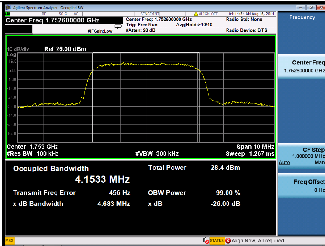
(Plot 5.3.2 C: Channel 1513: 1752.6MHz WCDMA Band IV)
