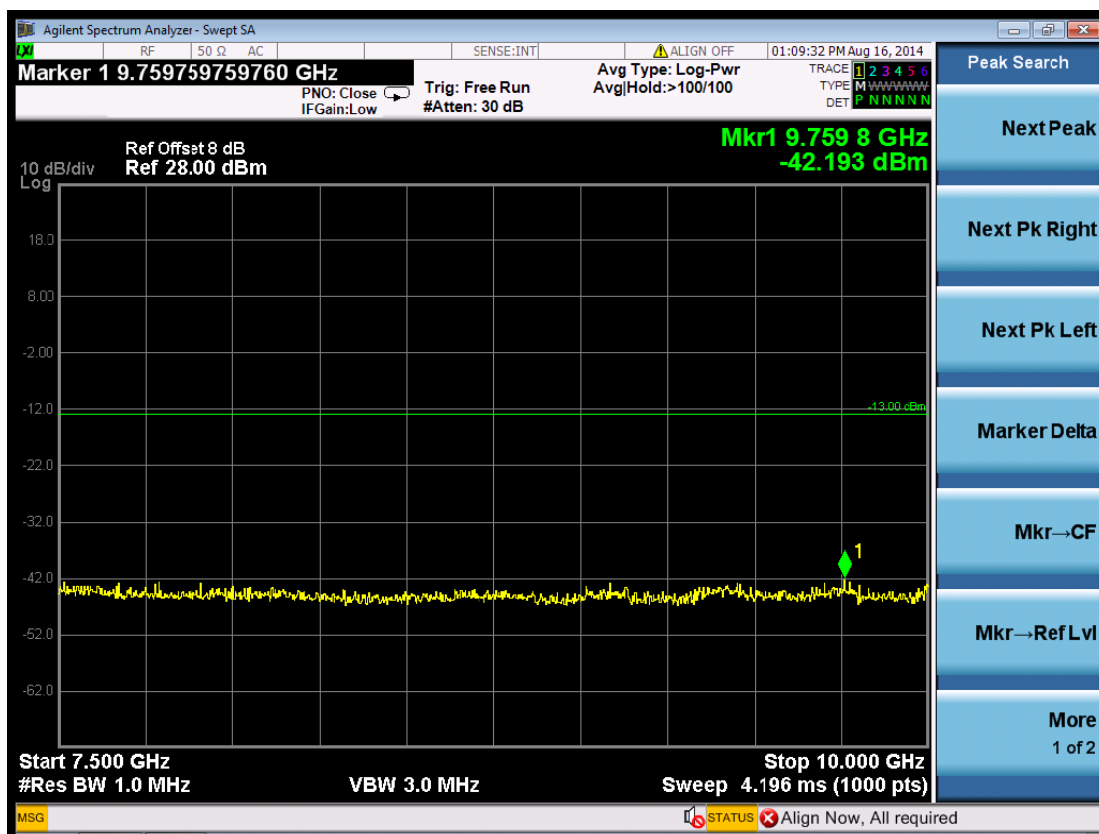
(Plot 5.5.2 C6: Channel 4233: 846.60 MHz @ WCDMA Band V)
