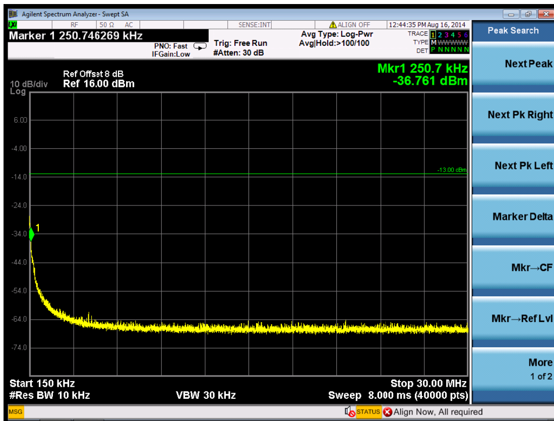
(Plot 5.5.2 B2: Channel 4183: 836.60 MHz @ WCDMA Band V)
