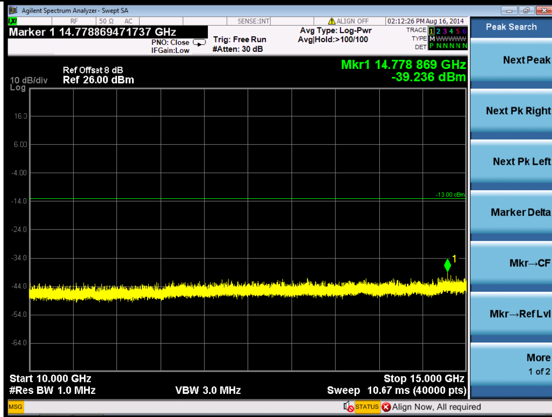
(Plot 5.5.3 A7: Channel 1312: 1712.4MHz @ Traffic WCDMA Band IV)
