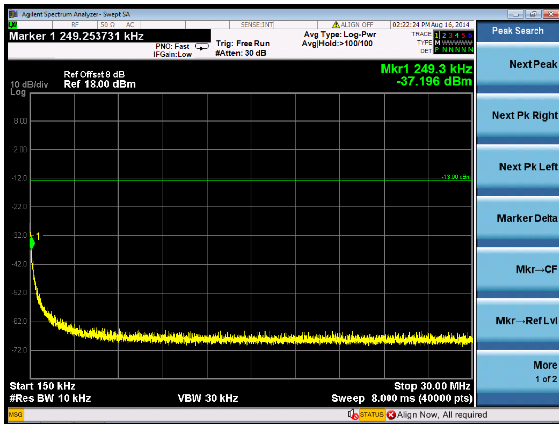
(Plot 5.5.3 C2: Channel 1513: 1752.6MHz @ Traffic WCDMA Band IV)
