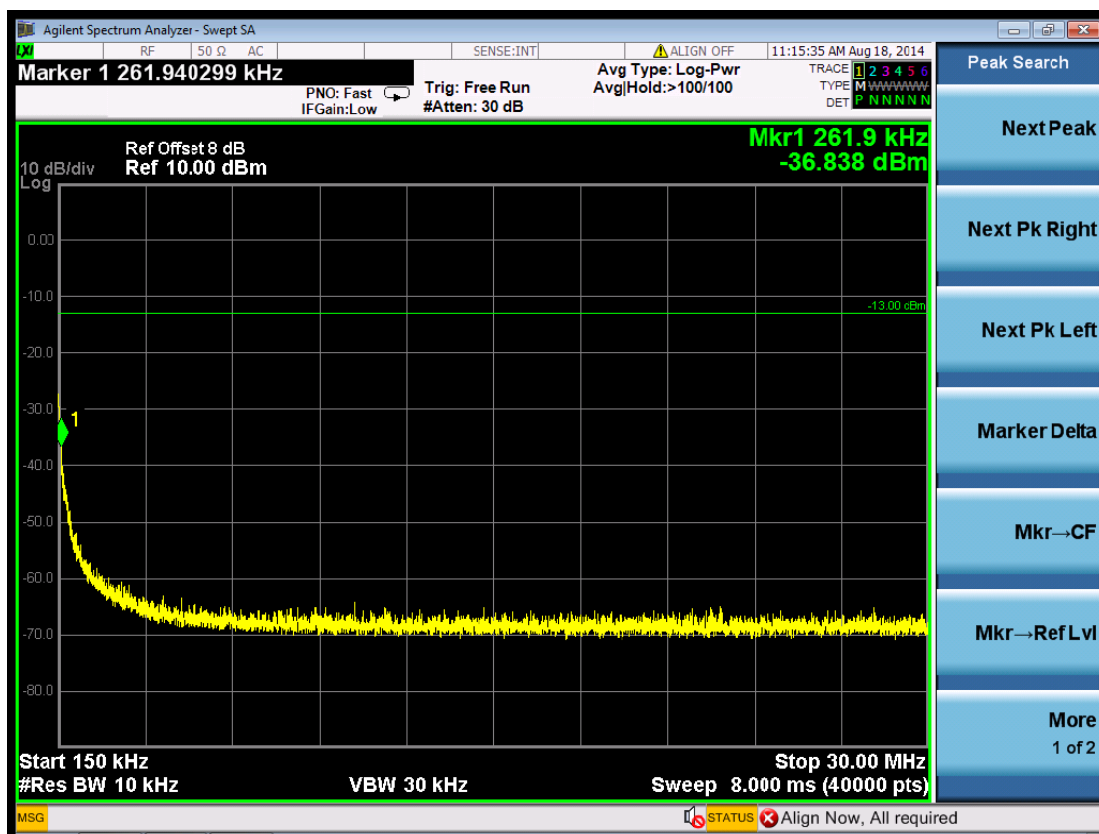
(Plot 5.5.1 C2: Channel 9538: 1907.6MHz @ Traffic WCDMA Band II)
