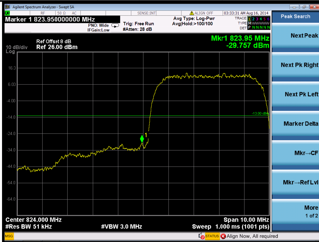
(Plot 5.4.3 A: Channel 4132: 826.4MHz @ WCDMA Band V)
