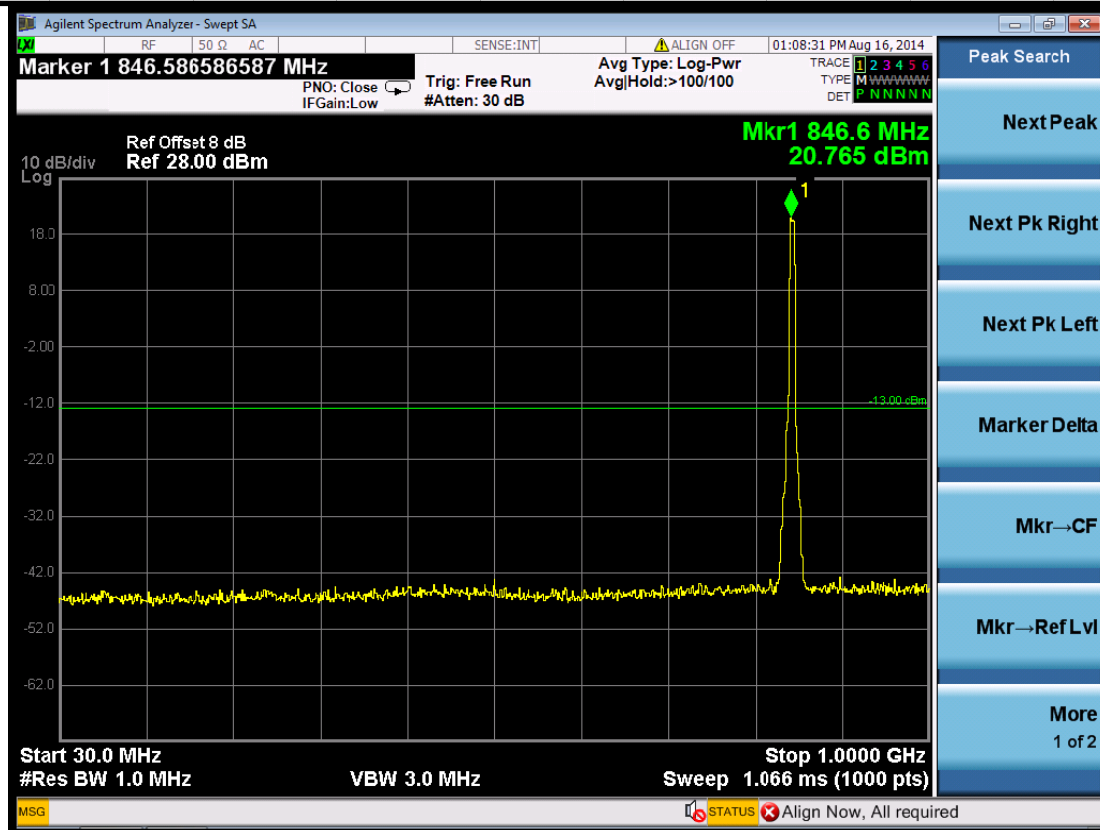
(Plot 5.5.2 C3: Channel 4233: 846.60 MHz @ WCDMA Band V)
