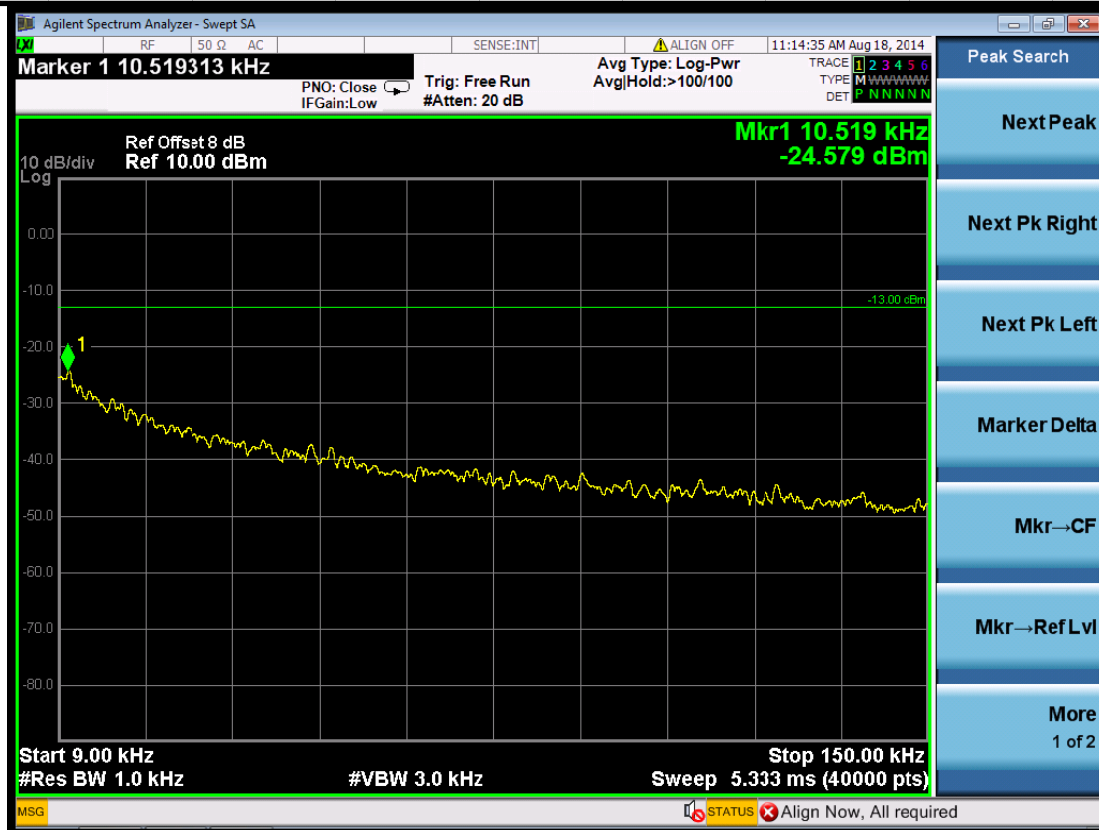
(Plot 5.5.1 C1: Channel 9538: 1907.6MHz @ Traffic WCDMA Band II)
