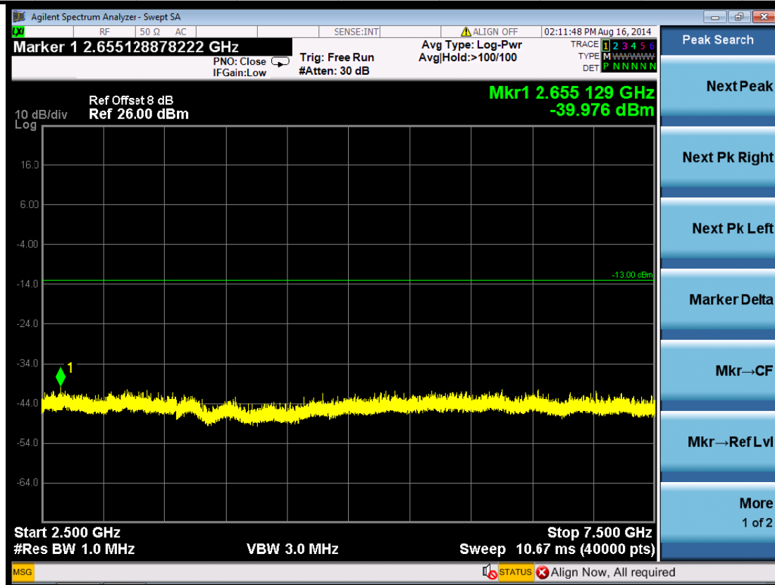
(Plot 5.5.9 A5: Channel 1312: 1712.4MHz @ Traffic WCDMA Band IV)
