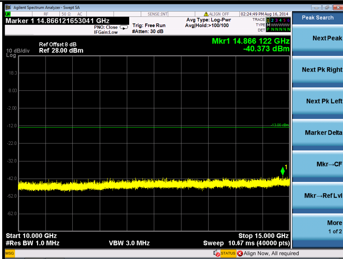
(Plot 5.5.3 C7: Channel 1513: 1752.6MHz @ Traffic WCDMA Band IV)
