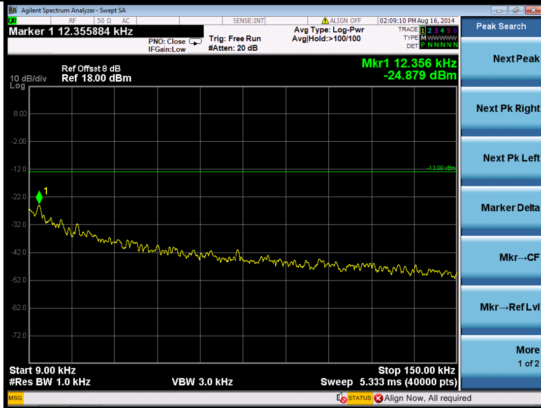
(Plot 5.5.3 A1: Channel 1312: 1712.4MHz @ Traffic WCDMA Band IV)
