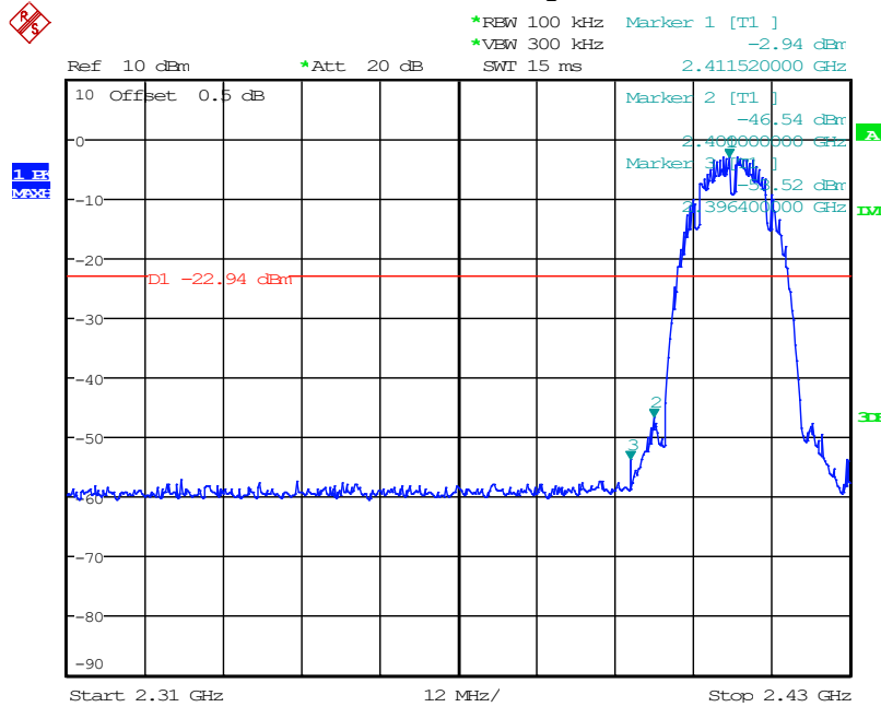
802.11b: Band Edge, Left Side
