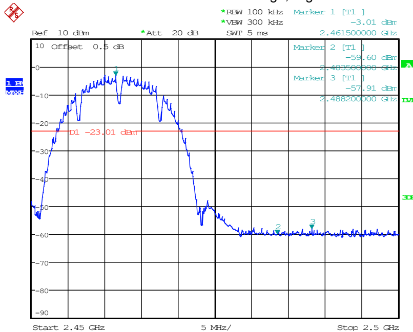
802.11b: Band Edge, Right Side
