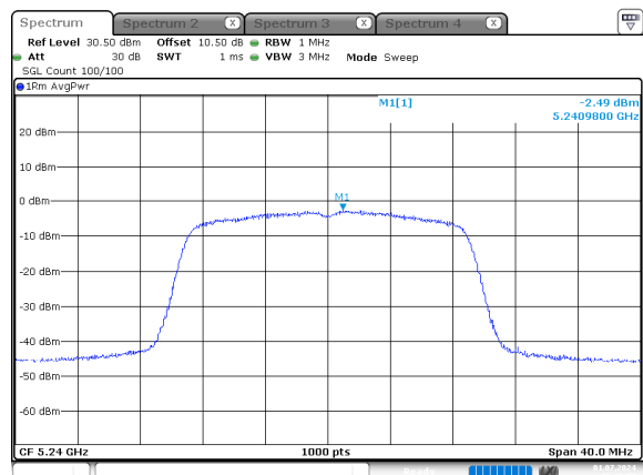
n20_5240MHz_Chain 1
