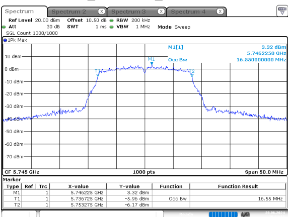
a_5745MHz_Chain 0
