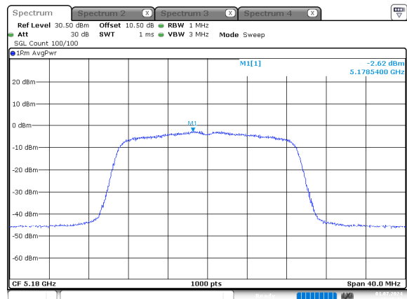
n20_5180MHz_Chain 1
