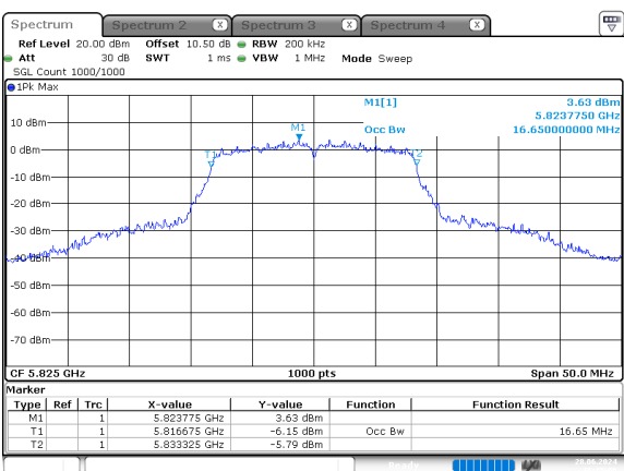
a_5825MHz_Chain 0
