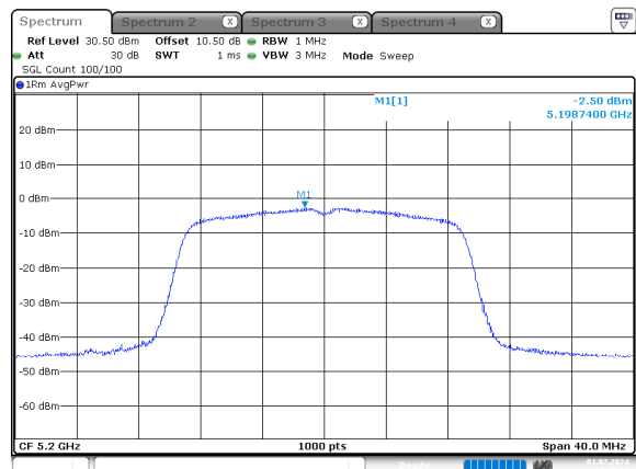
n20_5200MHz_Chain 1
