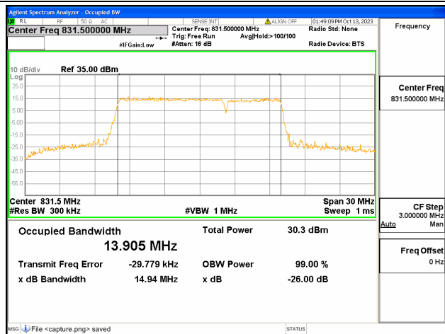
5B / 10+5MHz / 64QAM/ Low CH
