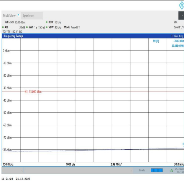
2-2-20MHz-15MHz-QPSK-QPSK-18700-18871-100RB#0-75R B#0-0.15~30MHz-PASS
