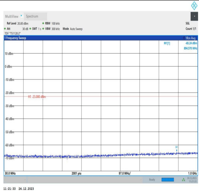
2-2-20MHz-15MHz-QPSK-QPSK-18700-18871-100RB#0-75R B#0-30~1000MHz-PASS
