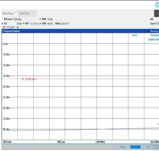
2-2-20MHz-15MHz-QPSK-QPSK-18826-18997-100RB#0-75R B#0-0.15~30MHz-PASS
