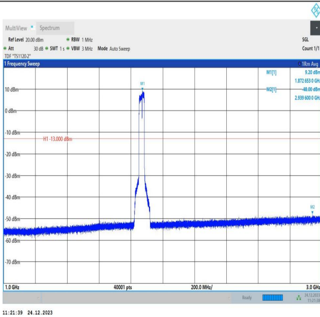
2-2-20MHz-15MHz-QPSK-QPSK-18700-18871-100RB#0-75R B#0-1000~3000MHz-PASS
