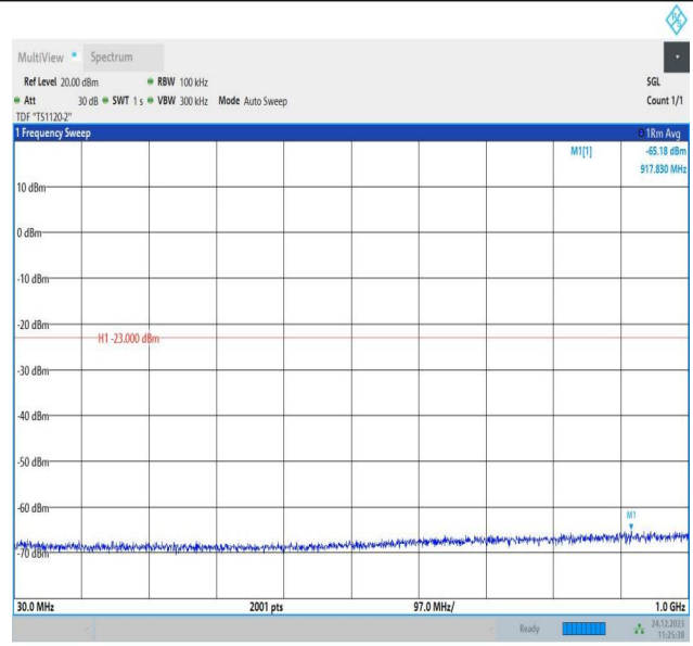
2-2-20MHz-15MHz-QPSK-QPSK-18826-18997-100RB#0-75R B#0-30~1000MHz-PASS
