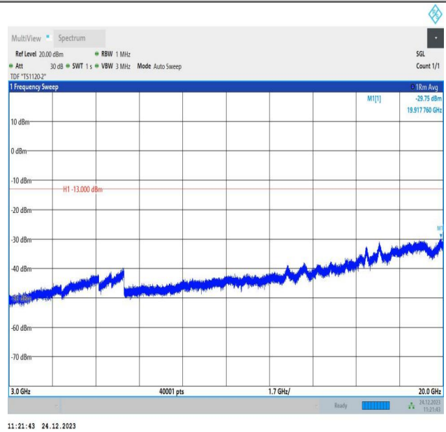
2-2-20MHz-15MHz-QPSK-QPSK-18700-18871-100RB#0-75R B#0-3000~20000MHz-PASS
