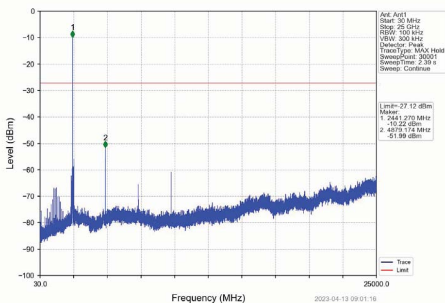
Pi/4DQPSK_2DH5_MCH_2441MHz_Ant1_NTNV
