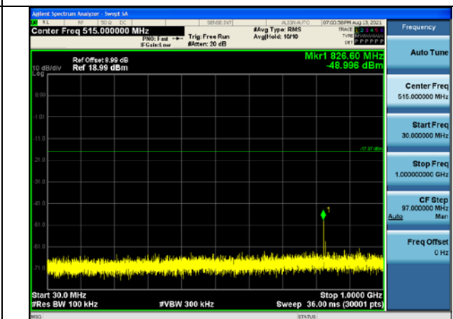
8DPSK on Channel 78
