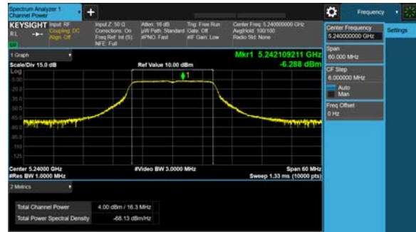
Antenna D
